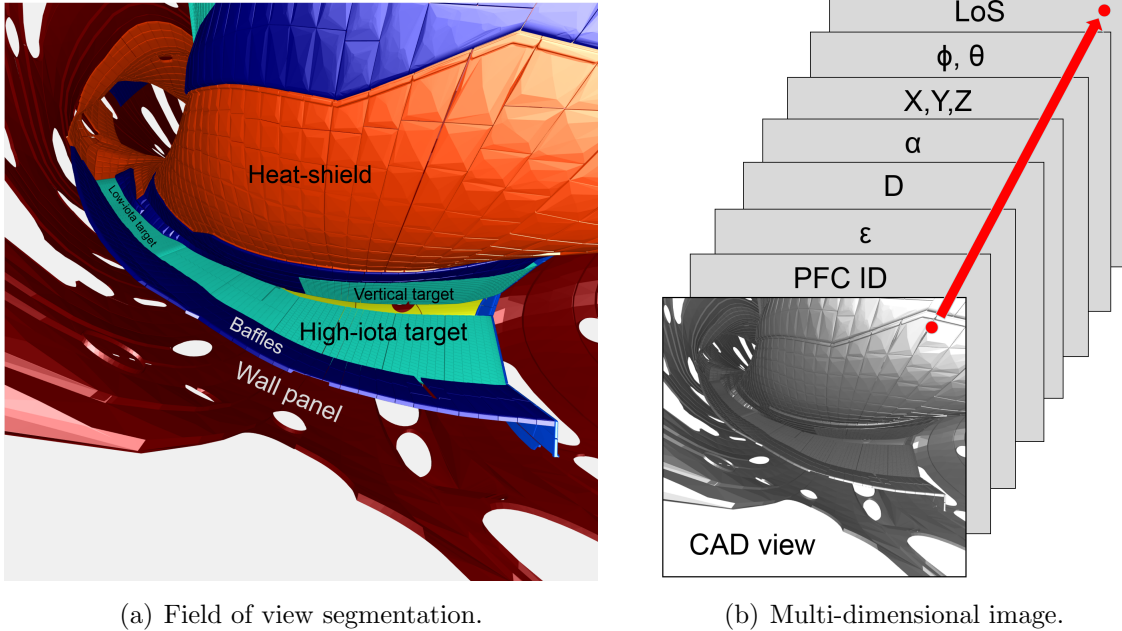
Figure 6. The scene model is a full segmentation of the field of view and it stores for each pixel the corresponding PFC, emissivity \epsilon , distance D to the target object, the angle \alpha of the line of sight respect the normal to the surface, the Cartesian world coordinates X,Y,Z , the toroidal and poloidal world coordinates \phi, \theta and the line of sight (LoS). The scene model is saved in a multi-dimensional image for each camera.
