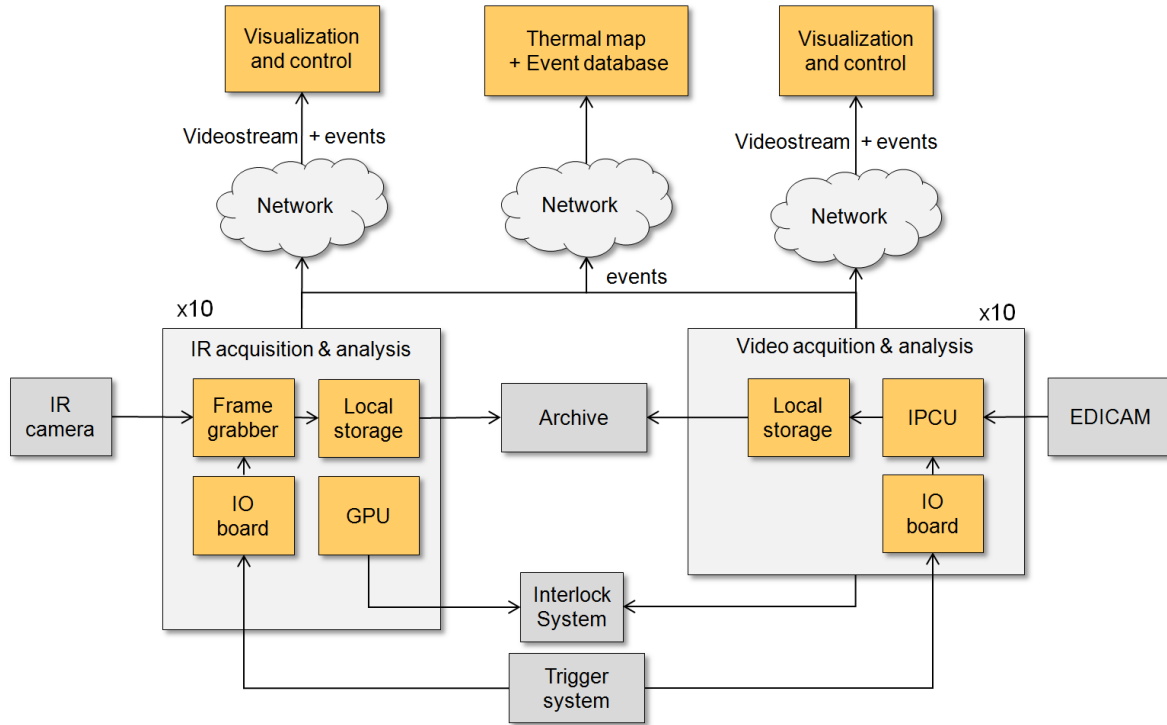
Figure 2. The system overview. 10 workstations acquire and analyze the images from the thermographic cameras and 10 workstations acquire and analyze images from 10 EDICAM video cameras. The acquisition workstations analyze the video streams and send alarms to the Interlock System. The video streams and the detected events are also sent to a centralized computer in the control room for visualization and control of the cameras.
