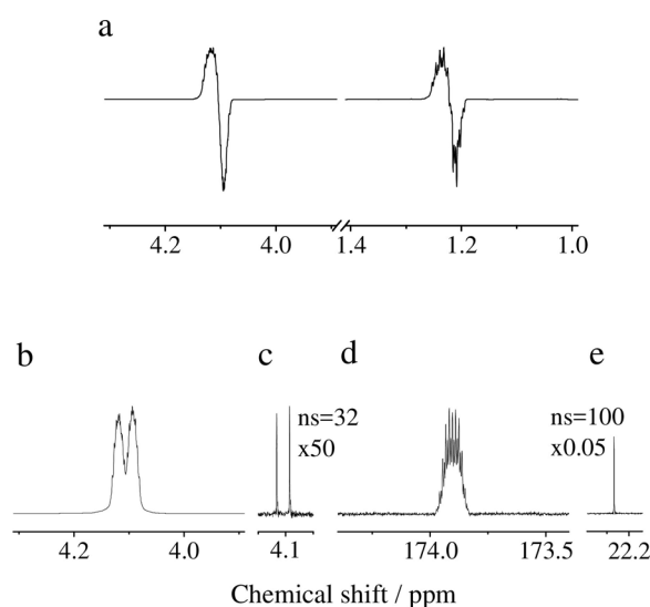
Figure 2. a) ^1\text{H} spectrum of hyperpolarized protons in ethyl acetate- d_6 detected with a 45^\circ pulse at B_0 = 7 \text{ T} . b) ^1\text{H} spectrum of the hyperpolarized ( P = 56.9\% , highest achieved polarization) methylene protons of ethyl acetate- d_6 in 0.6 mL solution after pulse sequence 1. c) Corresponding ^2\text{H} -decoupled ^1\text{H} spectrum after thermal equilibration. d) ^{13}\text{C} spectrum of the hyperpolarized ( P = 60.5\% , highest achieved polarization) carbonyl carbon of ethyl acetate- d_6 (at natural abundance) in 0.6 mL solution after utilizing sequence 2. e) ^1\text{H} -decoupled ^{13}\text{C} spectrum of toluene- \alpha - ^{13}\text{C} (enrichment >99\% ) used as internal reference after thermal equilibration. Note: The chemical shift scale is the same in both spectra for (d) and (e). Owing to hardware limitations, we could not decouple deuterium in the same experiment as the polarization transfer.
