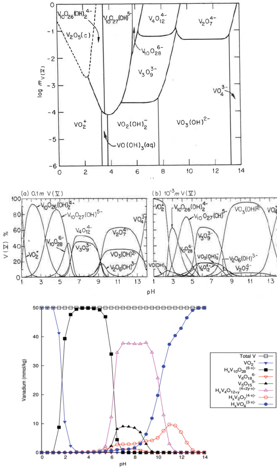
Fig. 1.2: Speciation diagrams for vanadate species in aqueous solutions. Top: based on potentiometry[1]. Middle: detailed speciation diagram for 0.1 M and 0.001 M V, based on potentiometry[1] Bottom: 50 mmol/kg vanadate solution, based on ^{51}\text{V} -NMR measurements.[3]
