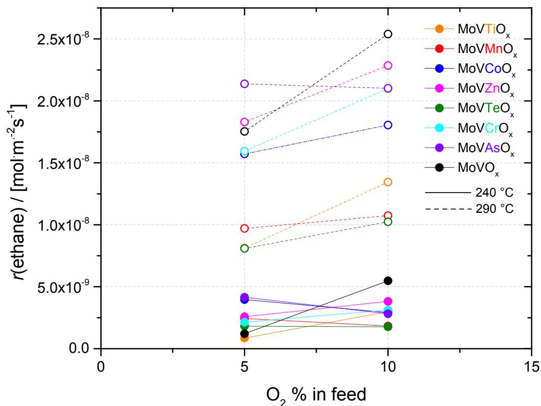
Fig. 6.11: Ethane conversion rate in \text{mol}(\text{ethane})/(\text{m}^2_{\text{cat}}\cdot\text{s}) depending on the \text{O}_2 content of the gas feed. Straight line indicates rates at 240 °C, dashed line at 290 °C.
