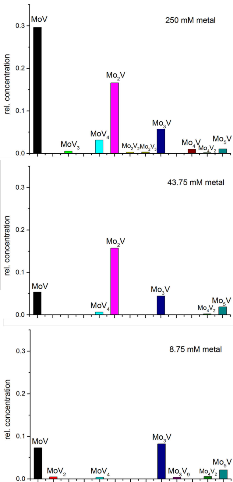
Fig. 5.8: Relative concentrations of mixed MoV species in mass spectra of mixed MoV solutions containing metavanadate as V source.
