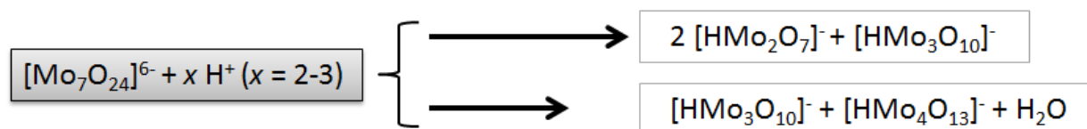
Fig. 3.19: Possible fragmentation processes of the condensed octamolybdates including a varying amount of protons. The length of the arrows symbolizes the probability of the process to take place based on the ion count in the measured spectra of a 0.35 M molybdate solution with pH 5.
