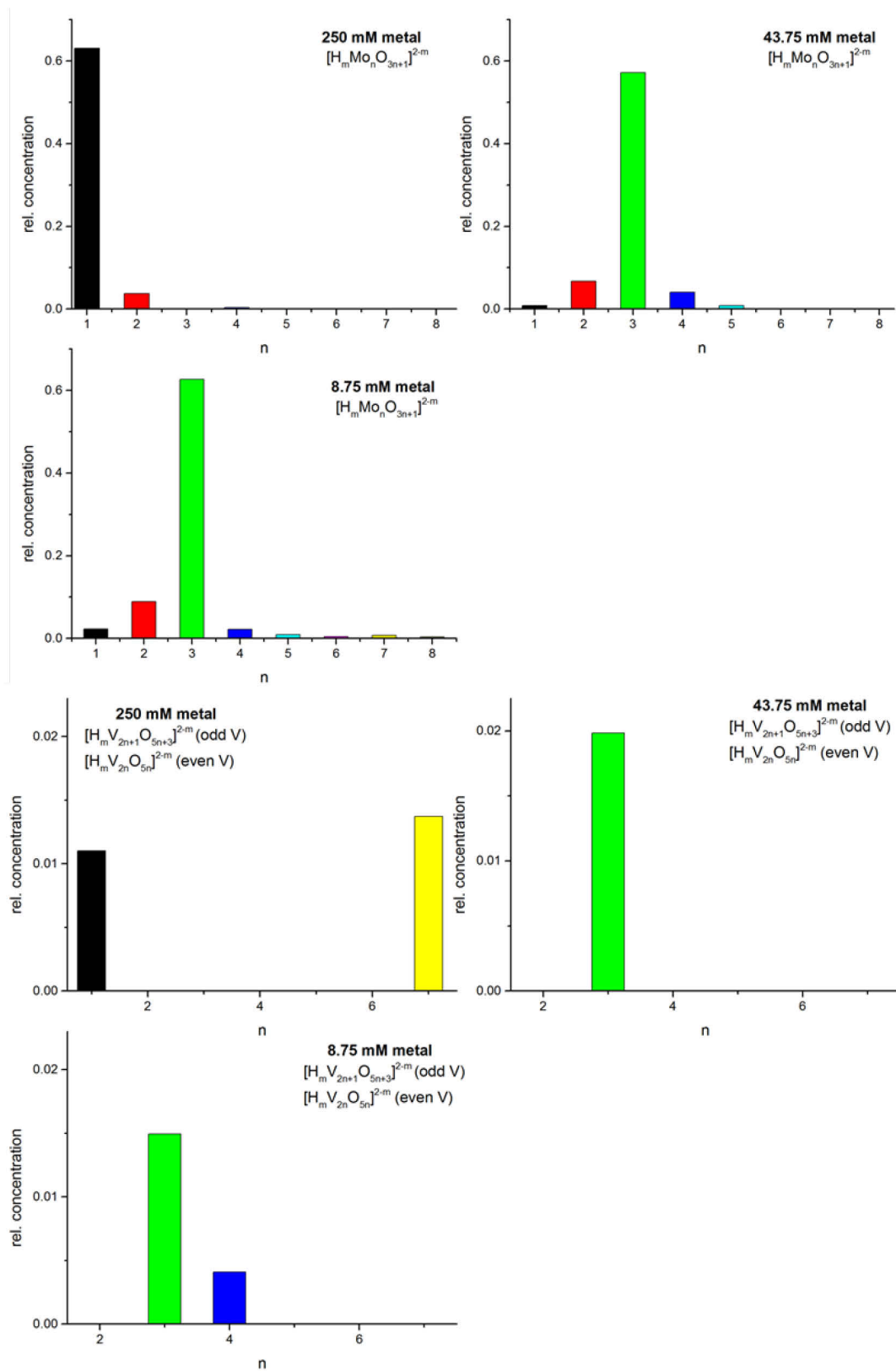
Fig. 5.7: Relative concentrations of isopolymolybdate and isopolyvanadate species in mass spectra of mixed MoV solutions containing metavanadate as V source.
