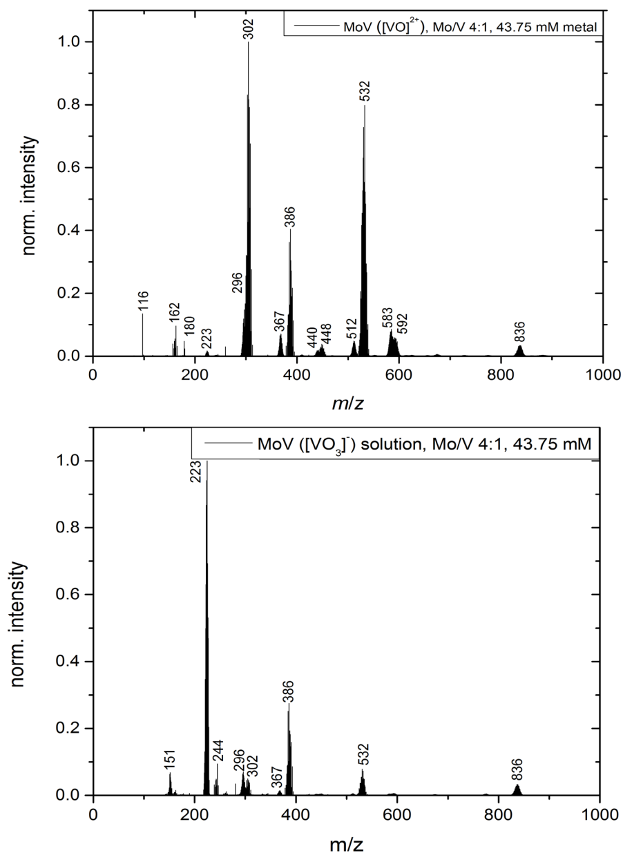
Fig. 5.3: Mass spectra of aqueous mixed MoV solutions with \text{VOSO}_4 (top) and \text{NH}_4\text{VO}_3 (bottom) as vanadium source.
