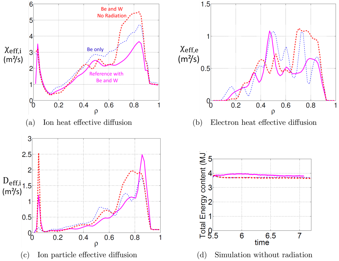
Figure 25: Ion and electron heat effective diffusion and ion particle effective diffusion at t=6.5\text{s} , and timetrace of the total energy content. Reference simulation with W and Be (magenta), simulation with Be only (blue) and simulation with Be and W without radiation (red)
