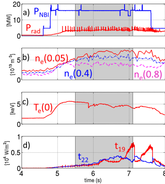
Figure 1: Experimental time traces of NBI and radiated power from bolometry (a), electron density at different position from HRTS (b), central electron temperature from ECE (c), and central (t19) and \rho=0.22 (t22) SXR lines of 82722 JET pulse
