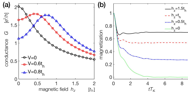
FIG. 9. (a) The differential conductance G (in unit of e^2/h ) is plotted against a magnetic field h_z for different bias potentials V . (b) Time evolution of the impurity magnetization ( \hat{\sigma}_{\text{imp}}^z(t) ) after the quench at finite bias V and magnetic field h_z . System size is L = 100 for each lead and we use j = 0.35 , V = 0.8t_h in (b).
