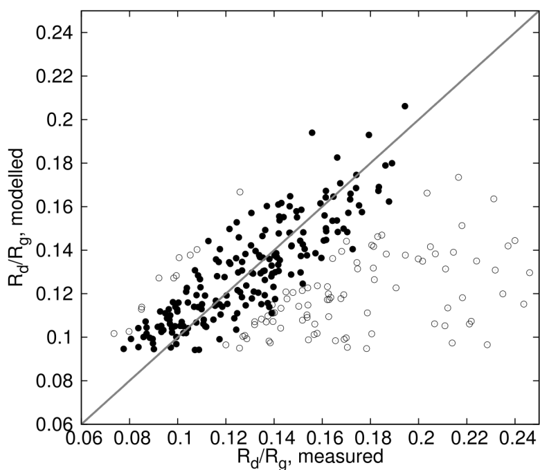
Figure 3. Diffuse fraction of global irradiance: modelled vs measured (SMEAR Estonia, 2016). Closed symbols: criterion of clear sky based on diffuse and global irradiance ( R_{d,meas}/R_{d,mod} > 0.8 , R_{g,meas}/R_{g,mod} > 0.9 ), closed symbols and open symbols: criterion of clear sky based on global irradiance ( R_{g,meas}/R_{g,mod} > 0.9 ).
