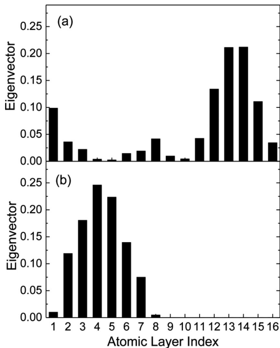
FIG. 5. (a) Eigenvector analysis of the calculated longitudinal-acoustic phonon mode at 35 meV vs the atomic-layer number in the bilayer of the Fe(8 ML)/Ag(8 ML) multilayer. The vibrational amplitude (vertical scale, arb. units) is found to decrease abruptly nearly to zero at the Fe/Ag interface (Fe layers number 1 and 8) as compared to the center Fe layer (Fe layer number 4). This demonstrates confinement of the 35-meV mode in the Fe layer. (b) Eigenvector analysis of the calculated phonon mode at 15 meV vs the atomic-layer number in the bilayer of the Fe(8 ML)/Ag(8 ML) multilayer. The vibrational amplitude (vertical scale, arb. units) demonstrates that the 15-meV phonon mode of Fe is coupled with the 15-meV vibrations of center Ag layers.
