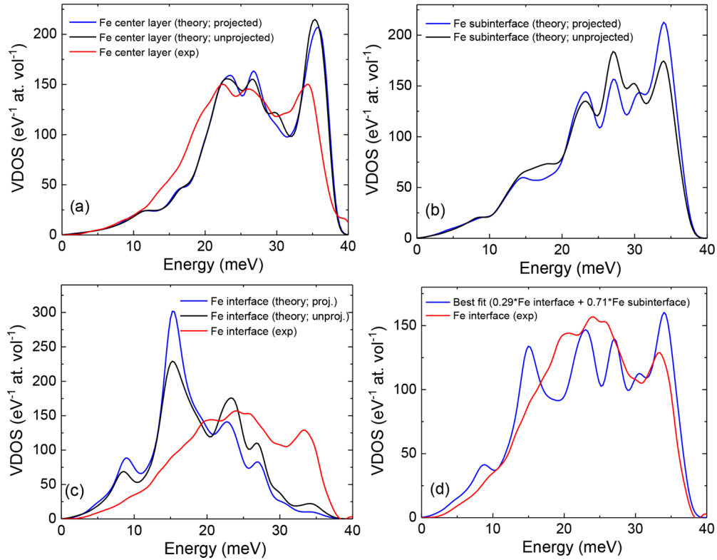
FIG. 9. A comparison among unprojected [from Fig. 4(c)] and direction-projected theoretical Fe-VDOS and experimental Fe-VDOS [from Fig. 3(a)] for Fe/Ag(001) multilayers. The areas below the theoretical VDOS curves are normalized according to the experimental VDOS. (a) The theoretical unprojected (black line) and projected (blue line) Fe-VDOS of Fe/Ag(001) at the center [Fe layer 4 in Fig. 4(c)] together with the experimental (red line) VDOS for the Fe center layer in Fe/Ag; (b) the unprojected (black line) and projected (blue line) theoretical Fe-VDOS of the Fe/Ag(001) subinterface [Fe layer 2 in Fig. 4(c)]. (c) The theoretical unprojected (black line) and projected (blue line) Fe-VDOS of Fe/Ag(001) at the interface [Fe layer 1 in Fig. 4(c)] together with the experimental (red line) VDOS for the Fe/Ag interface sample. (d) Best-fit of the experimental interface VDOS (red line) by the sum of the theoretical projected Fe interface and subinterface layer VDOS. The best fit (blue line) can be obtained by mixing 29% of the calculated interface VDOS and 71% of the calculated subinterface VDOS.
