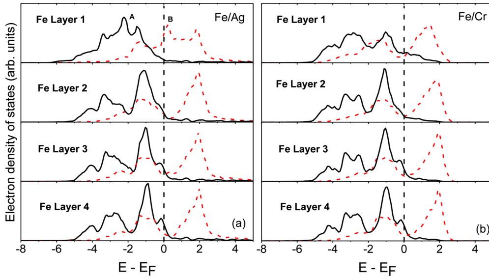
FIG. 8. DFT-calculated layer- and spin-resolved electronic density of states, D(E) , of the Fe layer in (a) Fe/Ag(001) multilayer and (b) Fe/Cr(001) multilayer. Fe layer 1 is located directly at the Fe/Ag or Fe/Cr interface, and Fe layer 4 is the center layer in the Fe film. Fe layer 2 (Fe layer 3) is the second (third) Fe layer from the interface. Majority spins: black lines; minority spins: red dotted lines. ( E_F = Fermi energy). A and B indicate peaks that exist only at the Fe/Ag interface.
