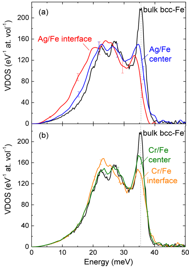
FIG. 3. Fe-projected vibrational density of states (VDOS), g(E) , obtained by ^{57}\text{Fe} NRIXS at room temperature for (a) Fe/Ag multilayers, and (b) Fe/Cr multilayers. All samples contain ultrathin ^{57}\text{Fe} probe layers either at the interface or in the center of the Fe layer. (a) Fe/Ag center layer (blue line) and interface layer (red line). (b) Fe/Cr center layer (green line) and interface layer (orange line). For comparison, also the VDOS of bulk bcc Fe at room temperature is shown (black lines), and the position of the LA peak near 36 meV is shown by the vertical dotted line. The energy resolution \Delta E is 0.9 meV for Fe/Ag and 2.3 meV for Fe/Cr. Representative error bars are shown in (a) and (b).
