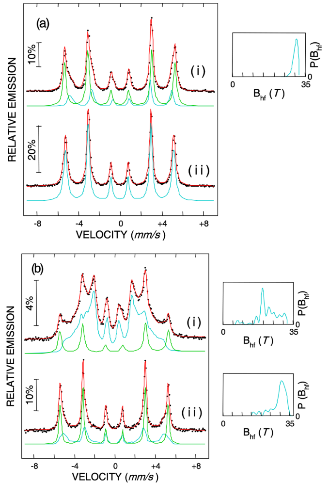
FIG. 2. ^{57}\text{Fe} conversion-electron Mössbauer spectra (CEMS) taken at 25 °C from (a) Fe/Ag, and (b) Fe/Cr multilayers: (i) “interface” and (ii) “center” samples. In (a)(ii), the data were fit with one sextet with sharp Lorentzian lines (blue line). In (a)(i), (b)(i), and (b)(ii), the data were least-squares fit with two spectral components: a sextet with sharp Lorentzian lines (green line), and a component (blue line) characterized by a distribution, P(B_{\text{hf}}) , of hyperfine magnetic fields B_{\text{hf}} (shown in each case on the right-hand side). Red lines: fits to the data. The fit parameters obtained are shown in Table SI (Ref. [39]).
