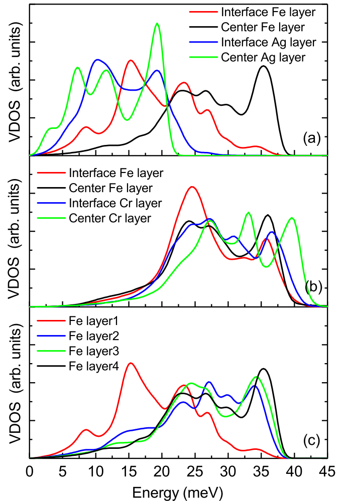
FIG. 4. DFT-calculated element-projected (partial) phonon density of states (VDOS) for (a) Fe/Ag(001) and (b) for Fe/Cr(001) multilayers. Only the VDOS of the interfacial and center layers of Fe and Ag or Cr are shown. (c) Calculated layer-resolved Fe-projected VDOS for the Fe/Ag(001) multilayer. Layer 1 (red: interface Fe layer; layer 2 (blue): second Fe layer from the interface; layer 3 (green): third Fe layer from the interface; layer 4 (black): center Fe layer. A Fermi-level smearing of 0.2 eV was used in the DFT calculations.
