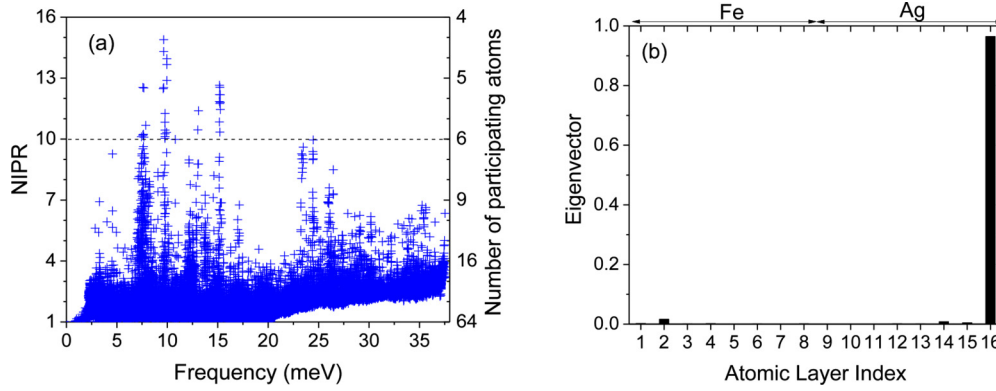
FIG. 6. (a) The calculated NIPR spectrum of the Fe/Ag(001) multilayer system. The horizontal dashed line represents the condition that N/\text{NIPR} = 6 . Phonons above the dashed line are considered as localized vibrations in a single layer; (b) The eigenvectors of atoms of the localized phonon mode at 9.6 meV with the highest NIPR value [14.9 in (a)]. This mode is localized at the Ag interface layer.
