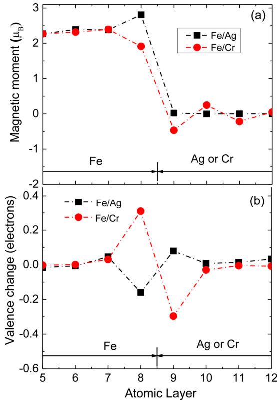
FIG. 7. DFT-calculated layer-resolved (a) magnetic moments and (b) d -valence charge change along the film normal direction of Fe/Ag(001) and Fe/Cr(001) multilayers, respectively. In (b), the positive value means electron accumulation (or valence increase), and the negative value means electron depletion (or valence decrease). Layer index 5: center Fe layer; layer index 8: interface Fe layer; layer index 9: interface Ag (or Cr) layer; and layer index 12: center Ag (or Cr) layer.
