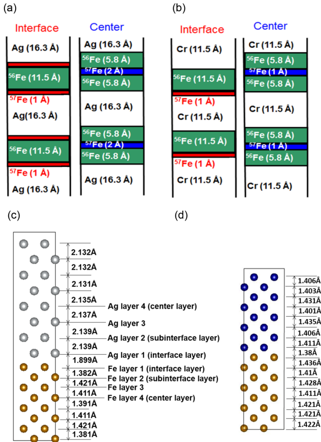
FIG. 1. Schematic experimental [(a) and (b)] and theoretical [(c) and (d)] structural models of [(a) and (c)] Fe/Ag and [(b) and (d)] Fe/Cr multilayers. In the drawing of the experimental samples, the ^{57}\text{Fe} layers are plotted in red when they are located at the interface of Ag or Cr, and in blue when they are placed at the center of a ^{56}\text{Fe} layer. In the theoretical plots, the numbers indicate out-of-plane atomic distances. Symbols: Ag atoms (silver), Fe atoms (gold), and Cr atoms (blue).
