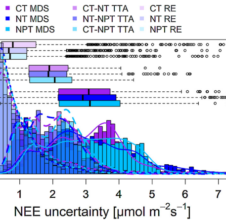
Fig. 7. Histograms of NEE flux uncertainties according to the random sampling error (most transparent colors and small dashed lines), the two-tower-approach (medium transparent colors and long dashed lines), and the standard deviation of the marginal distribution sampling (opaque colors and solid lines) for Spring 2014. Lines represent density fits to the respective histograms for better visibility where histograms are overlapping. CT MDS, NT MDS, and NPT MDS stand for the MDS uncertainty for the Control Tower-, Nitrogen added Tower-, and Nitrogen + Phosphorous added Tower; CT-NT TTA, NT-NPT TTA, and CT-NPT TTA for the two-tower-approach from the CT and NT tower, NT and NPT tower, and CT and NPT; and CT RE, NT RE, and NPT RE for the random sampling error of the respective towers.
