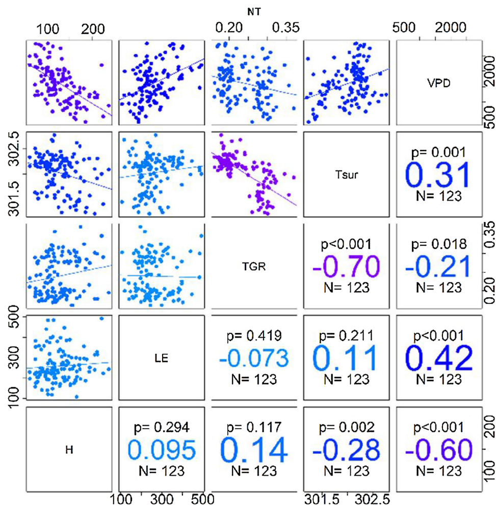
Fig. A11. Correlation matrix of H and LE of the NT with tree-grass-ratio (TGR), surface temperature (Tsur), and vapour pressure deficit (VPD) for the 13 days around the flight under high radiation condition. Upper left boxes display the scatterplots and a linear least square fit of the respective variables. Lower right boxes show the significance level (p), the spearman correlation coefficient (colored in the center) and the number of samples (N). The diagonal boxes show the respective variables. Colors indicate the strength of the correlation. Light blue for low correlation coefficients and bright pink for high correlation coefficients.
