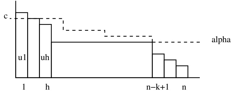
■ Figure 2 The allocation constructed in the proof of Theorem 15. The dashed line above agents 1 to n - k indicates the utility caps. The solid rectangles visualize the values of the bundles.
