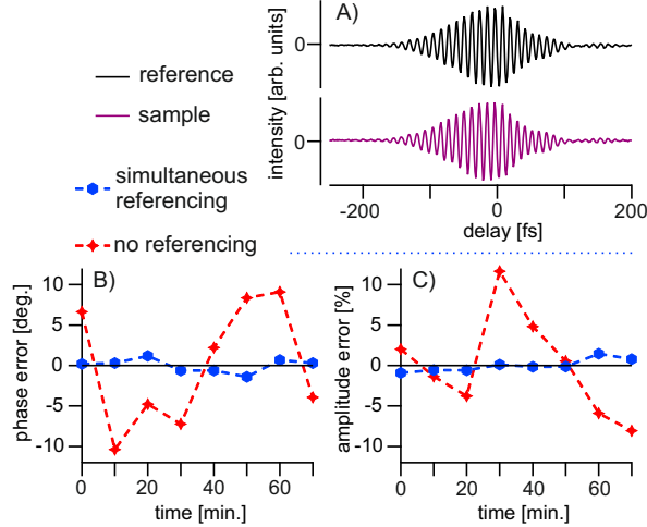
Figure 2: Measurement of the errors in phase and amplitude. Upper panel: A) interferometric raw data, lower panel: evolution of the B) phase and C) amplitude error with time from subsequent interferometric scans. Red crosses: phase/amplitude deviations from the respective mean values (without referencing); blue dots: phase/amplitude deviation from the reference (simultaneous referencing)
