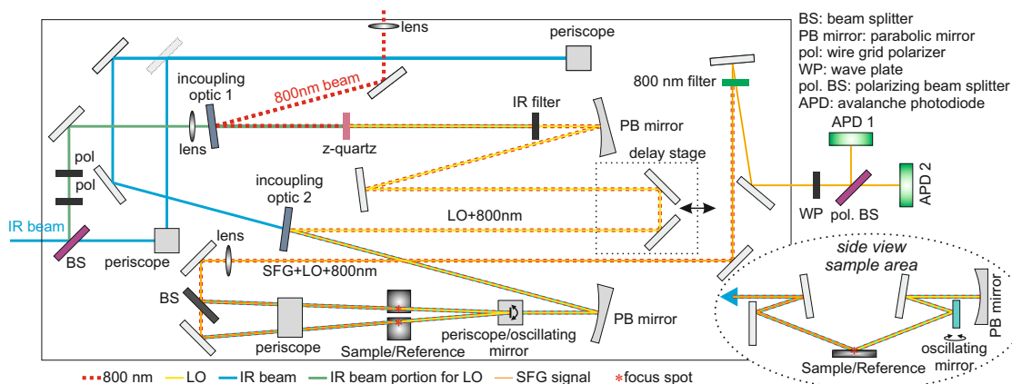
Figure 4: Diagram of the interferometer. The main portion shows the entire interferometer in the top view. The inset shows the sample area viewed from the side.
