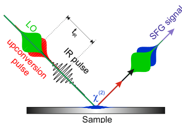
Figure 1: Schematic representation of time domain heterodyned SFG spectroscopy. The interaction of the infrared (black) and the upconversion pulse (red) with the sample generates an SFG signal (blue) which interferes with the local oscillator (green). Scanning the time delay t_{IR} modulates the relative phases between the SFG signal and LO which produces the desired interferogram.
