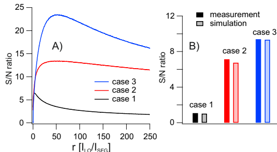
Figure 3: A) Simulation of the signal to noise ratio as function of the local oscillator intensity for a set of test parameters; B) Signal to noise ratios from experiment (solid bars) and simulation (transparent bars); case 1 simple heterodyned SFG; case 2 heterodyned SFG with balanced detection and taking the difference of the detector outputs; case 3 heterodyned SFG with balanced detection and taking the quotient of the difference and the sum of the detector outputs.
