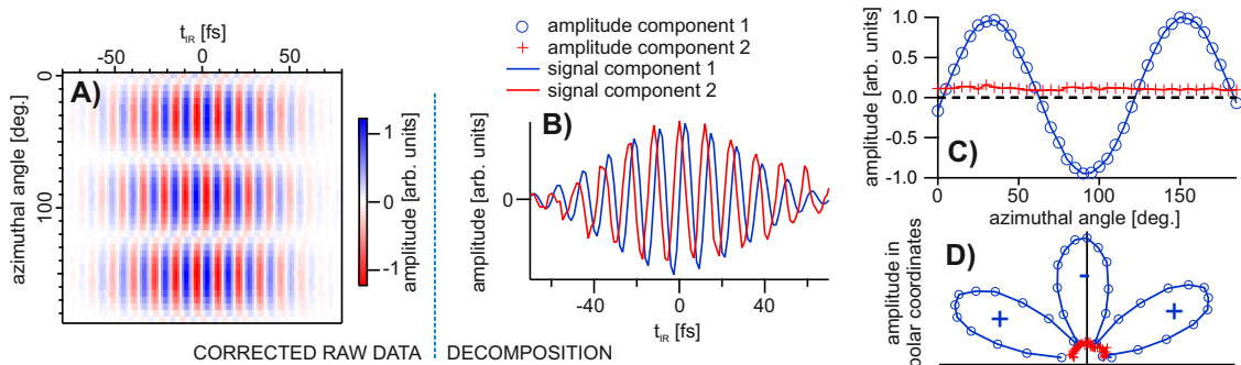
Figure 5: Referenced, phase resolved SFG measurement of the z-cut quartz surface. A) Interferometric raw data as function of the azimuthal angle (corrected for drifts in phase and amplitude); B) time domain signals from the two extracted components; C) azimuthal dependence of the amplitude for the two components; D) same as C) represented in polar coordinates.
