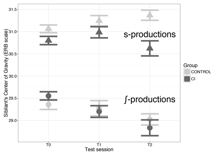
Figure 5.6: Means and standard errors for the sibilants' Center of Gravity (in ERB) for CI and control group across the three test sessions (T0, T1, T2). [ʃ] productions symbolized as circles, [s] productions as triangles.
