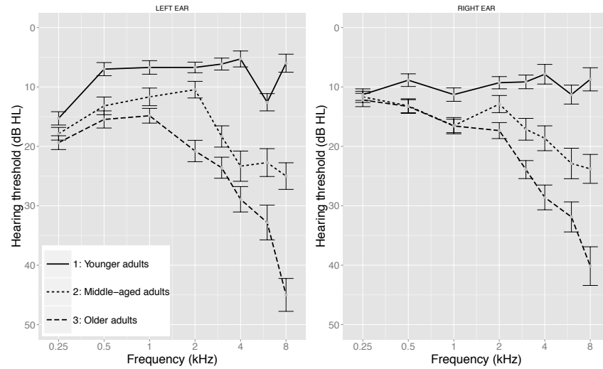
Figure 2.1: Mean audiometric pure-tone air conduction thresholds (for left and right ear) as a function of frequency for the younger, middle-aged and older adults. Error bars represent standard errors.
