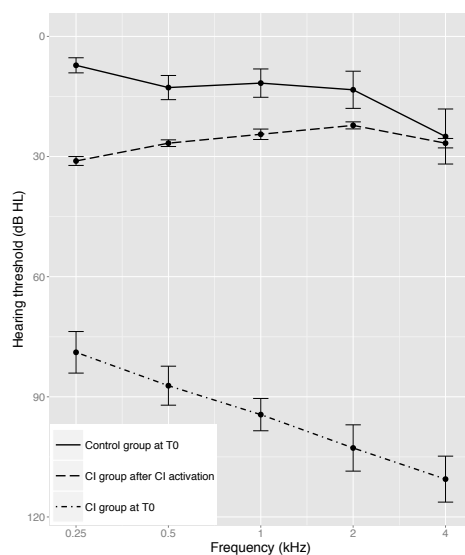
Figure 5.2: Mean audiometric pure-tone air conduction thresholds as a function of test frequency. Error bars represent standard errors. The figure shows performance at T0 for the CI and the control group (CI group: ear to be implanted, control group: best ear). Additionally, thresholds for the implanted ear are shown for the CI group at approximately eight weeks after activation of the cochlear implant.
