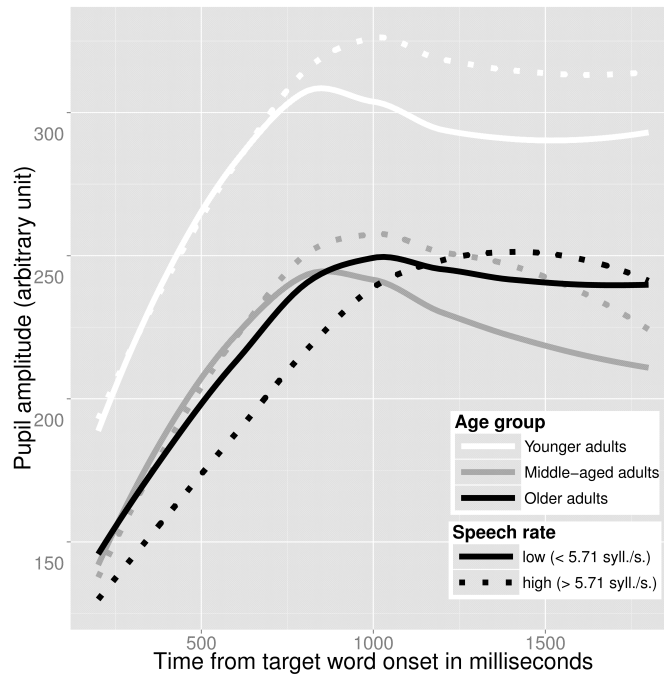
Figure 2.5: Task evoked pupillometry response per age group for low and high speech rate items (median split on speech rate). The window chosen for peak detection was from 500 ms to 1800 ms after word onset.
