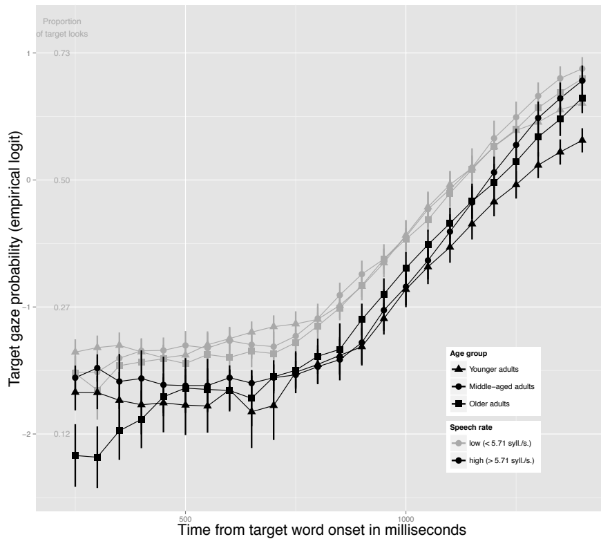
Figure 2.4: Target fixation probability over the analysis interval (200 ms – 1400 ms) for the three age groups for low and high speech rate items (median split on speech rate). Error bars represent standard errors.
