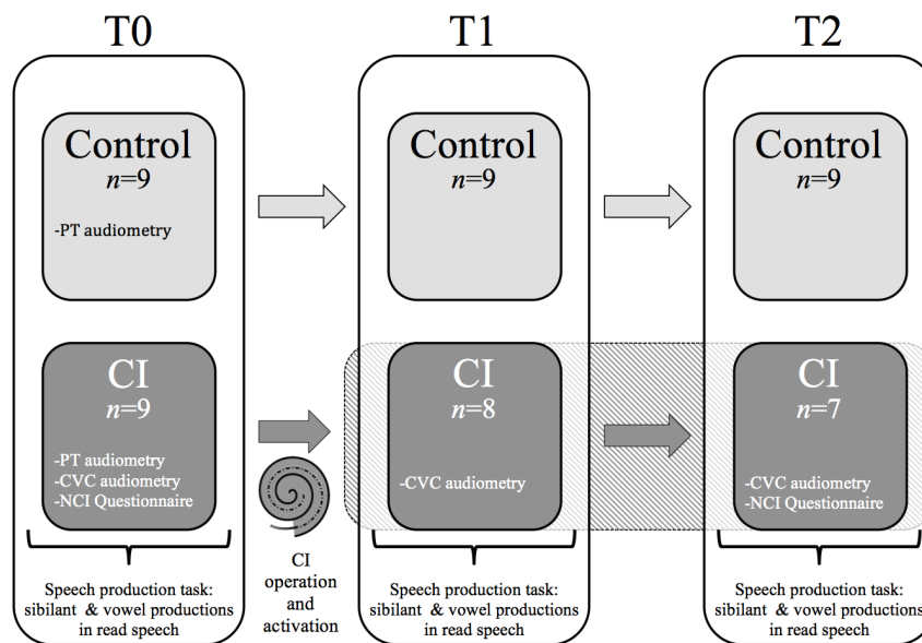
Figure 5.1: Schematic of the procedure.
