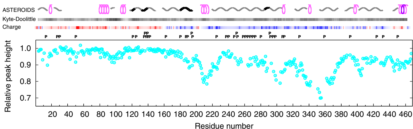
Figure 9. Relative decrease of peak height in HNC0 NMR spectra of 70 \mu\text{M} MAP2c upon the addition of 70 \mu\text{M} SR4-SR5-SH3 plectin fragment. Secondary structure motifs determined by the ASTERIODS analysis, hydrophaticity, and charge distribution are shown above the plot. The symbols used to describe the secondary structure motifs are explained in the legend to Fig. 4. The hydrophaticity index according to Kyte and Doolittle (85) is shown as darkness of the top bar above the plot (white and black correspond to values of -4.5 and +4.5 , respectively). The charge distribution is represented by the color in the bottom bar above the plot, corresponding to a relative electrostatic potential approximated by \sum_i CQ_i / (d_0 + d_1|n_i - n_j|) , where Q_i and n_i are charge and sequential number of the i th residue, C is a constant including the electric permittivity, and d_k are distance constants. The ratio d_1/d_0 was set to 2.0, and the colors were chosen so that red and blue correspond to the highest negative and positive potential, respectively, which makes the color code independent of C/d_0 (13). Letters P above the plot indicate positions of prolines.
