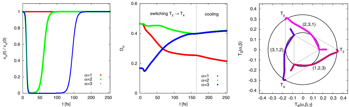
FIG. 2. Switching between T_8 > 0 states by suppression of hopping ( U = 1 eV, J = -0.25 eV, T = 33 K). The order parameter can be defined in terms of the linear combinations T_8(\alpha, \beta, \gamma) = (D_\alpha + D_\beta - 2D_\gamma)/\sqrt{3} and T_3(\alpha, \beta) = D_\alpha - D_\beta . The initial state is T_z = (I, I, M) , with order parameter T_8(1, 2, 3) > 0 , T_3(1, 2) = 0 , and the state after the switching is T_x = (M, I, I) . The left panel shows the time evolution of the hopping parameters for the three orbitals, the middle panel the time evolution of the double occupancy, and the right panel the (clockwise) rotation of the order parameter in the T_8 - T_3 plane.
