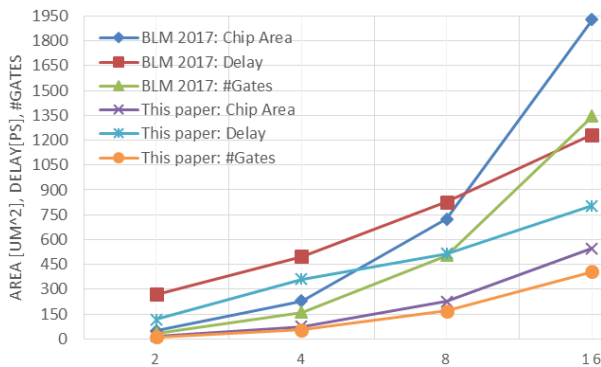
Figure 1: Area, delay, and gate count of 2\text{-sort}(B) for B \in \{2, 4, 8, 16\} ; we compare our solution to [2].
