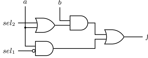
Figure 3: Selection circuit with inputs: a, b, sel_1, sel_2 and output f , used to implement \hat{\diamond}_M and out_M .
