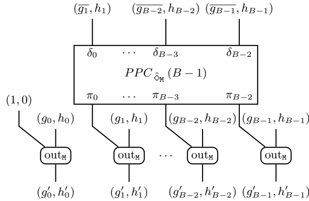
Figure 5: Construction of 2\text{-sort}(B) from out_M and PPC_{\hat{M}}(B-1) . PPC_{OP}(B-1) is specified in Figure 4, and we use the implementations of \hat{M} and out_M specified by Figure 3 and Table 6. For input Ns^{(0)} = (1, 0) , out_M reduces to an AND and an OR gate.
