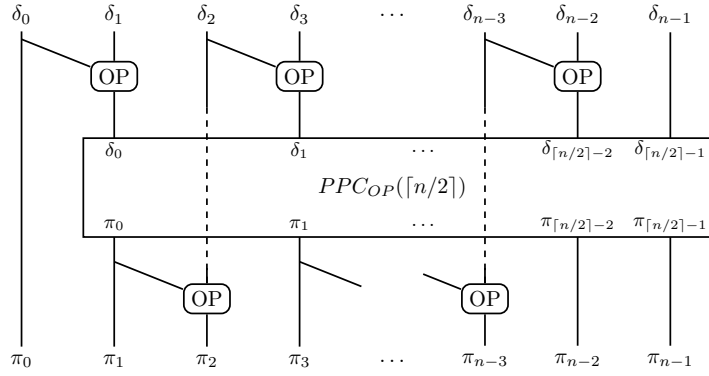
Figure 4: Recursive construction of PPC_{OP}(n) for odd n , computing \pi_i = \delta_0 OP \dots OP \delta_i . For even n the rightmost input ( \delta_{n-1} ) and output ( \pi_{n-1} ) are not present. Dashed lines are not connected to PPC_{OP}(\lceil n/2 \rceil) .
