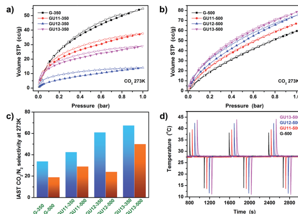
Fig. 4 CO 2 adsorption (solid symbols) and desorption (open symbols) isotherms at 273 K for materials prepared at (a) 350 °C and (b) 500 °C. (c) CO 2 /N 2 selectivity as calculated by the IAST method for a CO 2 : N 2 = 0.15 : 0.85 gas mixture at 273 K. (d) Thermal response measurements of CO 2 adsorption/desorption (1 bar, 298 K) of the materials prepared at 500 °C.
