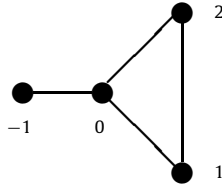
Fig. 4. Dynkin diagram of A_2^{++} with numbering of nodes.
