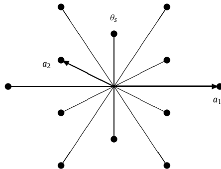
Fig. A.4. The root system of type G_2 with highest short root indicated.
