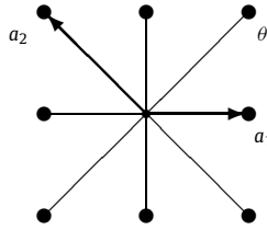
Fig. 5. The root system of type C_2 , with simple roots labeled and indicated by arrows. The lattice they generate is a scaled version of the ring of Gaussian integers. There are both long and short roots, and the same system gives type B_2 .
