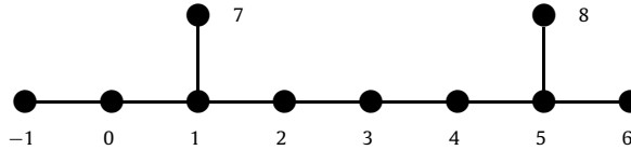
Fig. 16. Dynkin diagram of DE_{10} \equiv D_8^{++} with numbering of nodes.
