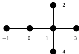
Fig. 9. Dynkin diagram of D_4^{++} with numbering of nodes.
