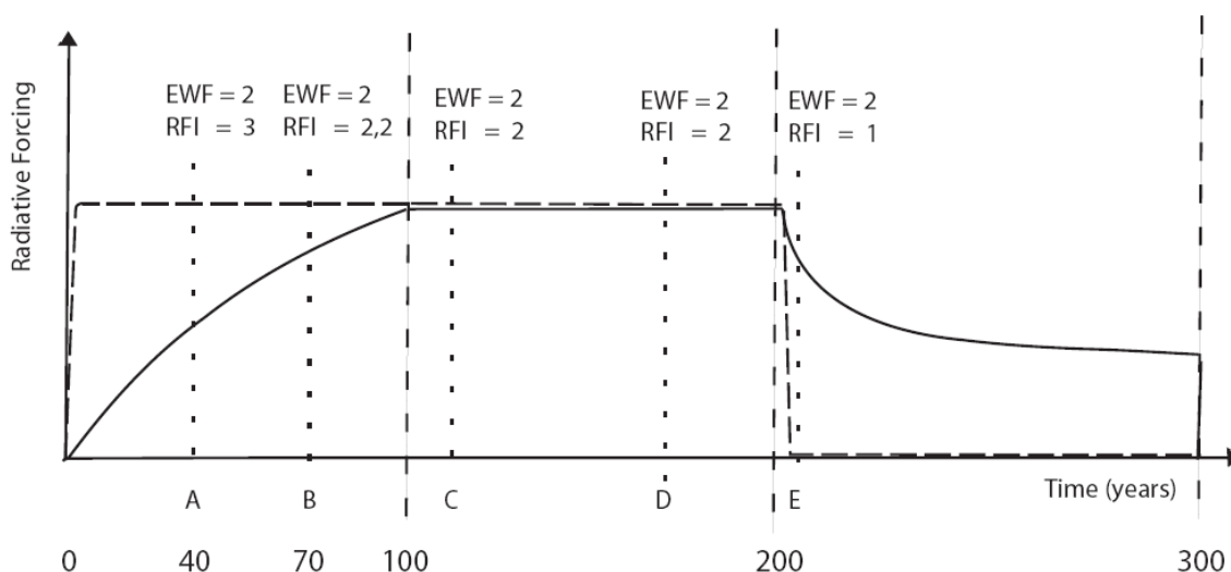
Figure 1: Radiative forcing as a function of time for \text{CO}_2 (full line) and the indirect effects of aviation (AIC, \text{O}_3 , \text{CH}_4 etc., dashed line). Emissions start in year 1, remain constant for 200 years and end in year 201. The numerical values are chosen illustratively as an example for an EWF of 2. \text{CO}_2 pulses are cut after a time horizon of 100 years, in analogy to the GWP. Furthermore, RFI values are given at certain points in time.
