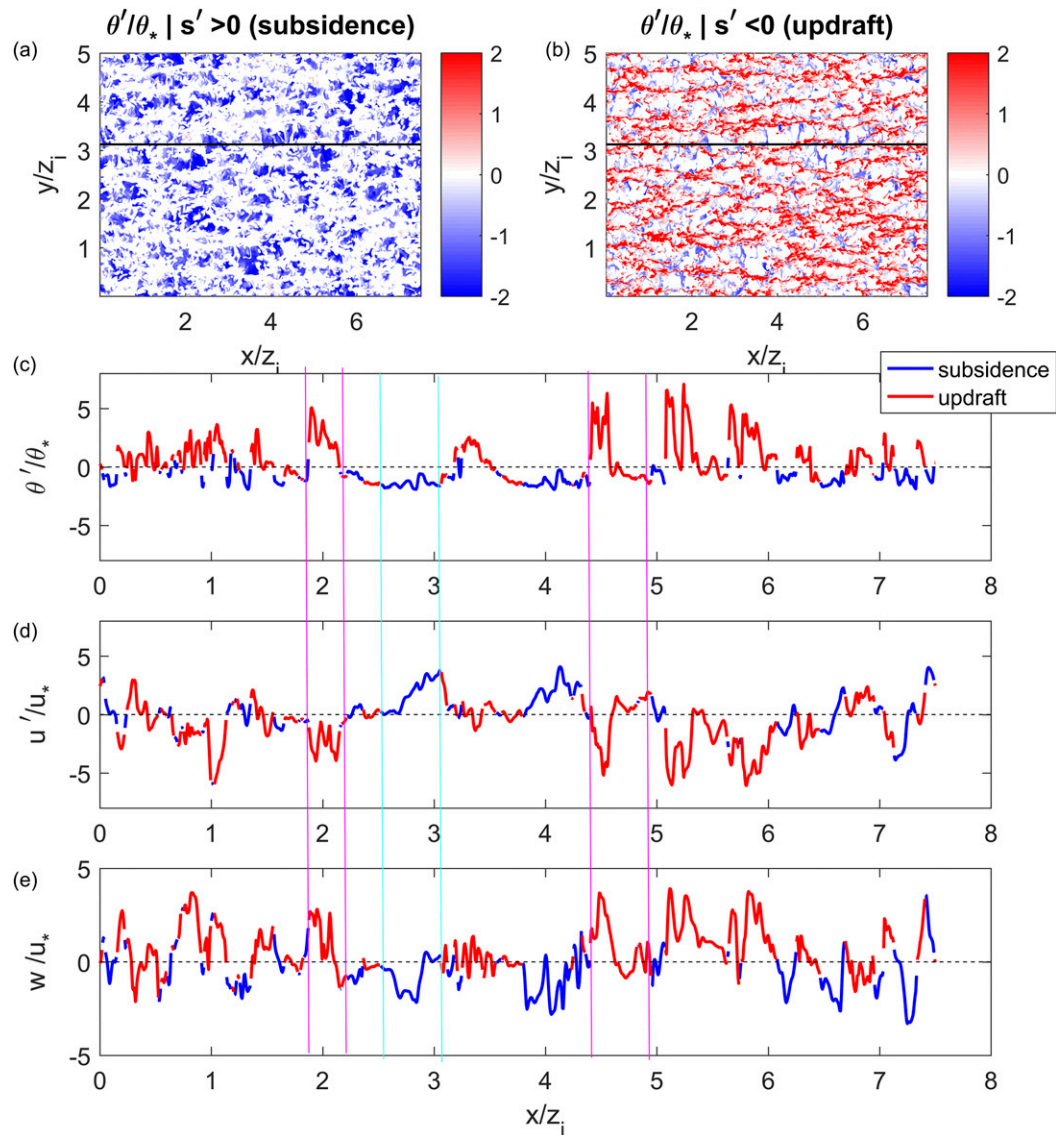
FIG. 1. (a) The x - y cross section of subsidence regions of \theta'/\theta_* . (b) The x - y cross section of updraft regions of \theta'/\theta_* . (c)–(e) Plots of \theta' , u' , and w along the black lines in (a) and (b).
