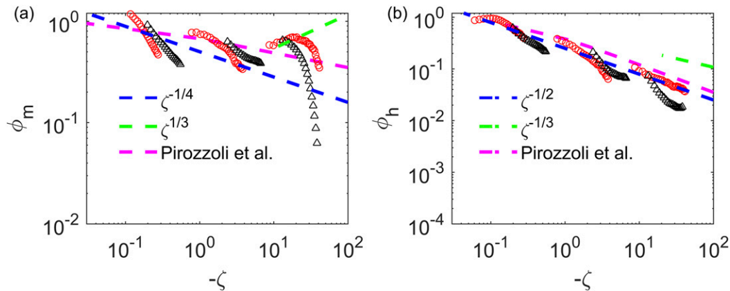
FIG. 2. The stability correction functions for (a) u and (b) \theta . Black triangles: DNS data; red circles: LES data. Blue dashed lines refer to the exponent in the classical Businger–Dyer relationships; green dashed lines are the free-convective limit predicted by Kader and Yaglom (1990); magenta dashed lines are (a) 1/0.399(1 - 14.6\zeta)^{-0.145} and (b) 1/0.375(1 - 5.67\zeta)^{-0.538} .
