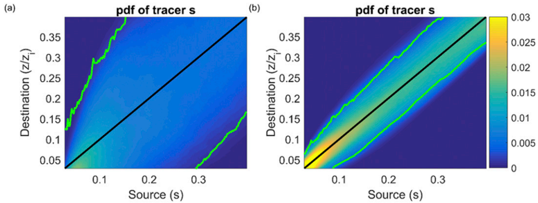
FIG. A1. The probability mass function of passive tracer s for different relaxation rate: (a) n = 1/3 and (b) n = 1/30 for the DNS run low-buoyancy case.
