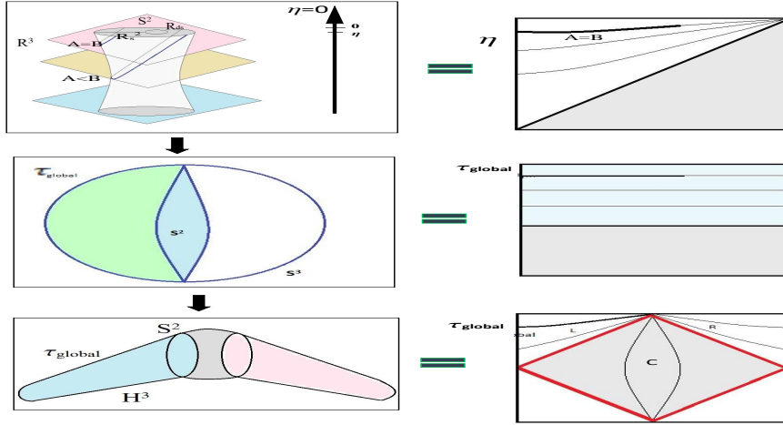
Figure 2. Schematic diagram for the geometrical construction and underlying symmetries of the bipartite quantum field theoretic system of de Sitter hyperbolic open chart. Corresponding Penrose diagrams are also drawn for completeness. \square
