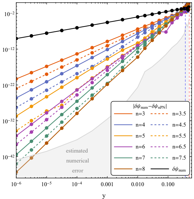
FIG. 2. Comparison of the numerical and PN results for \delta\psi in the weak field regime for \hat{a} = 0.9 . The plotted lines show the residual after subtracting the n th order PN approximation. The slopes of each line is compatible with an (n + 1/2) th order residual, as one would expect. The blue and red vertical dashed lines show the location of the ISCO and the light ring respectively. The shade region gives an estimate on the numerical error in the calculation of \delta\psi_{\text{num}} .
