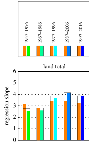
Figure 7. Regression slopes ( (\text{PgC yr}^{-1}) \text{K}^{-1} ) between interannual variations of global terrestrial NEE and of tropical mean air temperature (over 25^\circ \text{N} – 25^\circ \text{S} land regions, without decadal variations as used in the NEE– T inversion) for five 20-year windows. NEE has been estimated by the standard inversion (hollow black bars), the NEE– T inversion with the same ‘interannual climate sensitivity’ throughout 1957–2017 (as in figure 5, orange bars), and NEE– T inversions with independent sensitivities in each of the 20-year windows (green-to-blue bars). All inversions use the ‘quasi-homogeneous’ station set s57X. Before the regression, all time series were interannually filtered, and any linear trends have been removed.
