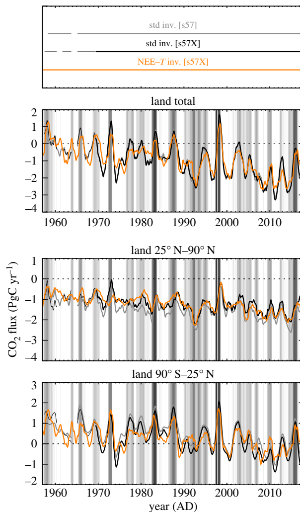
Figure 5. Interannual variations of NEE from standard and NEE–T inversions (IAV filtered/integrated as in figure 2). Black and orange runs use the ‘quasi-homogeneous’ station set s57X.
