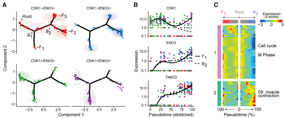
Figure 2. Single-Cell Trajectory Analysis with Monocle 2 Identifies Three MYOD-Mediated Myogenic Reprogramming Outcomes in hFib-MyoD
