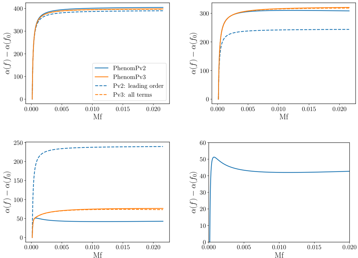
FIG. 1. Comparison of leading-order (IMRPhenomPv2: leading order ), NNLO (IMRPhenomPv2), full-PN (IMRPhenomPv3: all terms ), and the version we adopt in the final model (IMRPhenomPv3) expressions for the precession angle, \alpha . First panel: q = 1 , M_{\text{tot}} = 10M_{\odot} , \chi_{\text{eff}} = 0 , \chi_p = 0.9 ; second panel: q = 8 , M_{\text{tot}} = 10M_{\odot} , \chi_{\text{eff}} = 0 , \chi_p = 0.9 ; third panel: q = 10 , M_{\text{tot}} = 10M_{\odot} , \chi_{\text{eff}} = -0.8 , \chi_p = 0.1 ; fourth panel: same configuration as third panel, but zoom of non-physical behavior of \alpha_{v2}(f) . All cases are generated from a frequency of 2 Hz. See text for discussion.
