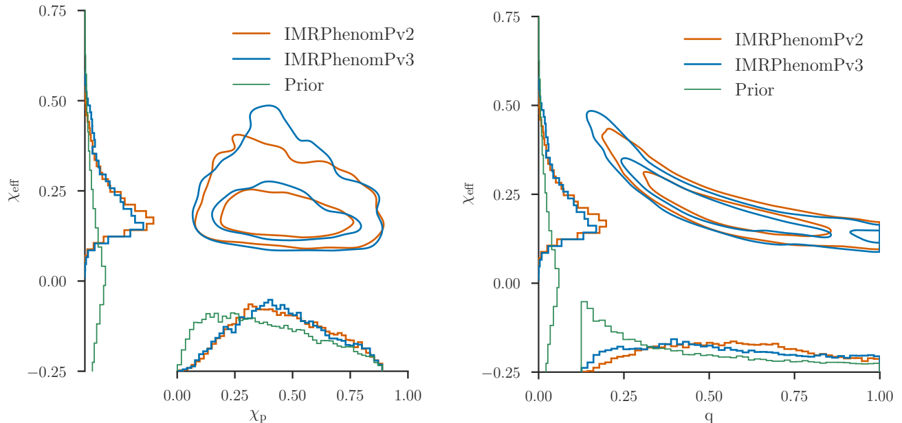
FIG. 5. Posterior probability densities for \chi_{\text{eff}} - \chi_p (left) and \chi_{\text{eff}} - q (right) for GW151226 using IMRPhenomPv2 and IMRPhenomPv3 . Despite the more accurate description of 2-spin dynamics of IMRPhenomPv3 the posteriors are consistent, demonstrating the difficulty of measuring 2-spin dynamics.
