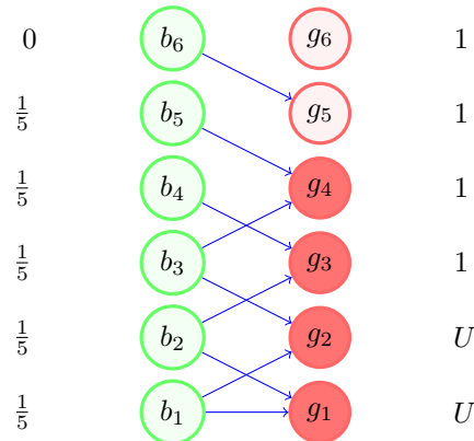
(b) The equality network changes for the first time. Edges (b_2, g_3) and (b_3, g_4) appear.
