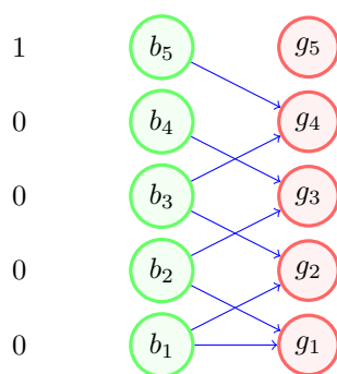
(a) The equality network N_p and the surplus vector with respect to f . Here k = 4 .
