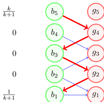
(b) Augmenting flow of \frac{1}{k+1} along a path from b_5 to b_1 (odd i ).
