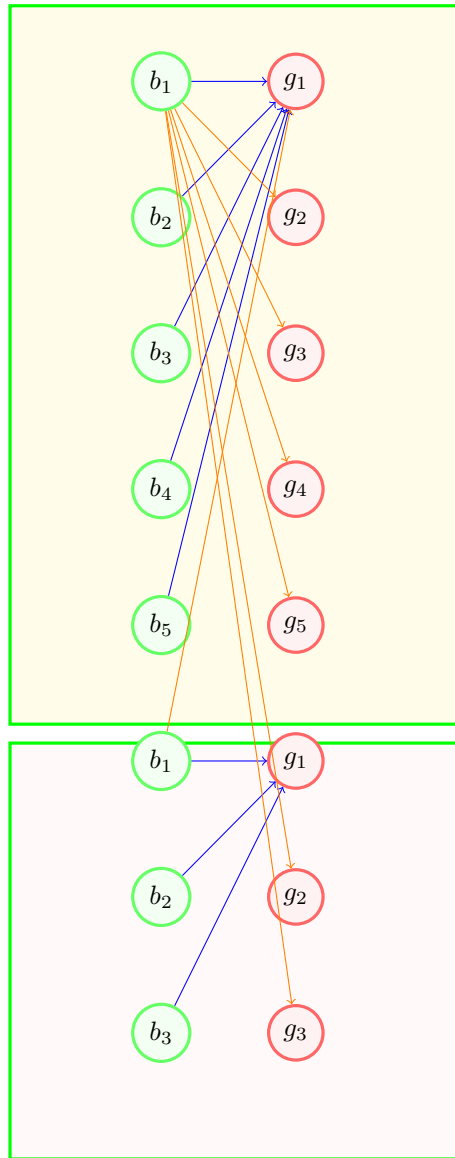
■ Figure 5 Utility graph where the agents are the nodes on the left and the goods are on the right. The agents have been partitioned into two disjoint blocks - block_1 (yellow block) and block_2 (pink block). In each block, agent b_i owns good g_i . The blue lines from b_i to g_j , indicates utility of U , and the orange ones a utility of 1.
