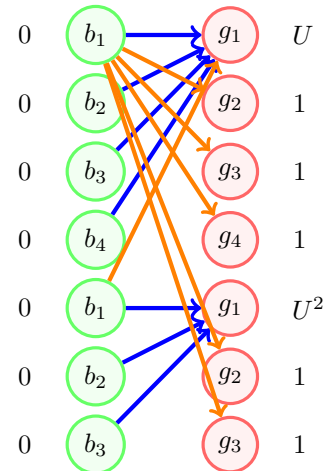
(c) The equality network changes for the second time. The edge from (b_1, block_2) to (g_1, block_1) appears.
