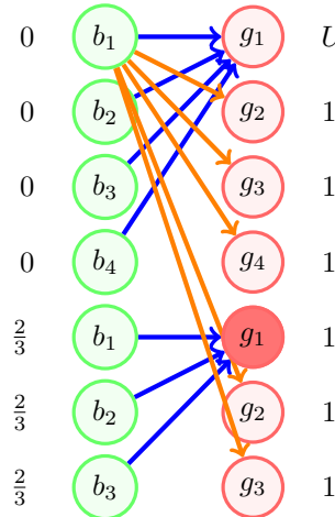
(b) The equality network changes for the first time. Orange edges appear. S = block_2 .
