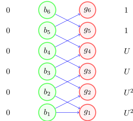
(c) The equality network changes for the third time. Edges (b_4, g_5) and (b_5, g_6) appear.
