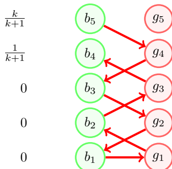
(c) Augmenting flow of \frac{1}{k+1} along a path from b_5 to b_4 (even i ).
