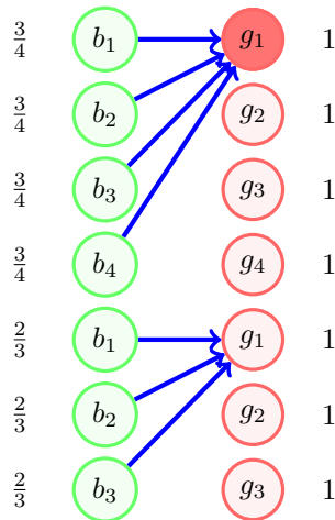
(a) During the first iteration of the algorithm in [10] on I'_n . We have S = block_1 .
