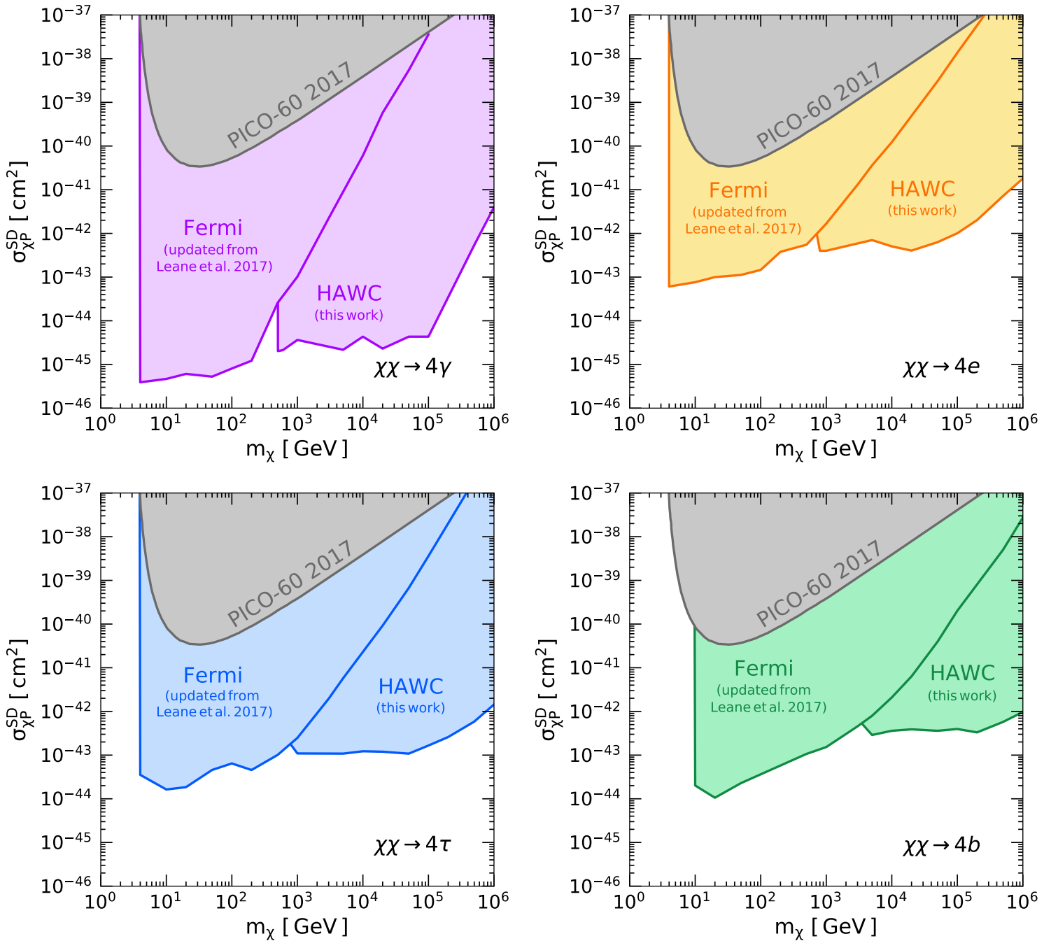
FIG. 3. The dark matter-proton spin-dependent cross section \sigma_{\chi p}^{\text{SD}} for annihilation into pairs of b\bar{b} , e^+e^- , \tau^+\tau^- , and \gamma\gamma , assuming an optimal mediator decay length equal to the solar radius; in less favorable models, which remain to be explored, the limits would be weaker. The Fermi-LAT constraints are updated from Ref. [32] using gamma-ray data from the Sun in the solar maximum (2014–2017). Also shown are the strongest direct detection constraints, obtained from PICO-60 [22].
