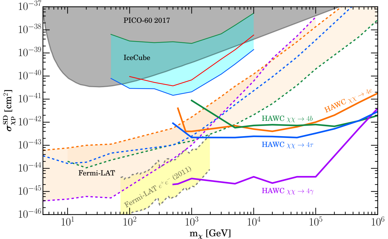
FIG. 4. Upper limits on the spin-dependent dark matter-proton scattering cross section \sigma^{\text{SD}} , from various gamma-ray and neutrino experiments. The thick solid lines show the limits obtained from HAWC in this work for \bar{b}b , e^+e^- , \tau^+\tau^- and \gamma\gamma channels. The dashed lines following the same channel-wise color scheme show the limits from Fermi-LAT for \bar{b}b , e^+e^- , \tau^+\tau^- and \gamma\gamma , updated from Ref. [32]. The HAWC and the Fermi-LAT limits are for scenarios where the mediator has a decay length L = R_\odot . The 2011 Fermi-LAT results are for mediators decaying into electrons, with decay lengths between 0.1 and 5 AU [56]. The thin solid lines show the results from IceCube for the \bar{b}b , W^+W^- , \tau^+\tau^- channels [29], and are for scenarios with short-lived mediators (results for long-lived mediators would be better [14, 32], but IceCube results are not yet available). The grey region indicates the parameter space excluded by PICO-60 [22].
