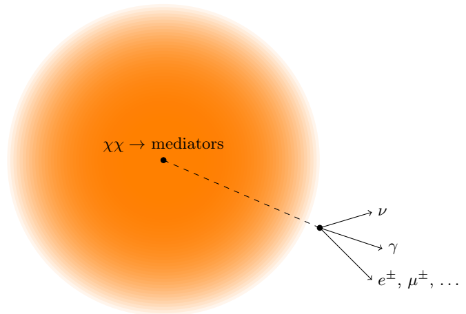
FIG. 1. Illustration of dark matter annihilation into long-lived mediators that decay to SM particles outside the solar surface (adapted from Ref. [32]).
