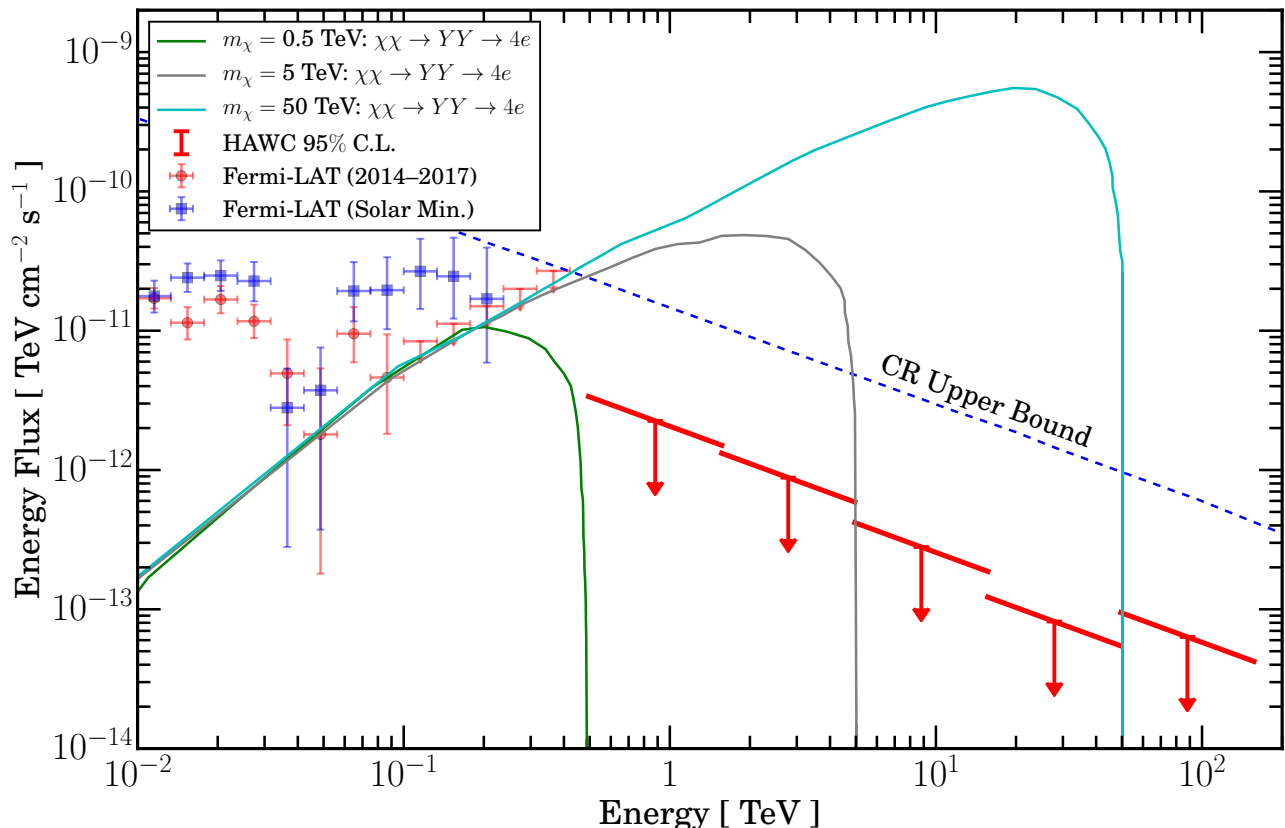
FIG. 2. HAWC 95% C.L. limits on gamma-ray flux from the Sun using three years of data [59]. The observed flux and the 90% upper limits by the Fermi-LAT spanning the same period are shown in red (2014–2017) [70]. The Fermi-LAT solar min. flux was measured during the solar minimum of the solar cycle 24. The dashed line shows the theoretical maximum flux produced by hadronic interactions [70]. Also shown are a subset of predictions for various dark matter masses obtained using nominal annihilation rates allowed by the Fermi measurements, showing the power of the new HAWC limits.
