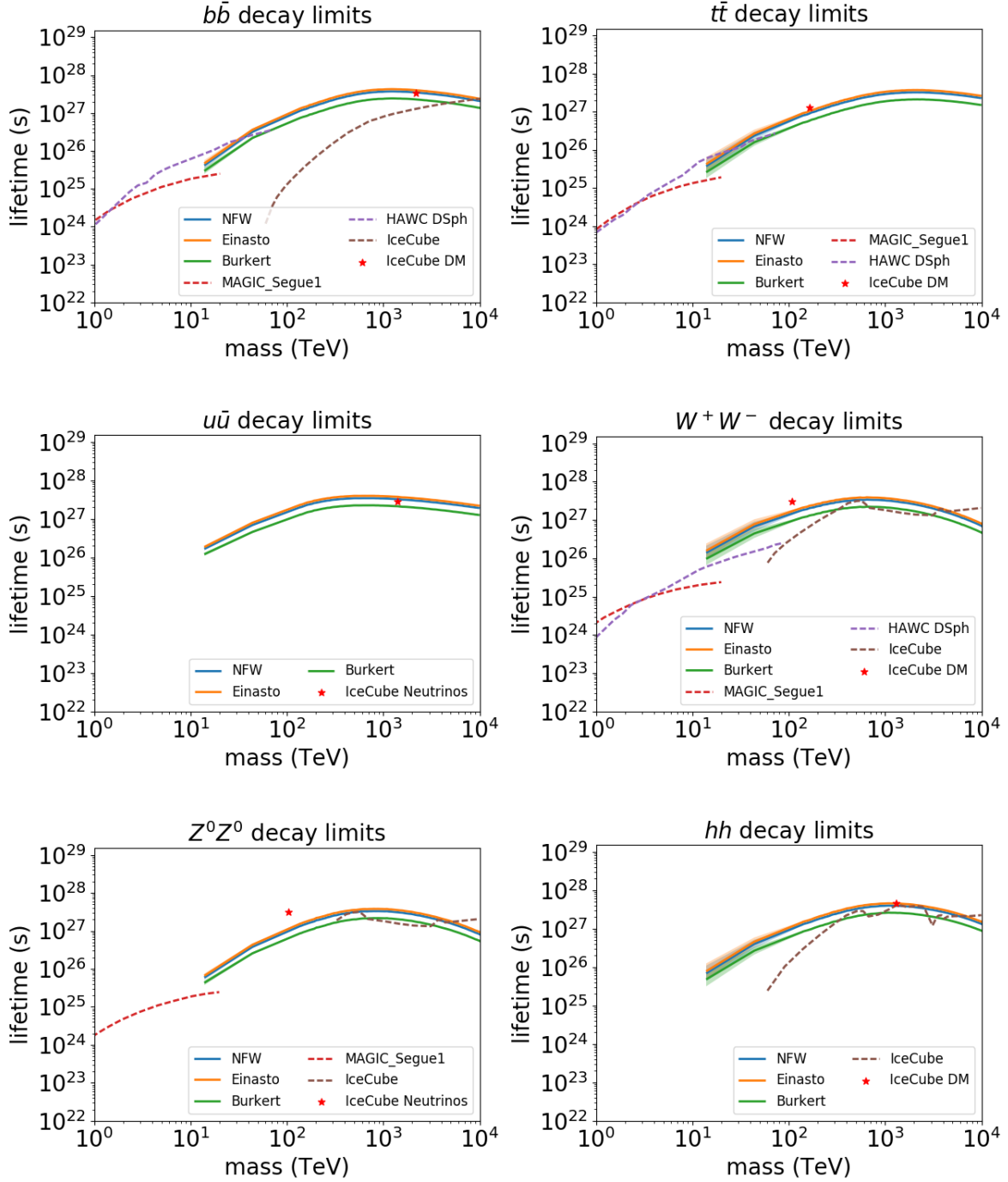
Figure 9. 95% confidence level lower limits on the DM decay lifetime for the hadronic and bosonic DM annihilation channels considered in this analysis. Limits for a Burkert (bottom, green), Einasto (top, orange), and NFW (middle, blue) profile are shown. Segue 1 dwarf galaxy limits from MAGIC [66] (lower left) are dashed in red. HAWC limits from dwarf galaxies (upper left) are shown dashed in purple. IceCube limits [67] are shown in brown (on right). The red star is a model in which the IceCube neutrinos are produced in decaying DM [7].
