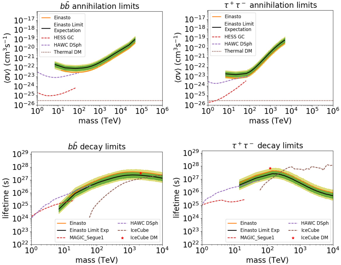
Figure 11. Demonstration of the statistical errors compared to the limits for b\bar{b} and \tau^+\tau^- DM annihilation and decay channels considered in this analysis. Limits for an Einasto (orange) profile are shown as in Figures 7-10. Segue 1 dwarf galaxy limits from MAGIC [66], GC limits from HESS [68], HAWC limits from dwarf galaxies, and the model for IceCube neutrinos from decaying DM [7] are also shown as in Figures 7-10. The black line is the expected value for the Einasto profile without any statistical fluctuations in the data. The green and yellow regions show the limits expected from 68 percent and 95 percent fluctuations from the black line. Note that the values observed in data are underfluctuations lying between the 68 and 95-percent regions.
