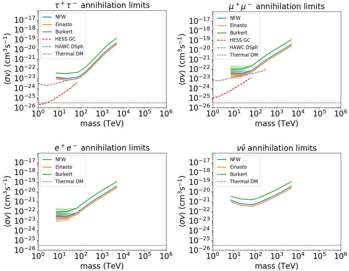
Figure 8. 95% confidence level upper limits on the DM annihilation cross-section for the leptonic and neutrino DM annihilation channels considered in this analysis. Limits for a Burkert (upper, green), Einasto (lower, orange), and NFW (middle, blue) profile are shown. All additional lines are as in Figure 7.
