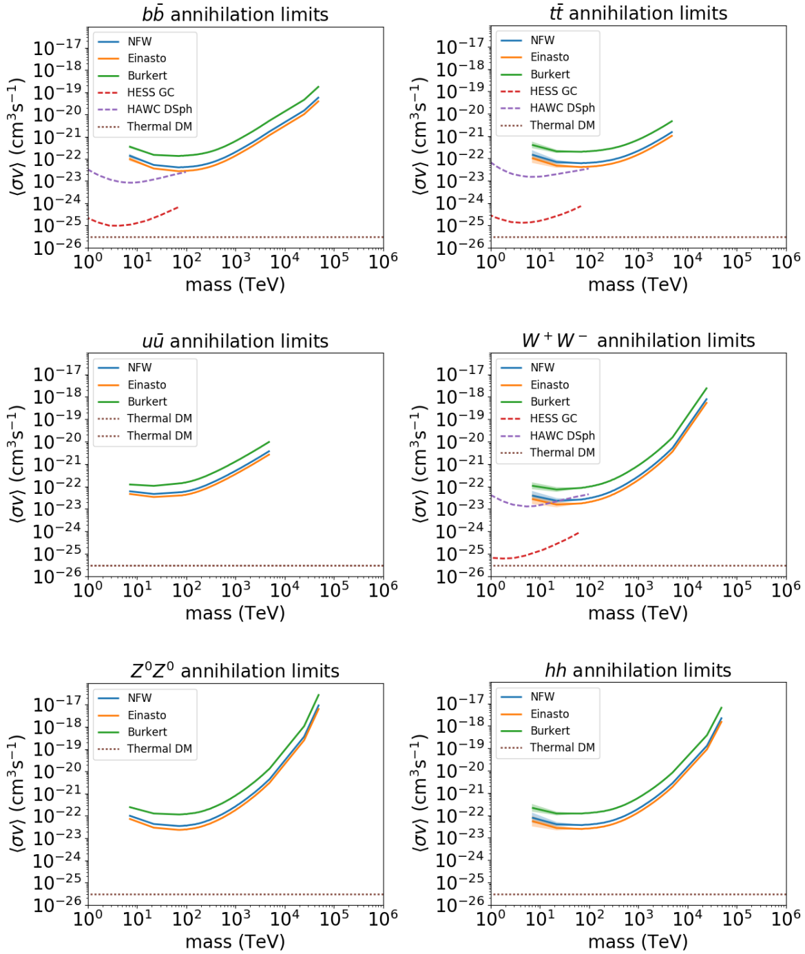
Figure 7. 95% confidence level upper limits on the DM annihilation cross-section for the hadronic and bosonic DM annihilation channels considered in this analysis. Limits for a Burkert (upper, green), Einasto (lower, orange), and NFW (middle, blue) profile are shown. GC limits from HESS (for Einasto profile) are shown near the bottom dashed in red. HAWC limits from dwarf galaxies are shown near the middle dashed in purple. The thermal dark matter cross-section is shown in brown for comparison (bottom).
