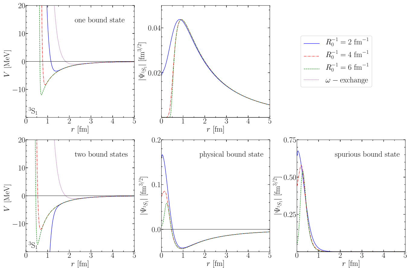
FIG. 2. Chiral LO potentials in the {}^3S_1 partial wave as well as the corresponding wave functions for one or two bound states for three cutoff values and n_1 = n_2 = n = 2 . In addition, we compare the chiral LO potentials with a potential where the short-range interaction is replaced by an \omega -meson-exchange potential.
