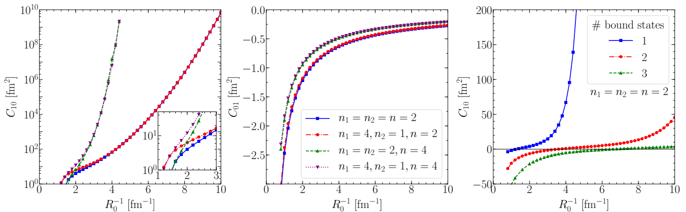
FIG. 1. Spin-isospin LECs C_{10} (left panel, logarithmic scale) and C_{01} (middle panel) as functions of the inverse cutoff R_0^{-1} for local chiral interactions at LO with different local regulators characterized by n_1, n_2, n . Right panel: Spin-isospin LEC C_{10} as function of the inverse cutoff R_0^{-1} for local chiral interactions at LO allowing one, two, and three bound states in the coupled {}^3S_1 - {}^3D_1 channel.
