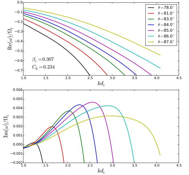
Figure 4. KAW—More oblique. Real (upper) and imaginary (lower) parts of the KAW dispersion relation, shown for different propagation angles \theta . We set \beta_e = 0.307 and C_0 = 0.234 for all calculations, but vary the propagation angle \theta . Here we see an instability in the range of wavenumbers 1 \lesssim kd_i \lesssim 4 . The distribution is unstable in the range 78^\circ \lesssim \theta \lesssim 87^\circ , and is maximally unstable at \theta \approx 85^\circ .
