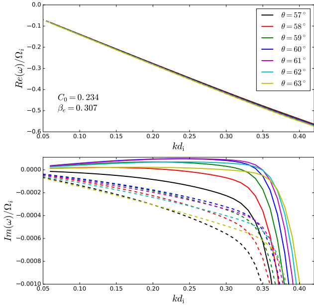
Figure A3. Magnetosonic. Dispersion relations for the original core-strahl model (solid lines, from Fig. 6) and the core-halo-strahl model (dashed lines) described in this appendix.
