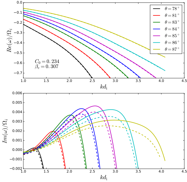
Figure A2. KAW—More oblique. Dispersion relations for the original core-strahl model (solid lines, from Fig. 4) and the core-halo-strahl model (dashed lines) described in this appendix.
