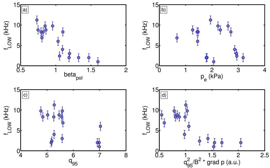
Figure 3: Frequency dependence of the low ( f_{\text{LOW}} ) frequency mode on: (a) normalized poloidal pressure ( \beta_{\text{pol}} ), (b) pedestal pressure ( p_e ) evaluated at \rho_{\text{pol}} of 0.98, (c) edge safety factor ( q_{95} ) and (d) normalized pressure gradient.
