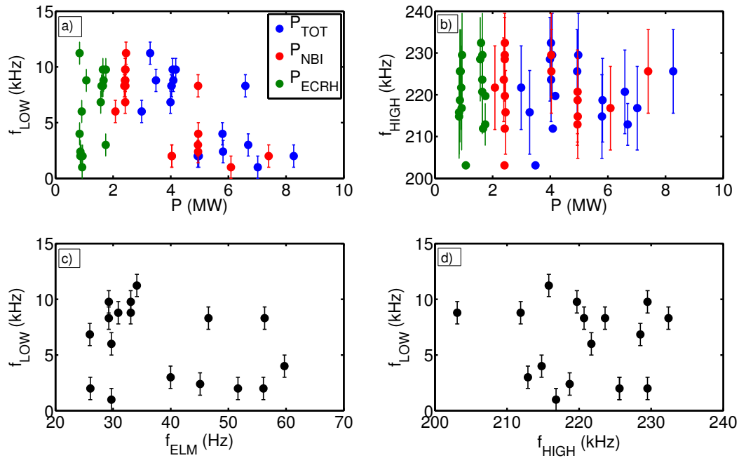
Figure 2: Frequency dependence of the low ( f_{LOW} ) (a) and high ( f_{HIGH} ) (b) frequency modes on the input ECRH, NBI and total power. In the bottom panels frequency of the low frequency modes is plotted against ELM repetition frequency ( f_{ELM} ) (c) and frequency of the high frequency modes ( f_H ) (d).
