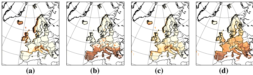
Fig. 1 Example results by Cancer and WNNMF on the Worldclim dataset. For each method, two selected columns from the left-hand factor matrix is shown on a map. The values are normalized to the unit interval, and darker shades indicate higher values. a Cancer high precipitation. b Cancer hot summer days. c WNNMF high precipitation. d WNNMF summer daily maximum temperature
