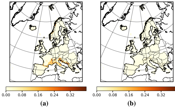
Fig. 3 Comparison of the overcovering when combining the Cancer factors from Fig. 1a, b using the standard (a) and the subtropical (b) algebras. All values are divided by the average value in the original matrix, negative values are ignored. Darker shades indicate higher values. a Overcovering when using the standard algebra. b Overcovering when using the subtropical algebra
