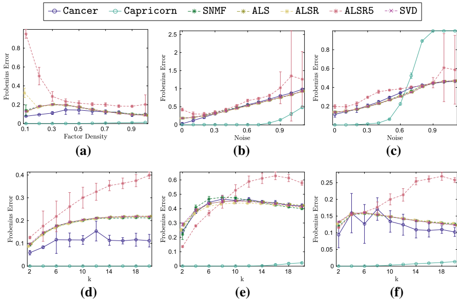
Fig. 6 Reconstruction errors on synthetic data with tropical noise. x -axis is the parameter varied and y -axis is the relative Frobenius norm. All results are averages over 10 random matrices and the width of the error bars is twice the standard deviation. a Varying density test. b Varying noise test. c Varying noise with high density. d Varying rank test with 10% noise and 30% factor density. e Varying rank test with 50% noise and 30% factor density. f Varying rank test with 10% noise and 60% factor density
