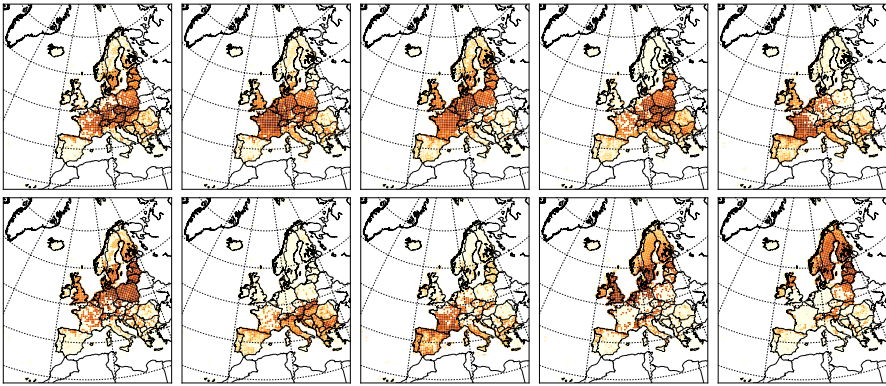
Fig. 16 Values in the factors by Cancer in the Mammals data plotted on a map. Every factor is normalized to take values from the unit interval and darker shades indicate higher values
