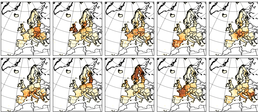
Fig. 17 Values in the factors by WNNMF in the Mammals data plotted on a map. Every factor is normalized to take values from the unit interval and darker shades indicate higher values
