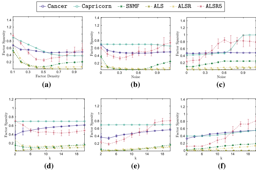
Fig. 7 Sparsity (fraction of zeroes) of the factor matrices for synthetic data with tropical noise. x -axis is the parameter varied and y -axis is the sparsity of the factors. The markers are averages of 10 random matrices and the width of the error bars is twice the standard deviation. a Varying density test. b Varying noise test. c Varying noise with high density. d Varying rank test with 10% noise and 30% factor density. e Varying rank test with 50% noise and 30% factor density. f Varying rank test with 10% noise and 60% factor density
