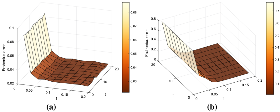
Fig. 4 Results of Cancer with different values of parameters t and f . a HPI. b Synthetic experiment with Gaussian noise
