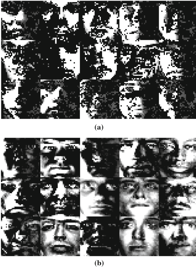
Fig. 14 Cancer finds the dominant patterns from the Eigenfaces data. Pictured are the left factor matrices for the Eigenfaces data. a Cancer. b ALS
