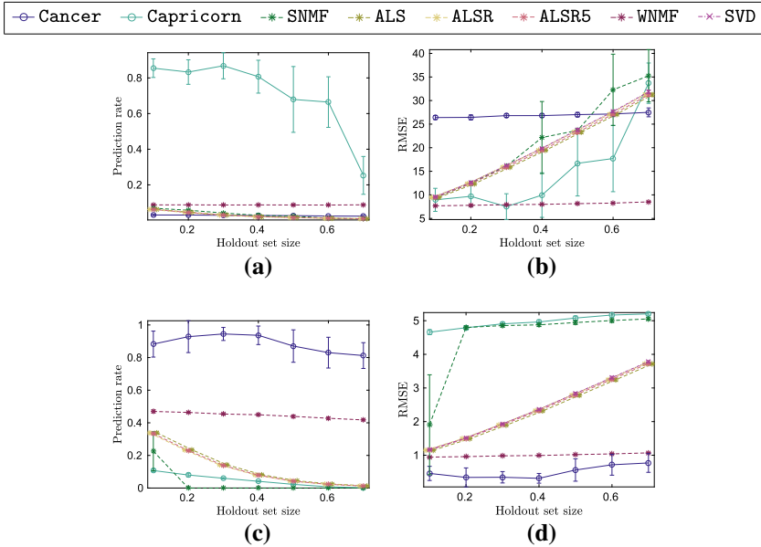
Fig. 12 Prediction rate on synthetic data with Gaussian noise. The x -axis represents the size of the holdout set. The y -axis is the correct prediction rate in (a) and (c), and RMSE in (b) and (d). The range is the interval that the values in input matrices are restricted to. All results are averages over 10 random matrices and the width of the error bars is twice the standard deviation. a Prediction rate, range [0, 100]. b RMSE, range [0, 100]. c Prediction rate, range [0, 9]. d RMSE, range [0, 9]
