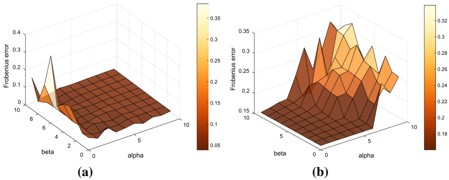
Fig. 5 Results of ALSR with different regularization parameters for the two factors matrices, which are denoted by \alpha and \beta respectively. a HPI. b Synthetic experiment with Gaussian noise
