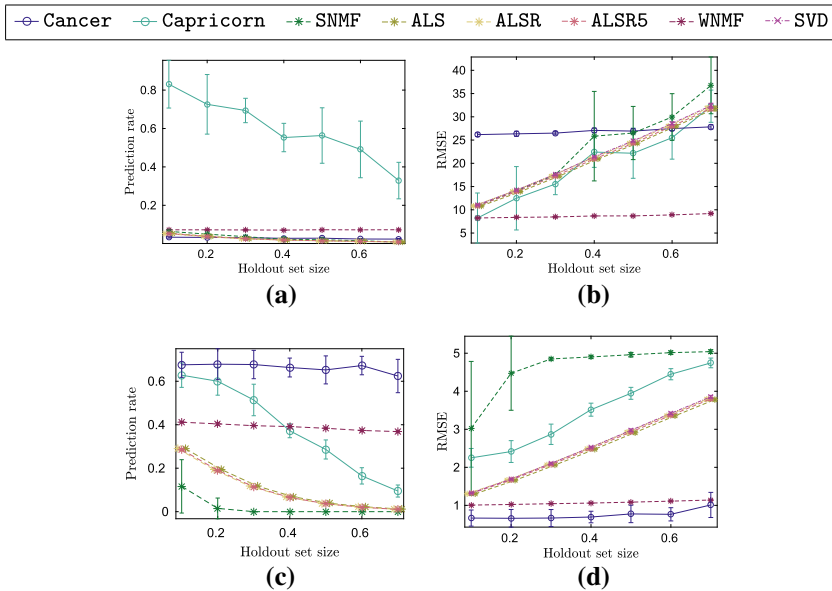
Fig. 11 Prediction rate on synthetic data with tropical noise. The x -axis represents the size of the holdout set. The y -axis is the correct prediction rate in (a) and (c), and RMSE in (b) and (d). The range is the interval that the values in input matrices are restricted to. All results are averages over 10 random matrices and the width of the error bars is twice the standard deviation. a Prediction rate, range [0, 100]. b RMSE, range [0, 100]. c Prediction rate, range [0, 9]. d RMSE, range [0, 9]
