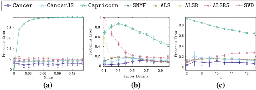
Fig. 10 Comparison of Cancer with Jensen–Shannon objective and other methods with Gaussian noise. x -axis is the parameter varied and y -axis is the relative Frobenius error. All results are averages over 10 random matrices and the width of the error bars is twice the standard deviation. a Varying noise test. b Varying density test. c Varying rank test with 10% noise and 30% factor density
