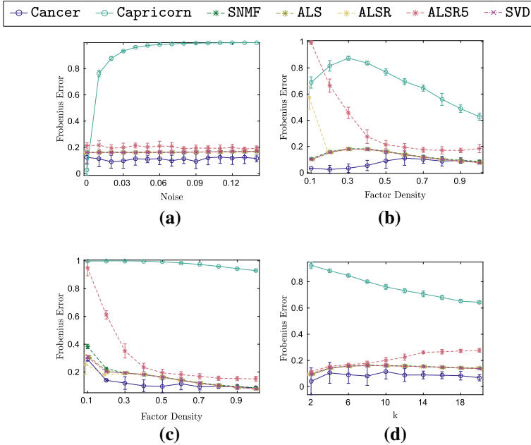
Fig. 8 Reconstruction error (Frobenius norm) for synthetic data with Gaussian noise. The markers are averages of 10 random matrices and the width of the error bars is twice the standard deviation. a Varying noise with density 50%. b Varying density with low Gaussian noise. c Varying density with high Gaussian noise. d Varying rank; 50% density and low Gaussian noise
