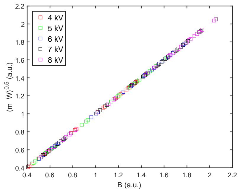
Figure 1.6: Test curve for mass calibration method described in the text. Each point corresponds to one mass peak in one particular acquisition. After performing the magnetic field to current fit all points align on the same straight line proving the validity of the analysis. Each data point corresponds to a measurement of Fig. 1.7
