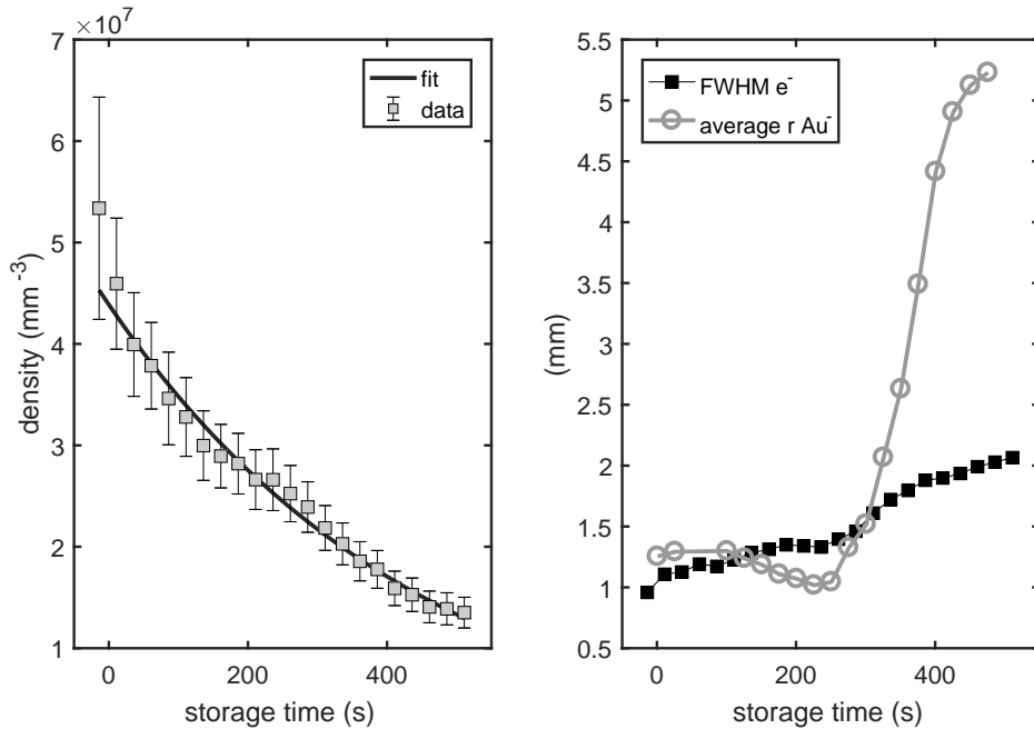
Figure 3.11: Left pane: On-axis density of the electron plasma as a function of the storage time. The exponential fit n_0 \exp(t/\tau) + n_{inf} gives n_0 = 4.56(38)10^7 \text{ mm}^{-3} , \tau = 4.52(85)10^2 \text{ s} , n_{inf} = -2(5)10^6 \text{ mm}^{-3} . Right pane: Dimension of the plasma are reported. As dimension of the e^- we report the radius where the e^- reaches half of the on-axis value. As dimension of Au^- the average of the radial position is used. The solid lines are meant to guide the eye.
