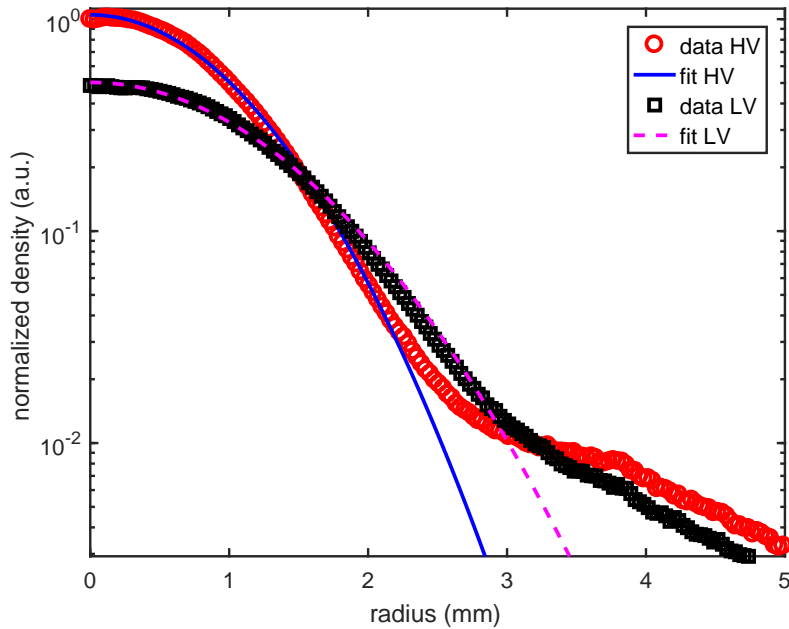
Figure 3.14: Radial profiles of ion clouds acquired by dumping anions from different storage potential after 100 s storage time. Ions were loaded in HV configuration and projected onto the detector either in HV or in LV configuration. Voltages applied were: (Front, center, back) = x + (-50, 0, -60) V with x_{HV} = -795 V and x_{LV} = -205 V with x indicating the floating potential of the trap. The fit lines are Gaussian profiles of the expression a \exp(-r^2/w^2) . The fit yielded a_{HV} = 358.7(4) w_{HV} = 1.172(2) mm and a_{LV} = 172.1(2) w_{LV} = 1.521(2) mm.
