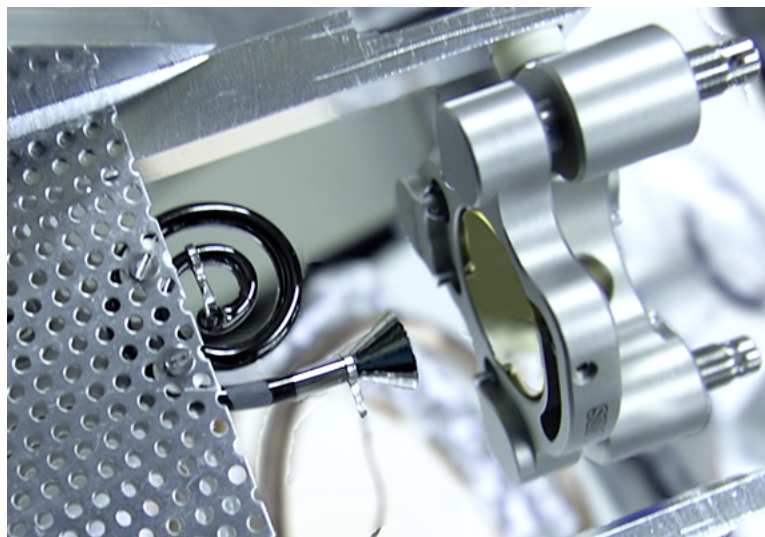
Figure 2.4: Photo of the channeltron detector facing the gold mirror. The 1-inch (25.4 mm) mirror is mounted after the aperture of the final electrostatic deflector in Fig. 2.3.
