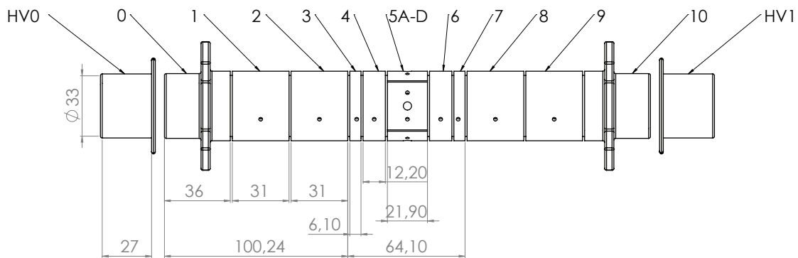
Figure 1.10: Schematic view of the electrodes of the Penning trap. Dimensions are in millimeters. The central electrode is split into four angular segments for rotating-wall excitation. Labels of the electrodes are indicated above.
