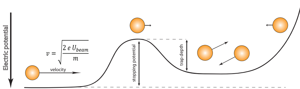
Figure 3.4: Schematic of the trapping principle. Anions approach the trapping region with energy U_{beam} and climb the stopping potential. Momentum transfer into the radial direction in trapping region may lead to stable confinement due to the reduction in the axial velocity component.
