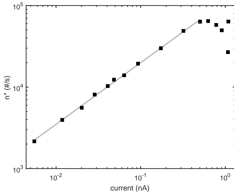
Figure 3.18: Loading ions for different currents. In the plot the solid line is a fit coefficient \alpha of Eq. 3.5. The fitted power law in the first part n^* = \alpha I^\beta with \alpha = 113(4)10^3/s and \beta = 0.75(1) . Front, central, back and floating potentials were -50 V, 0 V, -50 V and -795 V respectively. The loading time was varied between 1 s and 64 s.
