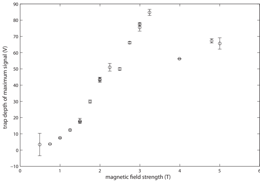
Figure 3.7: Optimal trap depth as a function of the confining magnetic field. Adapted from [91].
