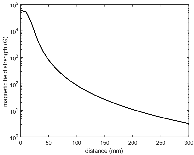
Figure 1.11: Axial magnetic field strength as a function of the distance from the center of the solenoid. The field is 6 T in the central region.
