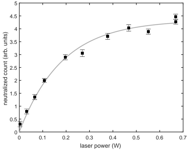
Figure 2.9: Relative number of excited \text{La}^- anions as a function of laser power. The effect of saturation can be observed from the non linearity of the curve. The solid line is a fit to the data with the function a(1 - \exp\{-bW\}) (see text).
