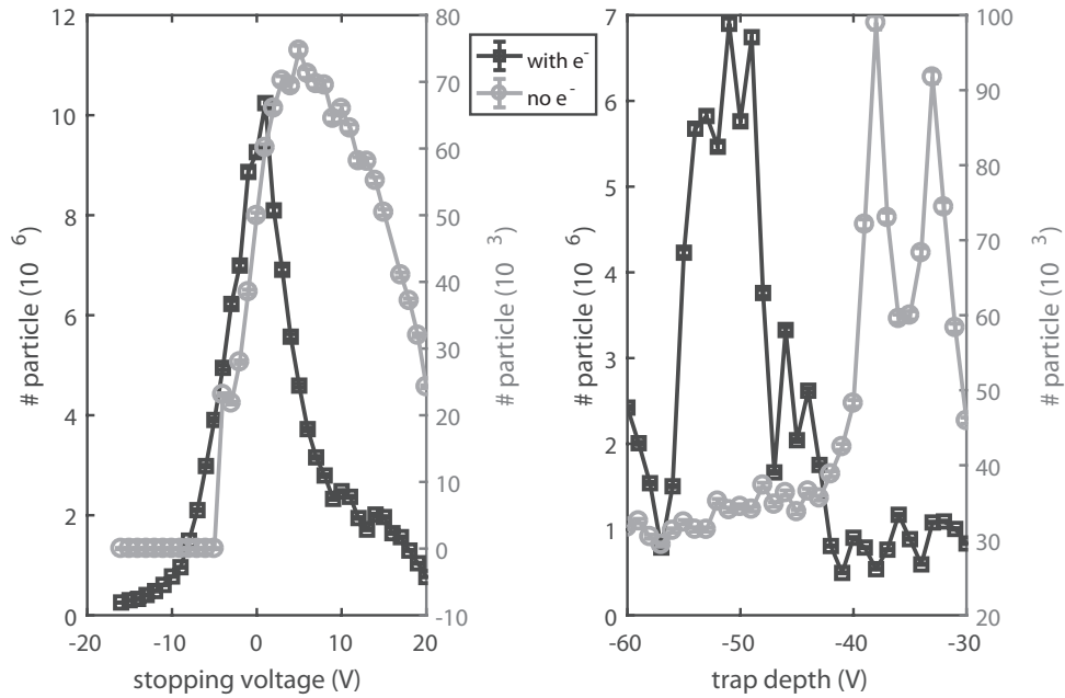
Figure 3.8: Number of anions trapped as a function of the stopping voltage (left) and trap depth (right). Ions were loaded for 20 s at a beam energy of 1006 eV with and without electrons. Data acquired with and without electrons are compared in the plots. Data acquired with no e^- pre-loaded in the trap have the scale on the right side of the plots. The lines are meant to guide the eye. Left Pane: Stopping voltage is relative to the anion beam energy. Front, central and back potentials were 5 V, 56 V and -100 V for acquisition with electrons and 5 V, 44 V, -100 V for data acquired without electrons. Right Pane: Influence of the trap depth on the trapping efficiency. Floating, front, back potentials were -1008 V, 5 V, -100 V respectively.
