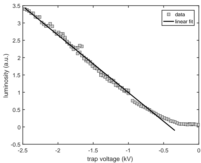
Figure A.3: Fluorescence signal obtained releasing anions from different reference voltage. The linear fit y = ax + b gives a = -6.7(2)10^2 \text{ V}^{-1} and b = -1.66(6) .
