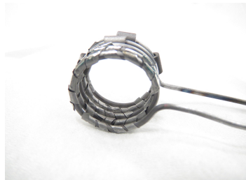
Figure 1.3: One of the first experimental attempts to modify the ionizer material. Platinum thin foils were wrapped around the surface of a W ionizer.
