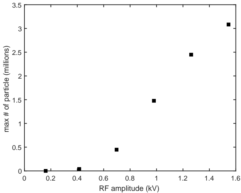
Figure 3.16: Maximum trapped particle number as a function of the RF amplitude. Experimental condition are reported in Fig. 3.15. The experiment was repeated several times for different V_{pp} and in this plot we show only the maximum values of each measurement.
