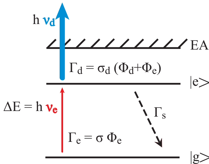
Figure 2.2: Simplified energy level diagram in a negative ion with the ground state |g\rangle , a bound excited state |e\rangle and the electron affinity EA . The light radiations have energy h\nu , photon densities \phi , and they induce transition rates \Gamma depending on the cross-section \sigma . The photodetachment (subscript d ) light has higher power than the excitation radiation (subscript e ) because the photodetachment cross-section \sigma_d is much lower than than cross-section \sigma of the resonant transition. In our spectroscopy experiments the contribution to the photodetachment rate \sigma_d\phi_e and the spontaneous emission rate \Gamma_s could be neglected.
