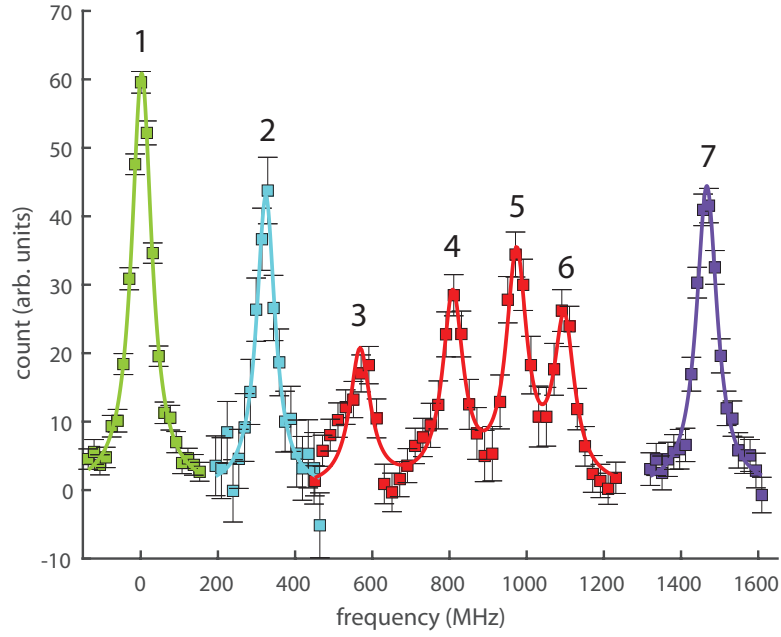
Figure 2.7: Composite graph of the {}^3F_2^e \rightarrow {}^3D_1^o resonance in \text{La}^- , resolving its hyperfine structure. Different colors correspond to four different acquisitions combined in this plot. Solid lines are Lorentzian fits of the peaks. The FWHM of Peaks 1–6 was found to be 64.3(1.5) MHz.
