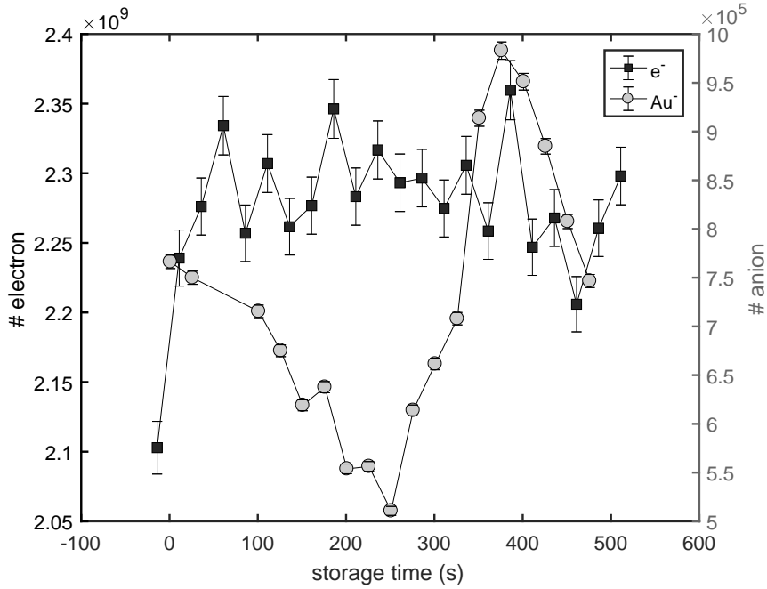
Figure A.5: Number of anions and electrons detected during the sympathetic cooling experiment. During the centrifugal separation of the two species there is an apparent increase in the number of anions.
