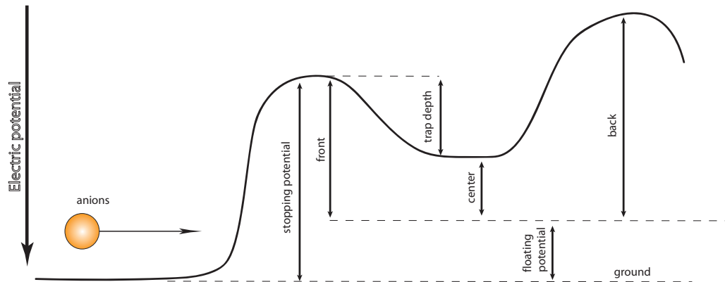
Figure 1.9: Schematic of the trapping DC voltage designation for axial confinement.
