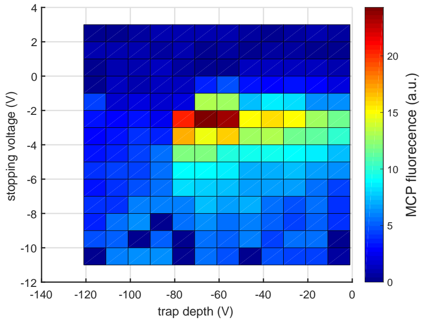
Figure 3.5: Trapping efficiency as function of stopping voltage and trap depth. The stopping voltage is relative to the beam accelerating voltage of -471 V. The magnetic field was 5 T, and anions were loaded for 5 s.
