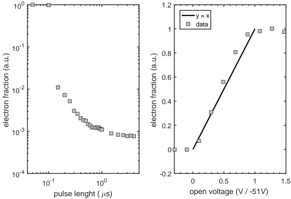
Figure 3.3: Fraction of ejected/detected electrons as a function of the ejection pulse time. The fraction of electrons is measured by taking a reference image of the content of the trap without the pulse. End caps electrodes were made by connecting 0-2 and 8-10 electrodes, while the central connecting 3-7 electrodes. The trap depth was -51 V. Left pane: Fraction of remaining e^- in the trap with a pulse of -51 V on the front electrode for different pulse lengths. Right pane: Fraction of ejected electrons as a function of the pulse amplitude with a 1 \mu\text{s} pulse. The pulse amplitude is given normalized to the front potential at trapping ( -51 V). The line corresponding to the equation x = y is shown to guide the eye.
