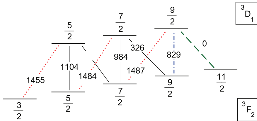
Figure 4.1: Laser cooling transition in \text{La}^- . In the picture the hyperfine levels are indicated by their respective F total angular momentum quantum number. The number on the line connecting the states indicates the transition frequency in MHz relative to 11/2 \leftrightarrow 9/2 . The colored lines (red, green, blue) indicate different laser frequencies for laser cooling and repumping.
