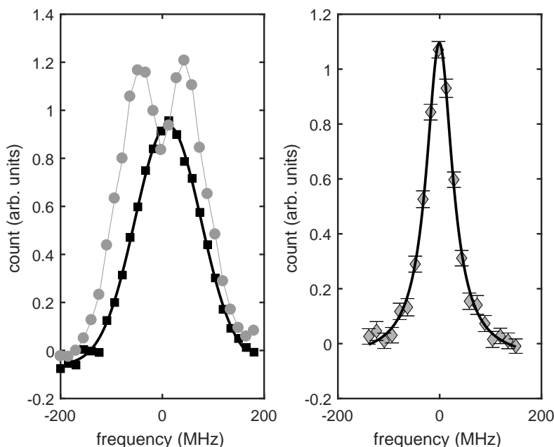
Figure 2.6: Data of the 11/2 \longleftrightarrow 9/2 hyperfine transition. Left pane: single (black) and double (gray) pass signal of transverse spectroscopy. The solid black line is a Gaussian fit to the data while the gray line helps to guide the eye. The dip resonance is calculated as described in the text and shown separately in the right pane, where the solid line corresponds to a Lorentzian fit to the data.
