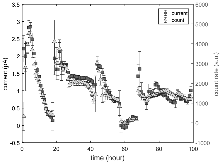
Figure 1.5: Measured current of La^- on the last Faraday cup (squares, left scale) and count neutral rate induced by the laser (triangles, right scale). The degradation behavior in the source caused by the ionizer poisoning is visible between hours 57 and 68 as a short-circuit. The neutral count rate is the corresponding neutral production rate of photodetached atoms by the laser (see Ch. 2)
