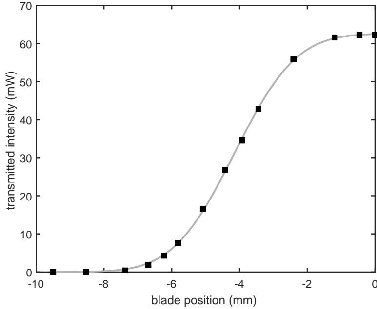
Figure 2.8: Measurement of the laser beam profile performed by progressively obstructing the beam with a blade while recording the transmitted power. The fit function I_0 \left(1 + \operatorname{erf}\left(\frac{x-\mu}{w}\right)\right) . In this measurement I_0 = 62.6(3) mW, w = 2.86(4) mm and \mu = -4.14(2) mm
