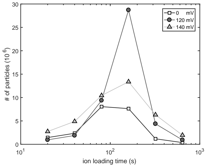
Figure 3.9: Number of anions as a function of loading time. If electron are kept compressed using the rotating wall excitation the loading can last longer, increasing the total number of captured anions. The rotating-wall frequency was 3 MHz with the peak to peak amplitude specified in the legend. The lines are meant to guide the eye.
