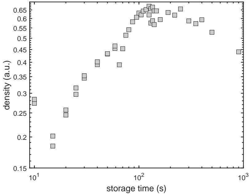
Figure 3.19: Density of anions on the axis of the Paul trap as function of time. As the storage time elapses the particle plasma cools down, resulting in a higher density of particles in the middle of the trap.
