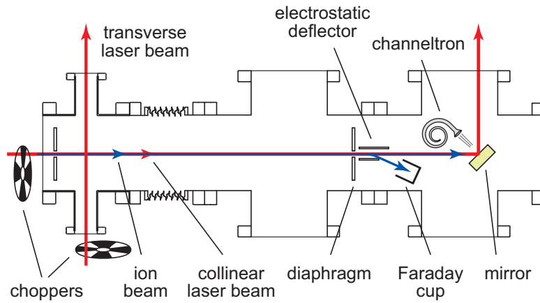
Figure 2.1: Sketch of the collinear/transverse laser spectroscopy setup (top view) with an overlap region of 730 mm. The ion beam is indicated by a blue line, the laser beams by red lines.
