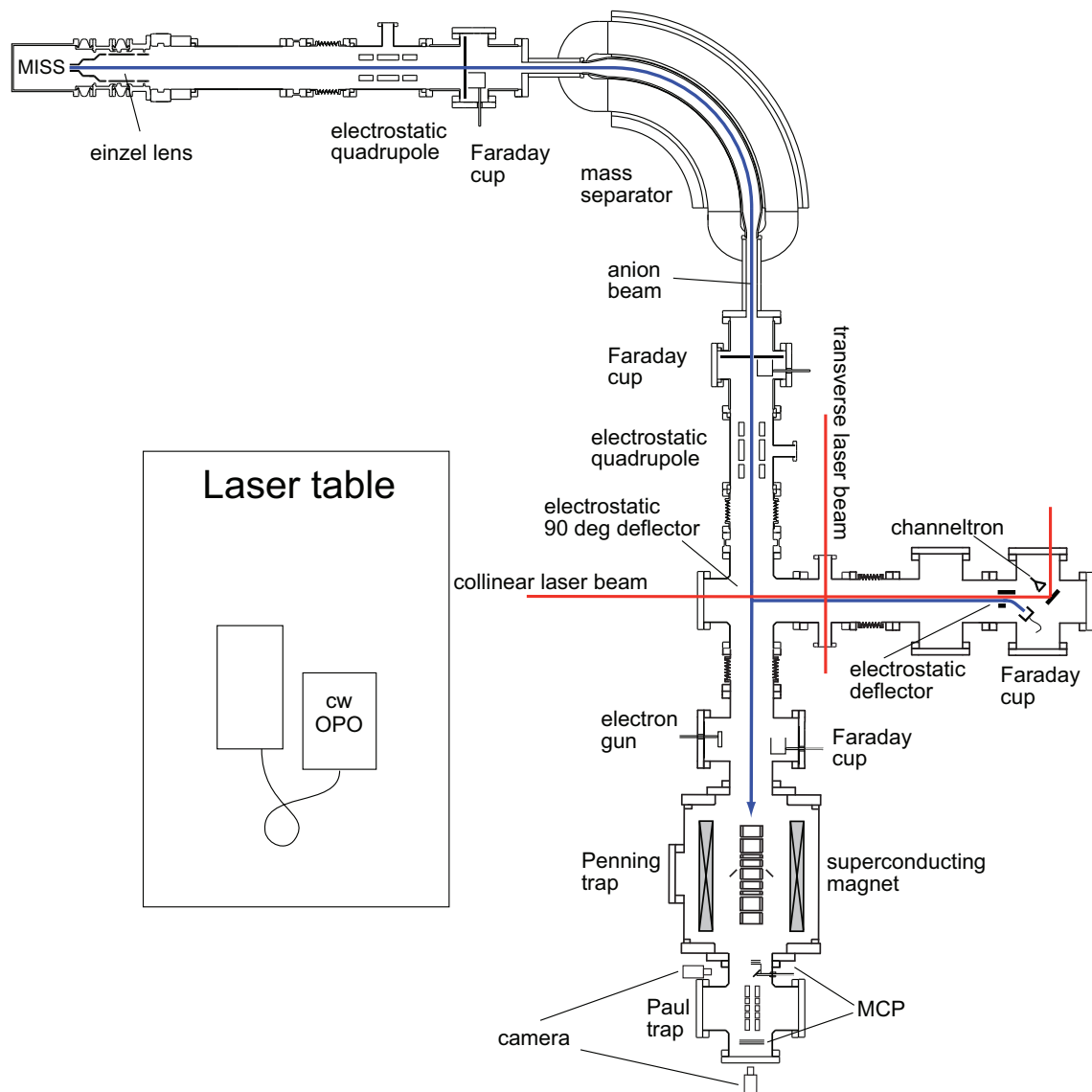
Figure 1.1: Schematic drawing of the experiment.
