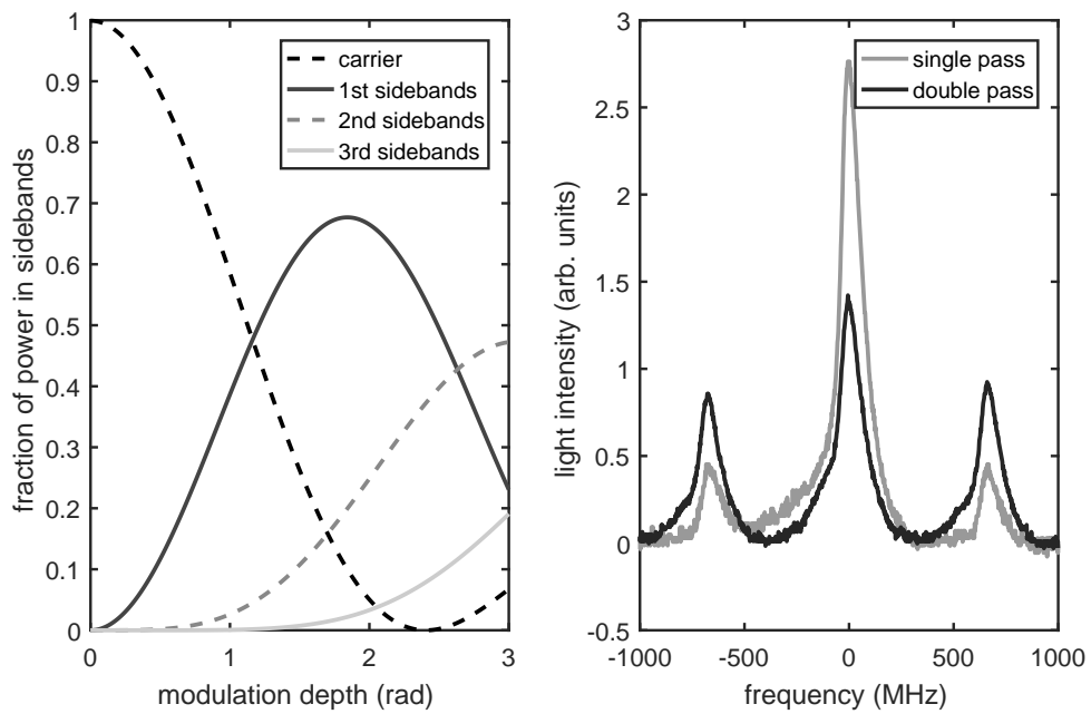
Figure 1.15: The left pane shows the relative power driven into the sidebands at different phase modulation depth b (Eq. 1.4 in the text). The right pane shows the measurement of the sidebands of the 665 MHz modulator performed by scanning Fabry-Perot cavity. In the plot of the transmitted intensity as a function of frequency. In single-pass configuration b \approx 0.71 rad to and in double-pass b \approx 1.3 rad.
