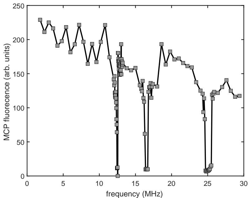
Figure 3.2: Number of remaining electrons as a function of the axial excitation frequency. Some resonances, corresponding to plasma eigenfrequencies, are visible in the spectrum. DC voltages of (-105 V, 0 V, -600 V) were applied respectively to front, center and back trap electrodes labeled 8, 9, 10. An oscillating potential of amplitude 10 V was superimposed to electrode 9 for 10 ms.
