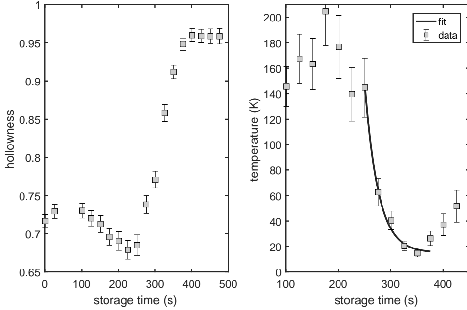
Figure 3.12: Hollowness (Eq. 3.1) and temperature evolution as a function of storage time. Left pane: Hollowness calculated as described in the text. The phase transition of centrifugal separation is evident around 300 s. Right pane: Calculated temperature of the anions during the transition. The solid line is an exponential fit T_0 \exp(t/\tau) + T_{inf} to the data with parameters T_0 = 2(9)10^6 K, \tau = 25.5(9.0) s, T_{inf} = 15(6) K.
