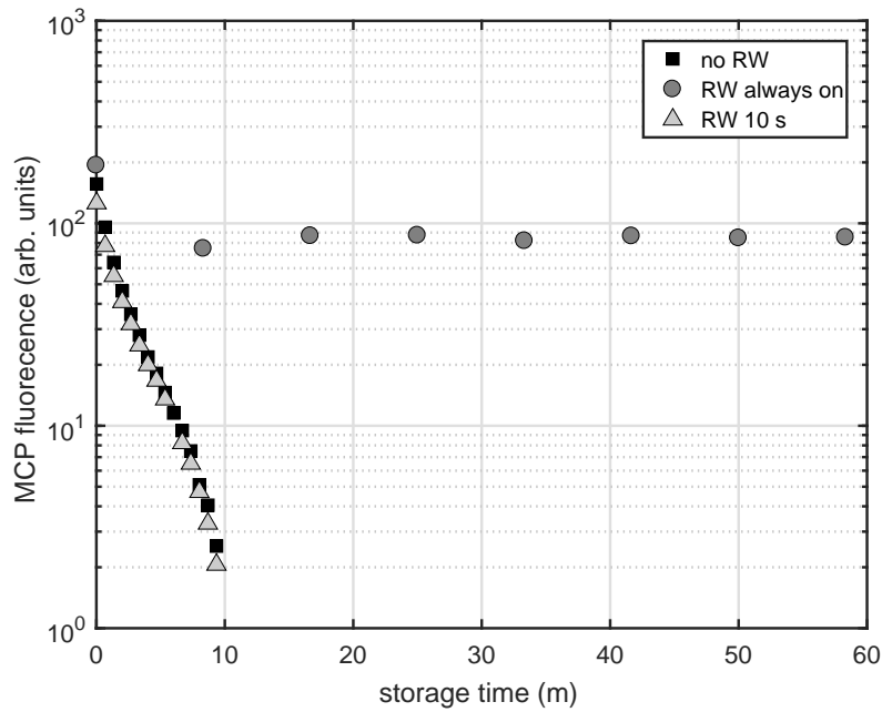
Figure 3.1: Number of remaining electrons as a function of the storage time in the long trap. The measurement shows how a constant rotating-wall drive may extend the lifetime of the trapped electrons by preventing plasma expansion and losses, as described in the text. The applied rotating-wall waveform at 5 MHz had an amplitude of 5 V only for 10 s ( RW 10 s ) or 0.5 V for the entire time ( RW always on ).
