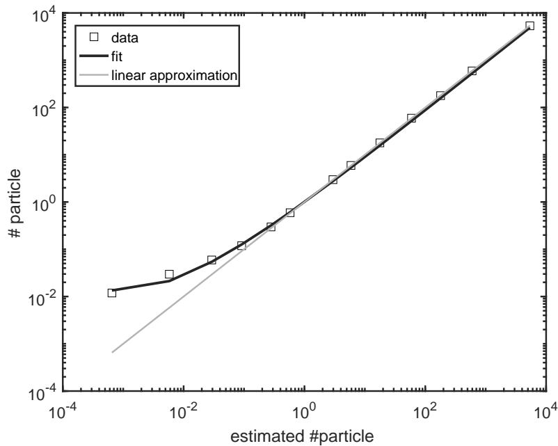
Figure A.2: The plot compares the number of detected ions using the approximation of Eq. A.1 against the real number of impinging ions. The scale is in particle per pixel. The second step of the calibration Eq. A.2 is the fit line. The correction takes into account the saturation at low particle number. The linear approximation follows the relation n = n' .
