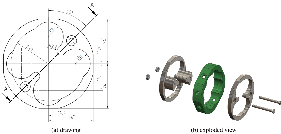
Figure 1.13: Transverse cut and exploded view of one DC fast switching electrode. It is mounted on the plastic insulator depicted in green that defines mutual distances and parallelism relative to the cylindrical rods. The length of the assembled electrode is 18 mm.
