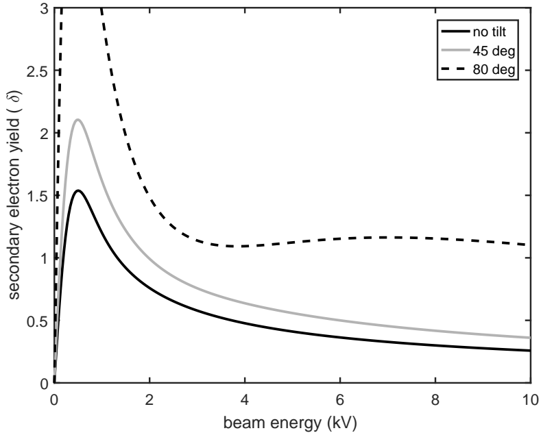
Figure 2.5: Calculated secondary electron emission from gold. Different curves correspond to different angles between the normal to the surface and the incoming particle. The spectroscopy on \text{La}^- reported in this work was performed with a mirror tilted 45^\circ with respect to the incoming neutrals. The collinear measurement in [85] was made at larger angle, closer to 80^\circ .
