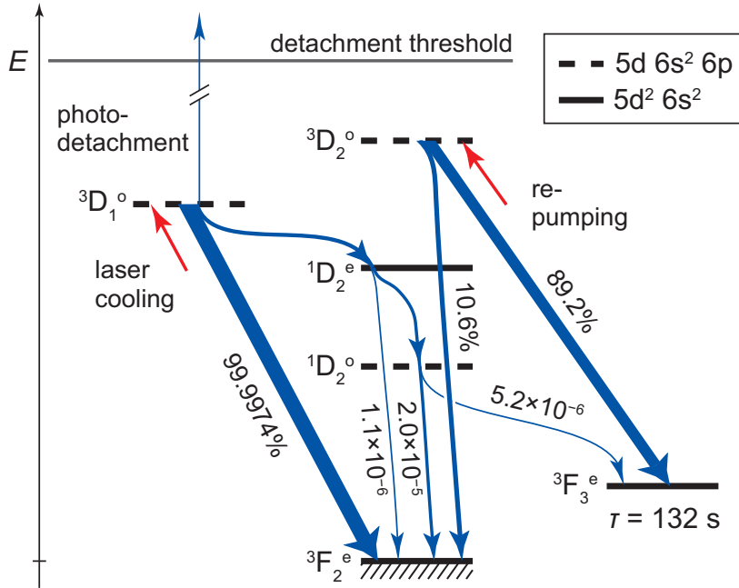
Figure 4.3: Partial energy level diagram of \text{La}^- (energies to scale). The relevant decay branches from the ^3D_1^o excited state of the laser cooling transition, as well as from the ^3D_2^o excited state of the repumping transition, are indicated. Branchings at least two orders of magnitude smaller than those indicated have been neglected. Thicknesses of blue arrows are indicative of branching ratios, but not to scale.
