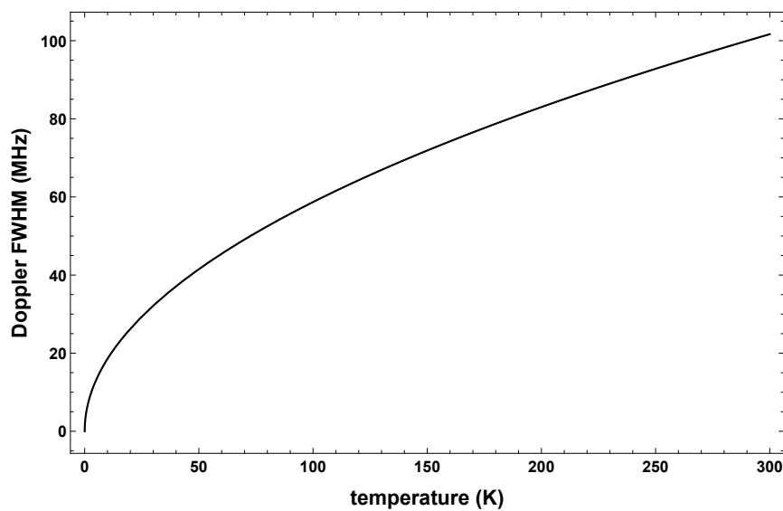
Figure 4.2: Doppler broadening of the transition lines for \text{La}^- as a function of temperature.
