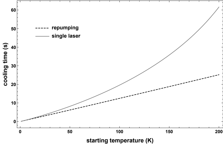
Figure 4.4: 1-D cooling times for \text{La}^- anions aiming to a final temperature of 0.17 \mu\text{K} (Doppler limit). The curve single laser assumes no repumping on the dark state ^3\text{F}_3^e state while the curve repumping assumes that no anion is lost due to the presence of dark states.
