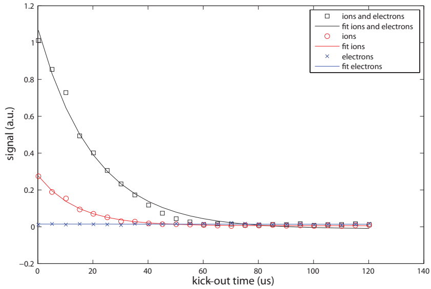
Figure 3.6: Number of anions remaining in the trap as a function of the release pulse time. The data show the presence of a heavy mass component in the trap. The experiment was repeated in the same conditions with electrons only, anions only and loading anions in a trap preloaded with electrons. The pulse time > 1 \mu\text{s} required for particles to escape indicates the presence of negative ions heavier than e^- (see Fig. 3.3). The signal is present only if the anion beam was guided through the trap. The exponential fit (solid lines) yields a storage time of 14.0(4) \mu\text{s} . Adapted from [91].
