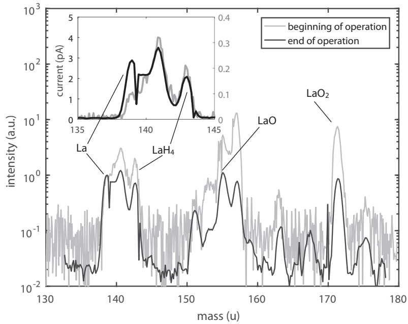
Figure 1.4: Mass spectra registered with a metallic La target. The curve beginning of operation was measured a few minutes after sputtering was started and the data at named end of operation after 2 days of continuous sputtering. The different noise levels have to be attributed to different data acquisition statistics. In the main figure the spectra normalized to the La peak to appreciate the ratio in the contaminants. Inset: The close view of the mass region of La in linear scale. The left scale refers to beginning of operation and right scale to end of operation .
