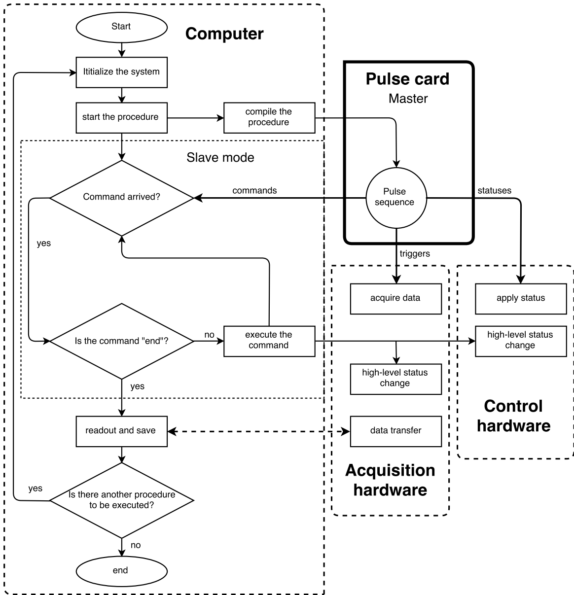
Figure 1.8: Flow chart of the execution of experimental procedures.
