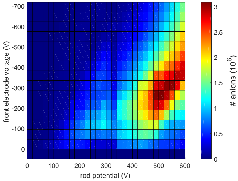
Figure 3.15: Trapping efficiency as function of storage and front potentials. The storage voltage was referenced to the beam kinetic energy. Anions were loaded for 20 s with with V_{pp} = 1.55 kV, the back voltage was -900 V relative to the rods' voltage.
