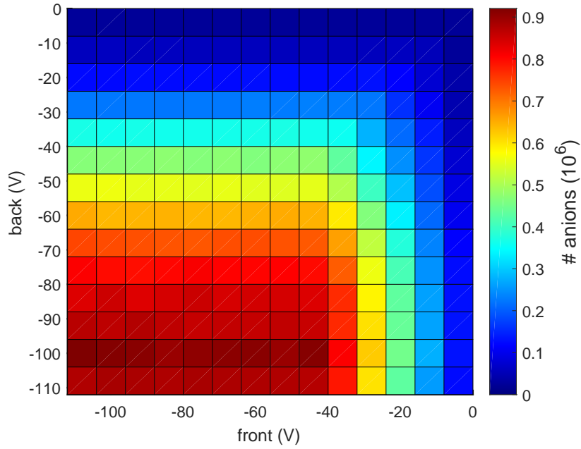
Figure 3.13: Trapping efficiency as a function of front and back potentials. During the experiment the center potentials was -795 V and the loading time 10 s. Front and back potentials are relative to the central voltage. The asymmetry in the measurement indicates that a back potential more confining than the front one leads to a higher trapping efficiency.
