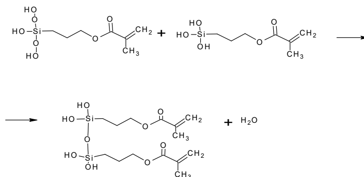
Figure 1. Reactions leading to spontaneous formation of O/W Pickering emulsions in the water/TPM + DCOIT system.
