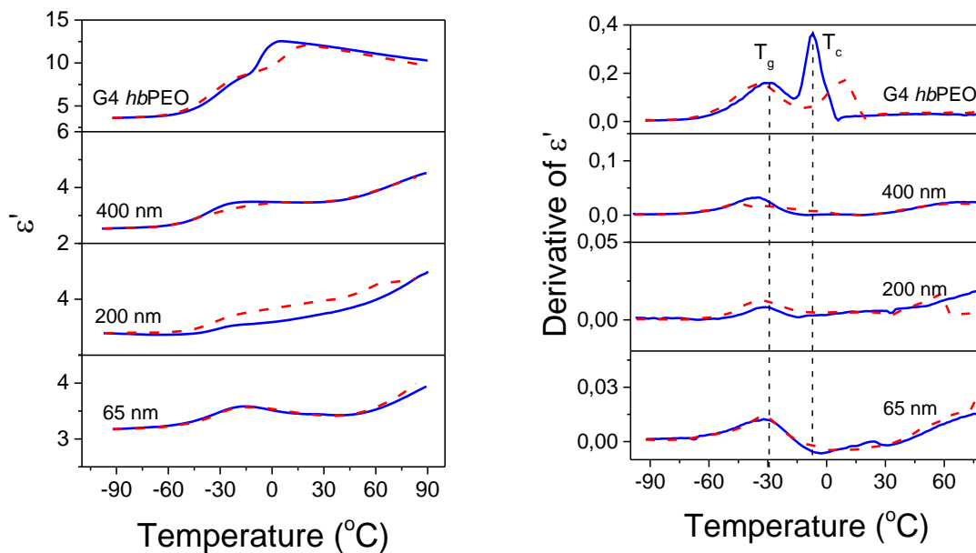
Figure S4. (Left) Temperature dependence of the dielectric permittivity of G4 hbPEO located within AAO with different pore diameters obtained on cooling (blue curves) and subsequent heating (red curves) with a rate of 5 °C/min. (Right) Derivative of dielectric permittivity, |\text{d}\epsilon'/\text{d}T| , as a function of temperature for the data shown in the left.
