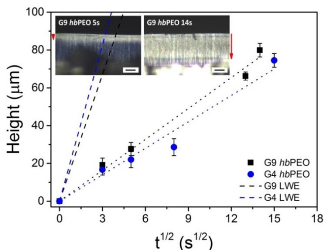
Figure 27. Imbibition length, h , as a function of t^{1/2} for G4 hbPEO and G9 hbPEO within self-ordered AAOs with a pore diameter of 65 nm. Dashed lines give the predictions of the LWE equation. Dotted lines are the results of a linear fit to the experimental data. The inset shows reflection microscopy images of G9 hbPEO located inside 65 nm AAO infiltrated for 5 s (left) and for 14 s (right) (scale bar is 20 \mu\text{m} ). Vertical arrows indicate respective imbibition lengths.
