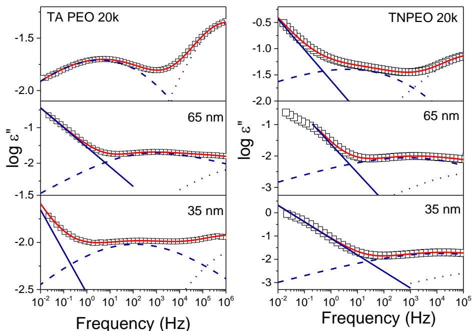
Figure S2. Comparison of dielectric loss spectra of bulk and confined TAPEO 20 k within self-ordered AAOs with pore diameters of 65 nm and 35 nm at -45\text{ }^{\circ}\text{C} (left) and bulk and confined TNPEO 20k at -35\text{ }^{\circ}\text{C} (right) within the same AAOs. The solid red lines are fits to a sum of two HN functions and to the ionic conductivity. Dashed and dotted lines give the individual contributions from the segmental ( \alpha -) and local ( \beta -) processes, respectively.
