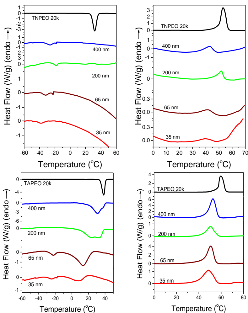
Figure. S8. Cooling (left) and heating (right) thermograms of TNPEO 20k (top) and of TAPEO 20k (bottom) located inside self-ordered AAO templates with different pore diameters (heating/cooling rates of 10°C/min).
