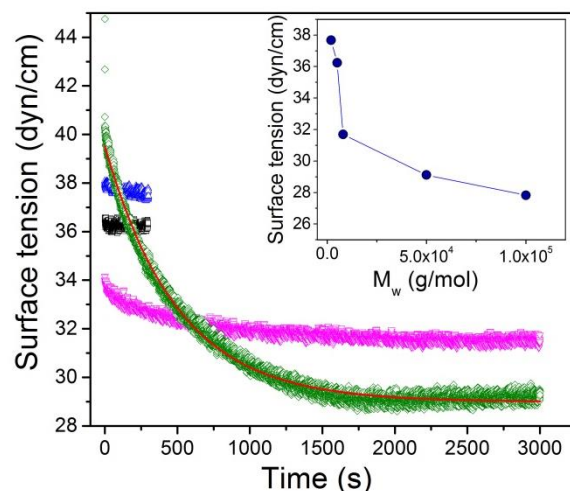
Figure 1. Surface tension as a function of time for different molecular weights of PEO all measured at 85 °C; (blue triangles): M_w=2\times 10^3 g/mol, (black squares): M_w=5\times 10^3 g/mol, (magenta down triangles): M_w=8\times 10^3 g/mol and (green rhombi): M_w=5.3\times 10^4 g/mol. The solid line is the result of a fit to an exponential function for the M_w=5.3\times 10^4 g/mol data. In the inset the equilibrium values of surface tension are plotted as a function of PEO molecular weight. The line is a guide for the eye.
