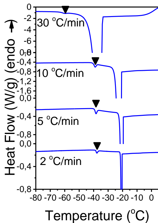
Figure S5. Differential scanning calorimetry traces of water/hollow silica spheres (diameter 341 nm) with different cooling rates as indicated.
