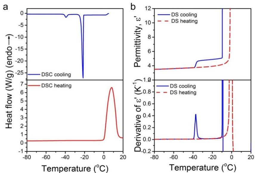
Figure 38. (a) DSC curves of water/hollow silica spheres with diameter of 533 nm obtained on cooling (top) and heating (bottom) with a rate of 10 °C/min. (b) Temperature dependence of the dielectric permittivity (top) and derivative of dielectric permittivity, d\epsilon'/dT , as a function of temperature of water/hollow silica spheres with diameter of 533 nm obtained on cooling and heating with a rate of 5 °C/min.
