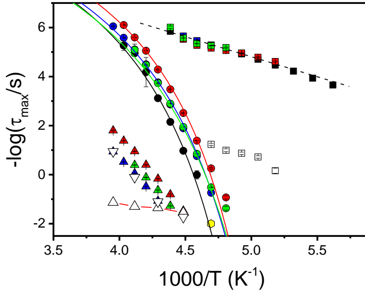
Figure S5. Relaxation times at maximum loss corresponding to the \alpha - (filled circles) and \beta - (filled squares) and MWS (filled triangles) processes of bulk G4 hbPEO (black symbols) and G4 hbPEO located inside self-ordered AAO pores with pore diameters; 400 nm (red), 200 nm (blue) and 65 nm (green). Solid and dashed lines are fits to the VFT and Arrhenius equations, respectively. The yellow hexagon is the bulk T_g (obtained from DSC). MWS model predictions based on a two-layer model where the layers are connected in parallel (series) are shown by the open right (inverted) triangles (data applicable to 65 nm pores).
