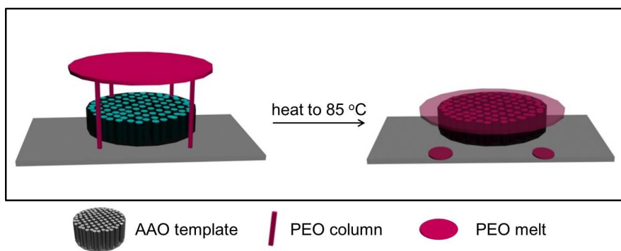
Figure S2. Schematic of the infiltration method.
