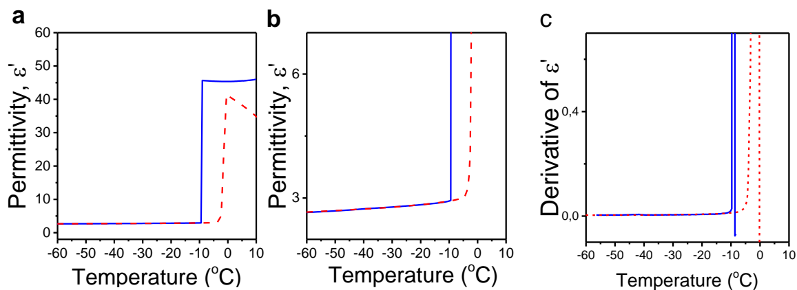
Figure S3. (a) Temperature dependence of the dielectric permittivity of water/polystyrene-silica core-shell particles (CS-261) with a diameter of 261 nm obtained on cooling (blue curves) and subsequent heating (red curves) with a rate of 5 °C/min. (b) Magnification of (a) in the region of low permittivity. (c) Derivative of dielectric permittivity, d\epsilon'/dT , as a function of temperature for the data shown in (a). In all cases the frequency is 1 MHz.
