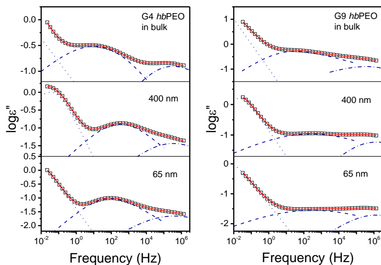
Figure 7. Comparison of dielectric loss spectra of bulk and of hyperbranched PEOs located within self-ordered AAOs with pore diameters of 400 nm and 65 nm at -50\text{ }^{\circ}\text{C} for G4 hbPEO (left) and for G9 hbPEO (right). In the bulk the solid red lines are fits to a summation of two HN functions and a conductivity contribution, whereas under confinement to a summation of three HN functions. The dashed and dashed-dotted lines give the contributions of the segmental ( \alpha -) and local ( \beta -) processes, respectively.
