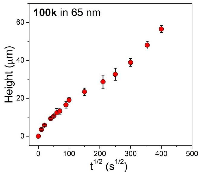
Figure S4. Imbibition length h , as a function of t^{1/2} for PEO 100k within self-ordered AAOs with pore diameter of 65 nm.
