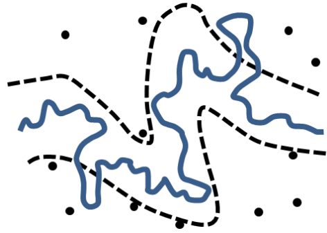
Figure 19. Schematic of tube model for flexible linear polymer chain (reproduced from ref 40 )
