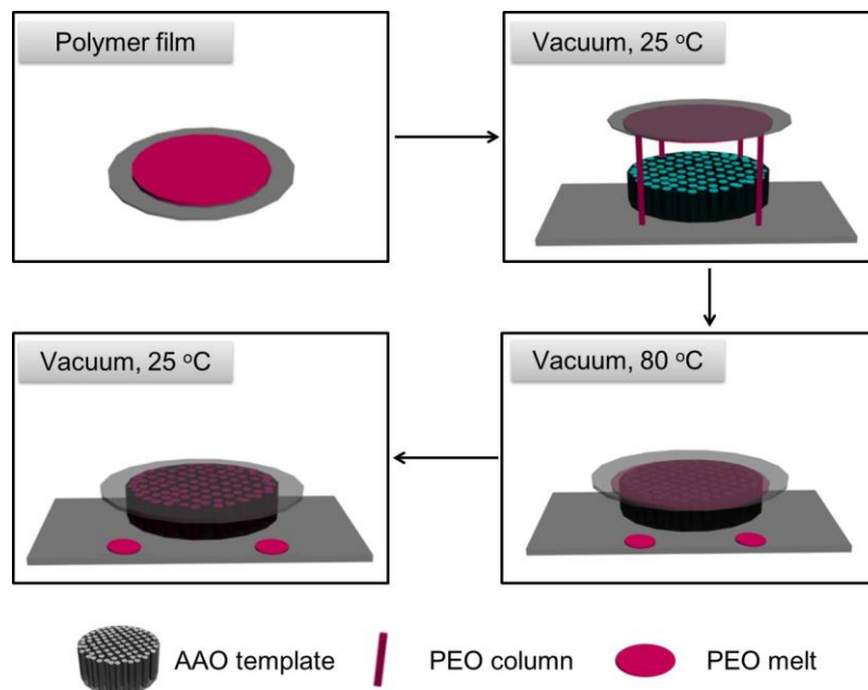
Figure 1. Schematic of the infiltration method under vacuum for bulk PEO.
