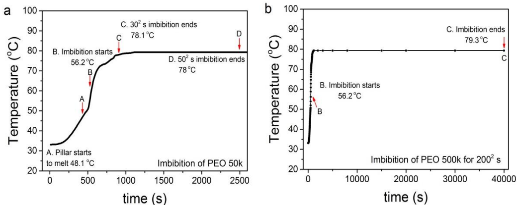
Figure A3. Temperature as a function of heating time during (a) the imbibition of PEO 50k for 30 2 s, 50 2 s and (b) imbibition of PEO 500k for 200 2 s.
