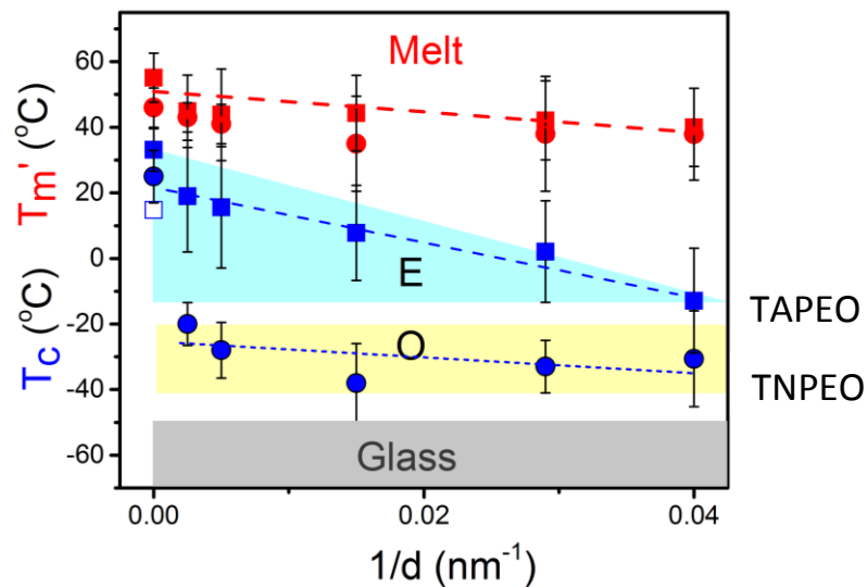
Figure 25. Apparent melting (red symbols) and crystallization temperatures (blue symbols) of TAPEO 10k (squares) and TNPEO 10k (circles) located inside AAO as a function of inverse pore diameter. The vertical bars do not indicate uncertainties but the temperature range corresponding to each crystallization/melting peak. Lines represent linear fits. Shaded areas indicate the (approximate) regions of heterogeneous nucleation (E), homogeneous nucleation (O) and glassy states.
