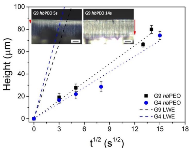
Figure 4. Imbibition length, h , as a function of t^{1/2} for G4 hbPEO and G9 hbPEO within self-ordered AAOs with a pore diameter of 65 nm. Dashed lines give the predictions of the LWE equation. Solid lines are the results of a linear fit to the experimental data. The inset shows reflection microscopy images of G9 hbPEO located inside 65 nm AAO infiltrated for 5 s (left) and for 14 s (right) (scale bar is 20 \mu\text{m} ). Vertical arrows indicate respective imbibition lengths.
