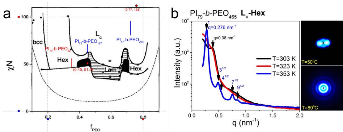
Figure 30. (a) Phase diagram of PI- b -PEO copied from ref 72 . The phase notation is as follows: L_c , crystalline lamellar, Lam, amorphous lamellar, Hex, hexagonal packed cylinders. The values of \chi N were obtained by using \chi = 65/T + 0.125 . (b) (left) SAXS spectra for PI 79 - b -PEO 465 shown at different temperatures. Arrows indicate positions of the main and higher order peaks. (right) 2D SAXS patterns obtained at 50 °C (top) and 80 °C (bottom).
