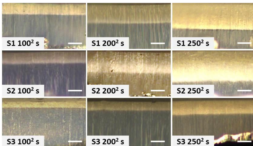
Figure 5. Reflection microscope images of PEO mixtures located inside 65 nm AAO infiltrated for different times: (top) S1 (PEO 50k/PEO 500k = 75/25); (middle) S2 (50k/500k = 50/50); (bottom): S3 (50k/500k = 25/75). Scale bar indicates 20 \mu m (Times are shown as 100^2 s, 200^2 s, 250^2 s that correspond to approximately 2.8 h, 11.1 h, 17.4 h, respectively.)
