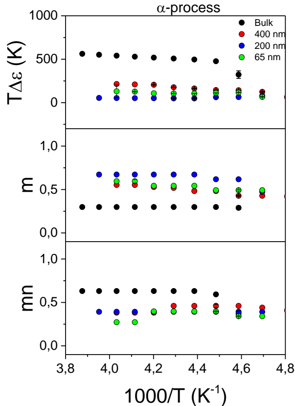
Figure S6. Summary of the Havriiliak-Negami fitting parameters obtained for the \alpha -process of G4 hbPEO .
