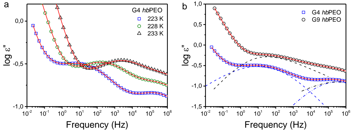
Figure 3. Dielectric loss curves of G4 hbPEO (a) at some temperatures as indicated. (b) Comparison of the dielectric loss curves for G9 hbPEO and G4 hbPEO at -50 °C. The solid red lines are fits according to a summation of two HN functions and a slower contribution. The dashed and dashed-dotted lines give the segmental ( \alpha -) and local ( \beta -) processes, respectively.
