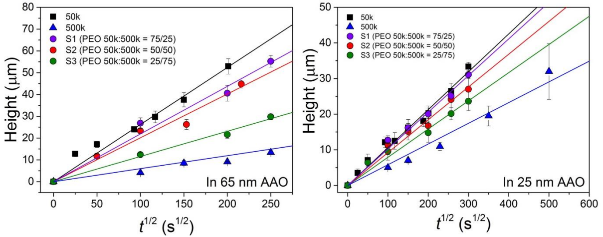
Figure 14. Imbibition length, h , as a function of t^{1/2} for two PEO homopolymers with molecular weights of 50k (squares) with 500k (triangles) and their mixtures with compositions: 50/50 (red spheres), 75/25 (magenta spheres), and 25/75 (green spheres) located inside AAO with pore diameters of (left) 65 nm and (right) 25 nm. Lines represent the result of a linear fit to the homopolymers and their mixtures.
