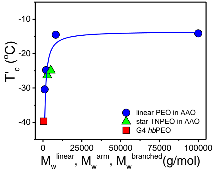
Figure 10. Dependence of the crystallization temperature T'_c initiated by homogeneous nucleation on the molecular weight of PEO in the limit d \rightarrow \infty ( d = AAO pore diameter). Spheres: the T'_c(d) profiles were obtained from DSC scans of linear PEO inside AAO at a cooling rate of 10 K/min. Triangles: star-shaped PEOs (in the limit d \rightarrow \infty ) obtained from DSC at a cooling rate of 10 K/min. Square: current studied G4 hb PEO (in the limit d \rightarrow \infty ) obtained from DSC at a cooling rate of 2 °C/min. The solid line is a fit using the Fox–Flory equation for linear PEOs located within self-ordered AAO templates.
