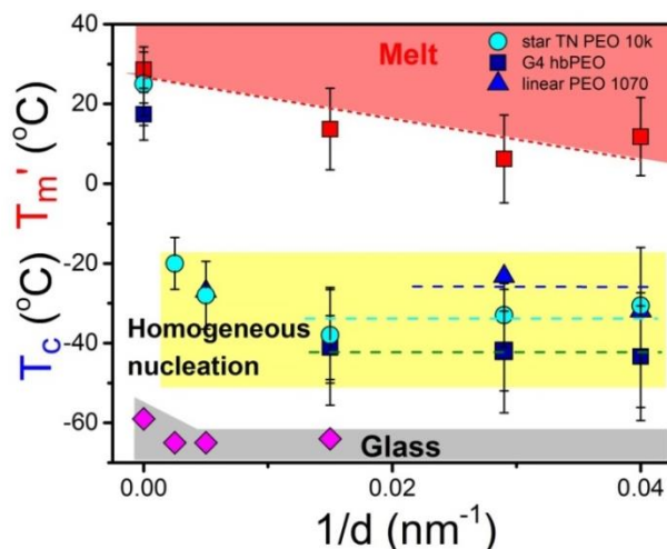
Figure 28. Apparent melting (red symbols) and crystallization temperatures (blue symbols) of star PEO 10000 g/mol (circles), G4 hbPEO (squares), and linear PEO (with molecular weight of 1070 g/mol) (triangles) located inside AAO as a function of inverse pore diameter. Glass temperatures from DS are shown with rhombi. The vertical bars indicate the temperature range corresponding to each crystallization/melting peak. Shaded areas indicate the (approximate) regions of melt state (red), homogeneous nucleation (yellow), and glass state (grey). Dashed lines are guides to the eye.
