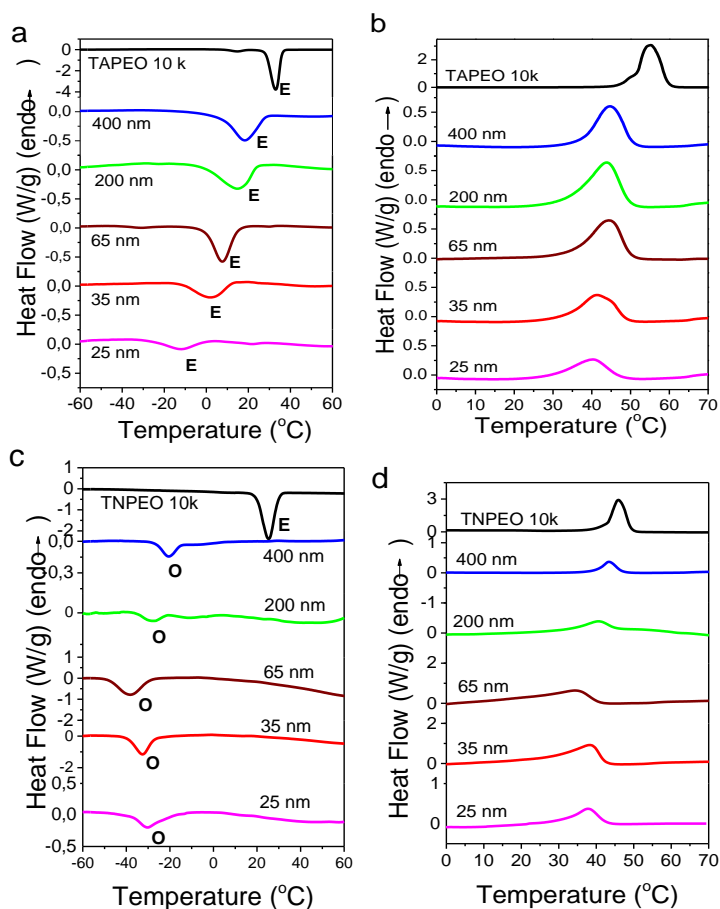
Figure 8. Cooling (left) and heating (right) thermograms of TAPEO 10k (a,b) and of TNPEO 10k (c,d) located inside self-ordered AAO with pore diameters ranging from 400 nm to 25 nm (heating/cooling rates of 10 °C/min). The letters, E and O, in (a) and (c) represent crystallization via heterogeneous and homogeneous nucleation, respectively.
