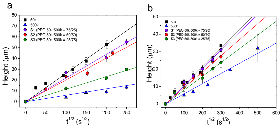
Figure 6. Imbibition length h , as a function of t^{1/2} for two PEO homopolymers with molecular weights of 50k (squares) with 500k (triangles) and their mixtures with compositions: 50/50 (red spheres), 75/25 (magenta spheres) and 25/75 (green spheres) located inside AAO with pore diameters of (a) 65 nm and (b) 25 nm. Lines represent the result of a linear fit to the homopolymers and their mixtures.
