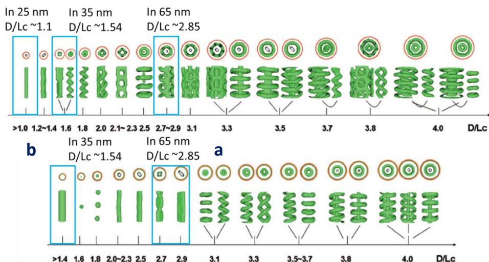
Figure 32. Self-assembled morphologies for asymmetric diblock copolymers with f_A=1/4 as a function of D/L_C . Only the A blocks are shown. The outermost red circle in each top view indicates the surface of the cylindrical pore. (top) \alpha=-1.0 and (bottom) \alpha=1.0 . Figure reproduced from ref 71 .
