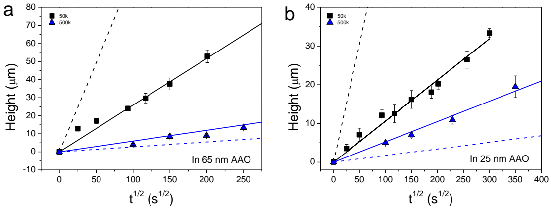
Figure 4. Imbibition heights as a function of t^{1/2} for the PEO homopolymers. Dashed lines give the predictions of the theoretical LWE for the PEO 50 k (black) and PEO 500k (blue) within AAO templates with diameters of 65 nm (a) and 25 nm (b). Note the slower (faster) imbibition for the shorter (longer) chains as compared to the theoretical predictions by the LWE.
