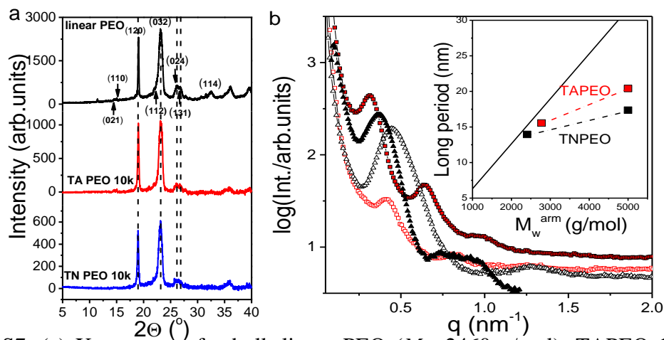
Figure. S7. (a) X-ray scans for bulk linear PEO ( M_w=2460 g/mol), TAPEO 10k and TNPEO 10k at ambient temperature. Arrows give the position and (hkl) indices of the Bragg reflections corresponding to the monoclinic unit cell of PEO. (b) SAXS patterns of bulk TAPEO 10k (open squares), TAPEO 20k (filled squares), TNPEO 10k (open triangles), and TNPEO 20k (filled triangles) at 30 °C. In the inset the long period is plotted as a function of arm molecular weight for the TAPEO (red symbols) and TNPEO (black symbols). Dashed lines are guides for the eye. The solid line gives the long period for an extended chain crystal. 4
