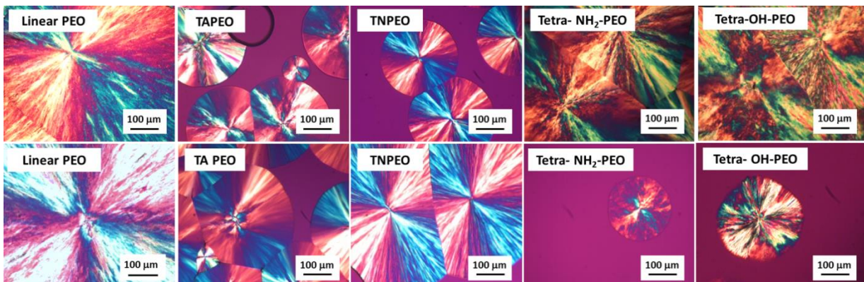
Figure S3 depicts POM images of linear PEO (with molecular weight of 2460 g/mol), TAPEO 10k and TNPEO 10k as well as star-shaped PEOs of tetra- \text{NH}_2 -PEO ( M_w=20\text{k} ), and tetra-OH-PEO ( M_w=20\text{k} ) compared after the same isochronal cooling with rate of (top) and under conditions of same degree of undercooling (bottom).
