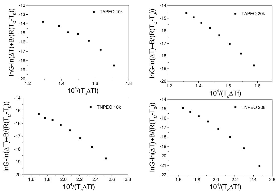
Figure. S6. Spherulitic growth rates for TAPEO 10k, TAPEO 20k, TNPEO 10k, and TNPEO 20k as a function of reduced temperature. The values of B and T_{inf} used LH theory are taken from DS fitting (as shown in Table S1).
