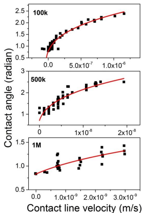
Figure S5. Dynamic contact angles for the three PEO polymers. Lines give the result of the fits according to the Cox equation.
