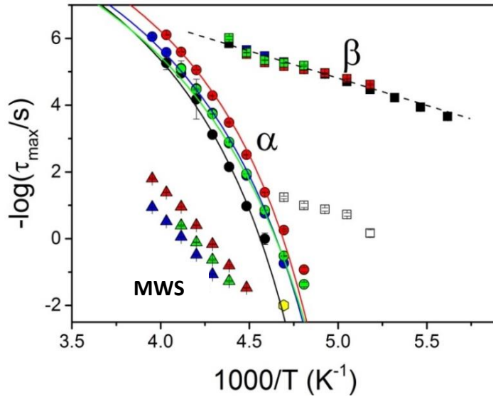
Figure 29. Relaxation times at maximum loss corresponding to the \alpha - (filled circles) and \beta - (filled squares) and MWS (filled triangles) processes of bulk G4 hb PEO (black symbols) and G4 hb PEO located inside self-ordered AAO pores with pore diameters; 400 nm (red), 200 nm (blue) and 65 nm (green). Solid and dashed lines are fits to the VFT and Arrhenius equations, respectively. Open squares show the contribution of a small amount of water in the bulk sample. The yellow hexagon is the bulk T_g (obtained from DSC).
