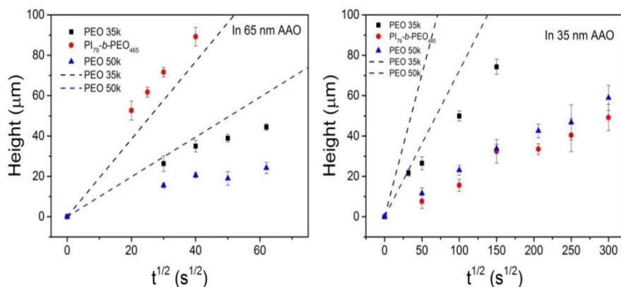
Figure 31. Imbibition length, h , as a function of t^{1/2} for PI 79 - b -PEO 465 within self-ordered AAOs with a pore diameter of 65 nm (left) and 35 nm (right). Dashed lines give the predictions of the LWE equation for linear PEO 35k and 50k, respectively.
