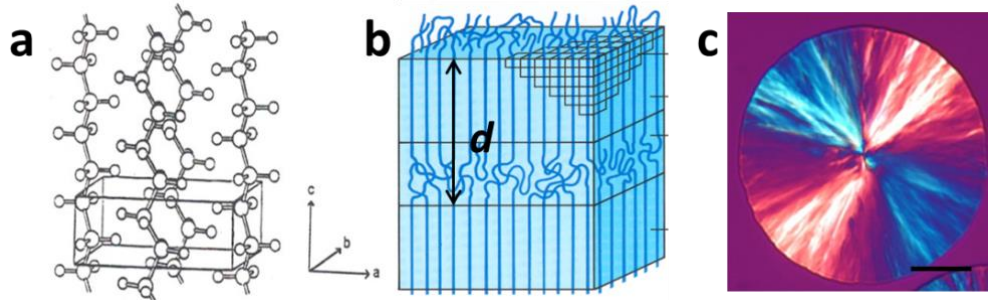
Figure 16. a. Unit cell of PE crystallites: Orthorhombic symmetry, a = 7.42 \text{ \AA} , b = 4.95 \text{ \AA} , c = 2.55 \text{ \AA} . Structure determination by Bunn 28 b. Schematic of lamellar crystals with the long period, d . c. POM image of a spherulite corresponding to a star PEO. The scale bar indicates 50 \mu\text{m} .
