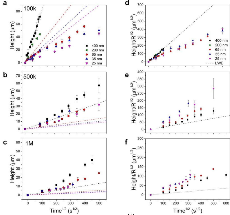
Figure 4. Imbibition length h , as a function of t^{1/2} for (a) PEO 100k, (b) PEO 500k and (c) PEO 1M within self-ordered AAOs with different pore diameters; (squares) 400 nm, (left triangles): 200 nm, (spheres): 65 nm, (up triangles): 35 nm and (down triangles): 25 nm. The respective data normalized to the pore radii are shown in the right (d, e, f). Dashed lines give the predictions of the LWE equation.
