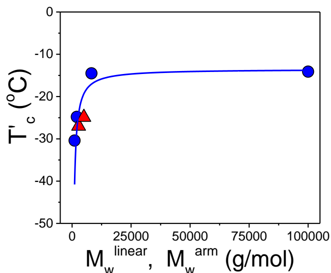
Figure 11. Dependence of the crystallization temperature T'_c of crystallization processes initiated by homogeneous nucleation on the molecular weight of PEO in the limit d \rightarrow \infty ( d = \text{AAO pore diameter} ). (Spheres): The T'_c(d) profiles were obtained from DSC scans of linear PEO inside AAO at a cooling rate of 10^\circ\text{C}/\text{min} . (triangles): current investigation of star-shaped TNPEOs (in the limit d \rightarrow \infty ) obtained from DSC at a cooling rate of 10^\circ\text{C}/\text{min} . The solid line is a fit using the Fox-Flory equation for linear PEOs located within self-ordered AAO templates.
