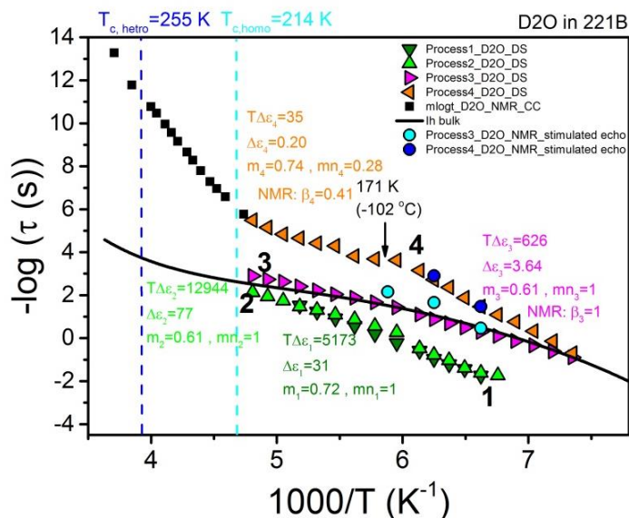
Figure 43. Relaxation times for different processes obtained from fitting DS spectra for D 2 O confined in 221B, compared with those obtained from NMR T_1 measurement, fitted with Cole-Cole function (filled squares), and stimulated echo. Solid line shows the relaxation of bulk ice 102 . The vertical dash lines show the crystallization temperature of D 2 O via heterogeneous and homogeneous nucleation, respectively.
