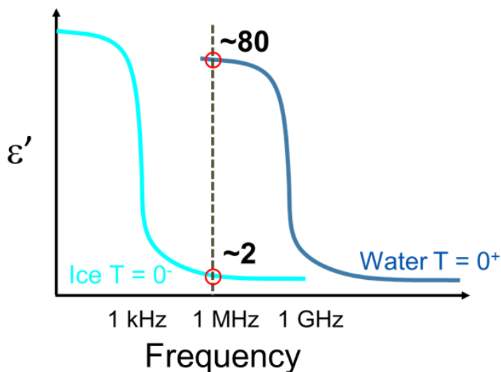
Figure 39. Schematic of permittivity of water and ice as a function of frequency at temperatures around freezing ( T=0^+ , T=0^- ). The vertical line indicates the frequency used in the isochronal measurement (1 MHz).
