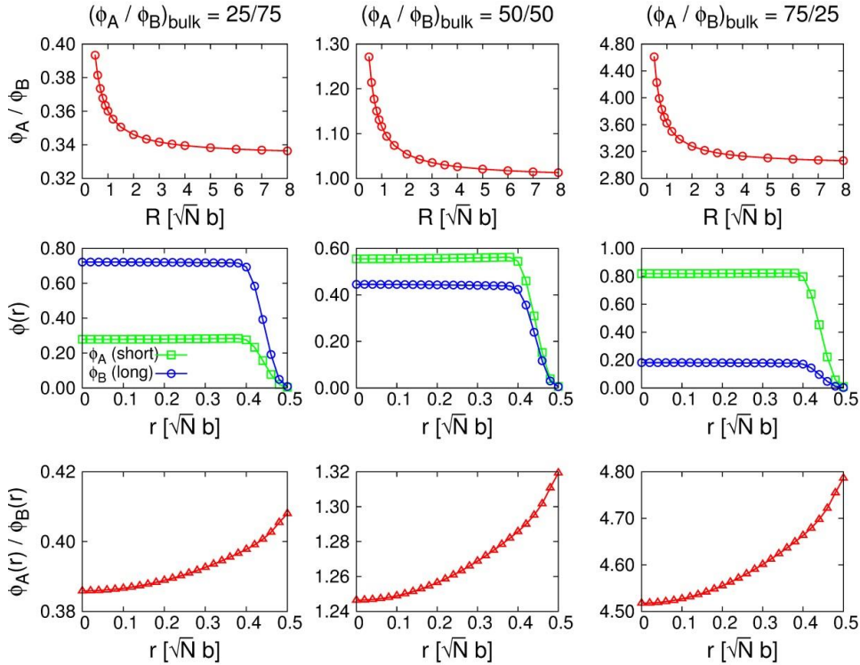
Figure 8. Self-consistent field theory calculations for three blend compositions; (left column) \varphi_A = 0.25 , \varphi_B = 0.75 , (middle) \varphi_A = \varphi_B = 0.50 and (right column) \varphi_A = 0.75 , \varphi_B = 0.25 . The results of the averaged \varphi_A/\varphi_B is shown in the first row as a function of the cylinder radius R (in units of b\sqrt{N} ). The spatial distribution of the polymers as a function of r , the distance to the pore axis is shown in the second row. The local density ratio of short to long chains is plotted in the third row.
