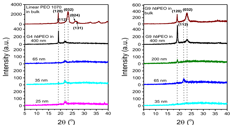
Figure 5. \theta - 2\theta scans for G4 hb PEO and G9 hb PEO confined within AAO with different pore diameters as indicated all measured at -50 °C (e.g. below the crystallization temperature). Dashed lines give the position and (hkl) indices of the main Bragg reflections corresponding to the monoclinic unit cell of PEO.
