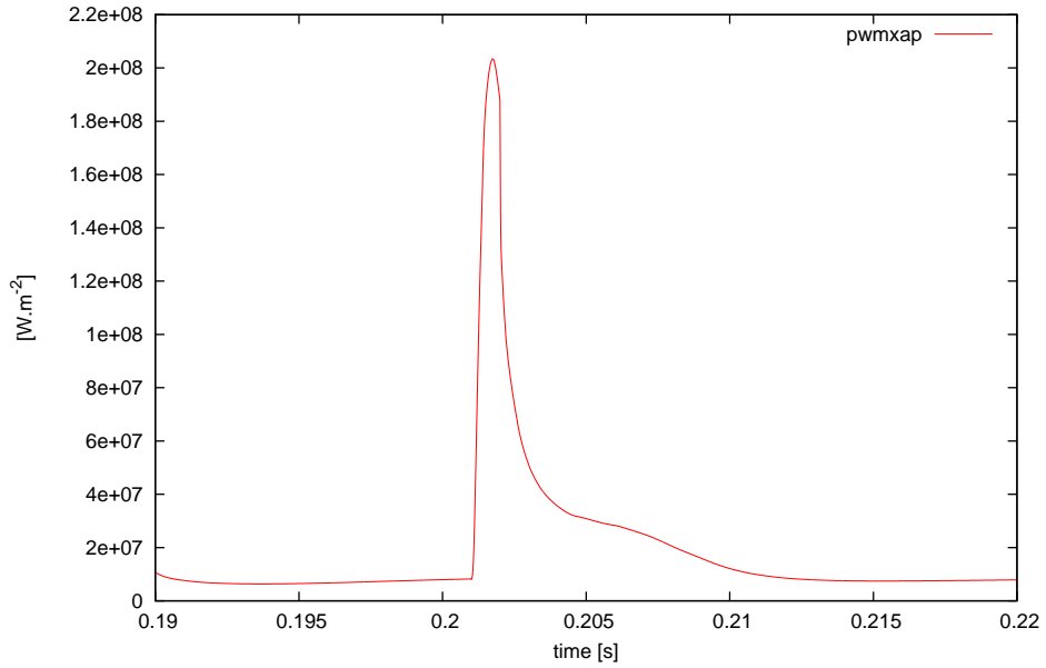
(b) The maximum total power flux on the 9 outer target for the same case as Fig.3a.
