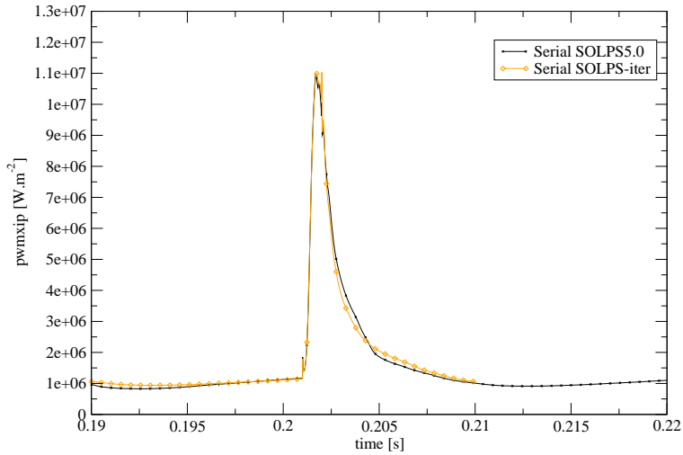
(a) The maximum total power flux on the inner target for an ELM cycle, obtained from SOLPS 5.0 and SOLPS-ITER. The normalized RMSE defined by eq.6 for these data sets is 1.557E-02.
