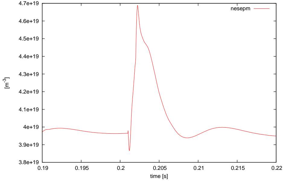
(a) The SOLPS5.0 calculated electron density ( n_{\text{esepm}} ) at the outer midplane separatrix shows a sudden rise followed by a reduction during the ELM cycle.
