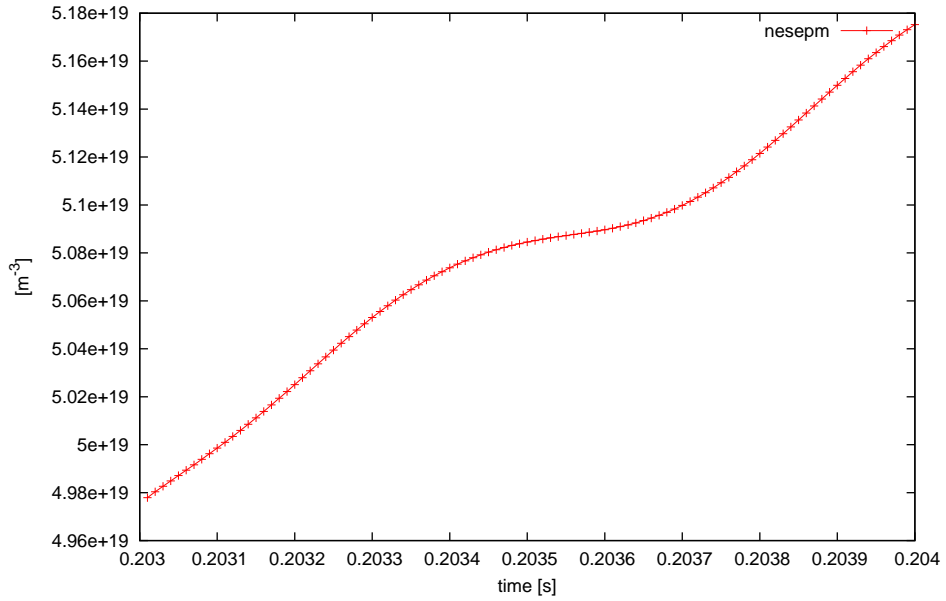
(b) At the parareal iteration k=2 , nesepm starts to increase affecting subsequent time chunks solved using the parareal algorithm eventually leading to the (wrong) solution shown in Fig.5b.
