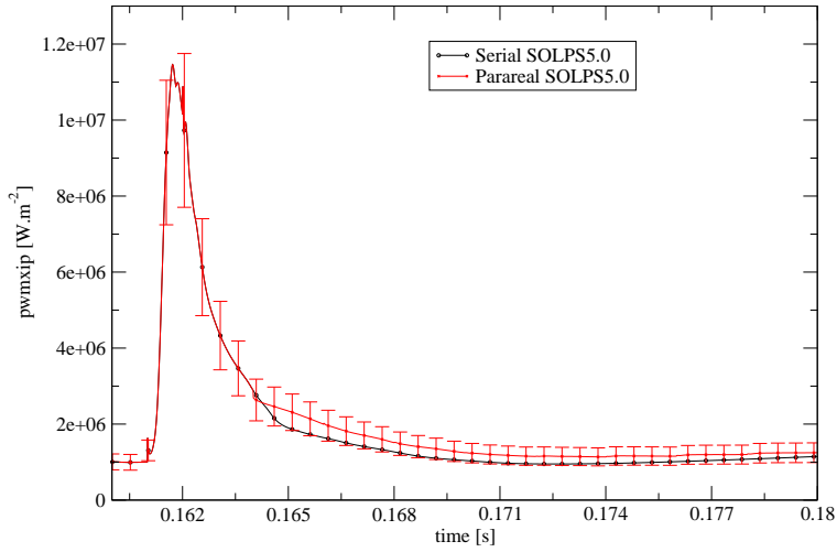
(a) The maximum total power flux on the inner target for an ELM cycle, obtained from SOLPS 5.0 and parareal. The normalized RMSE defined by eq.6 for these data sets is 1.95E-02.
