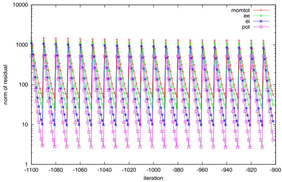
(b) The norm of the residuals for the equations as computed by the SOLPS code package for a converged case of the parareal formalism.
