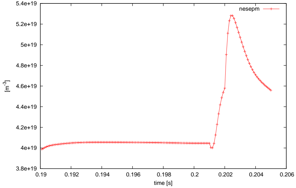
(a) nesepm from the coarse(G) computation at k=1 shows expected behaviour.
