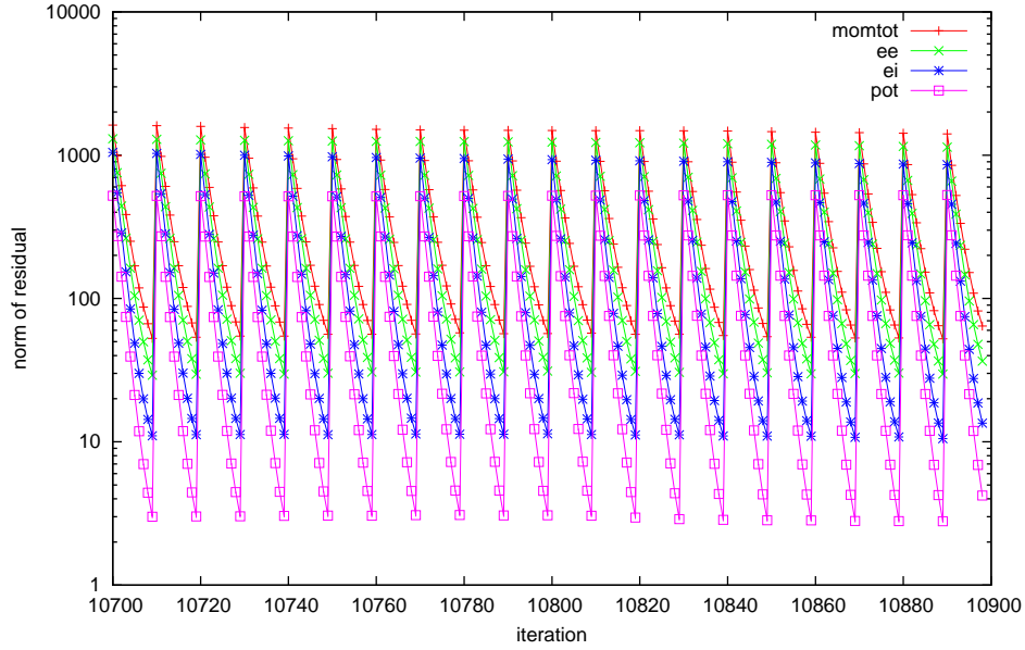
(a) The norm of the residuals for the equations as computed by the SOLPS code package for a serial or fine (F) simulation.
