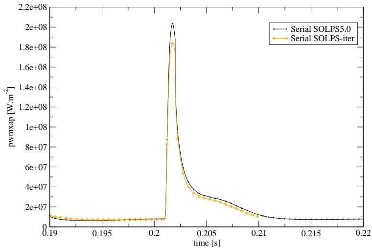
(b) The maximum total power flux on the outer target for the same case as Fig.11a. The normalized RMSE for these data sets is 2.0203E-02.
