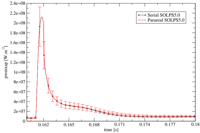
(b) The maximum total power flux on the outer target for the same case as Fig.12a. The normalized RMSE for these data sets is 6.43E-03.
