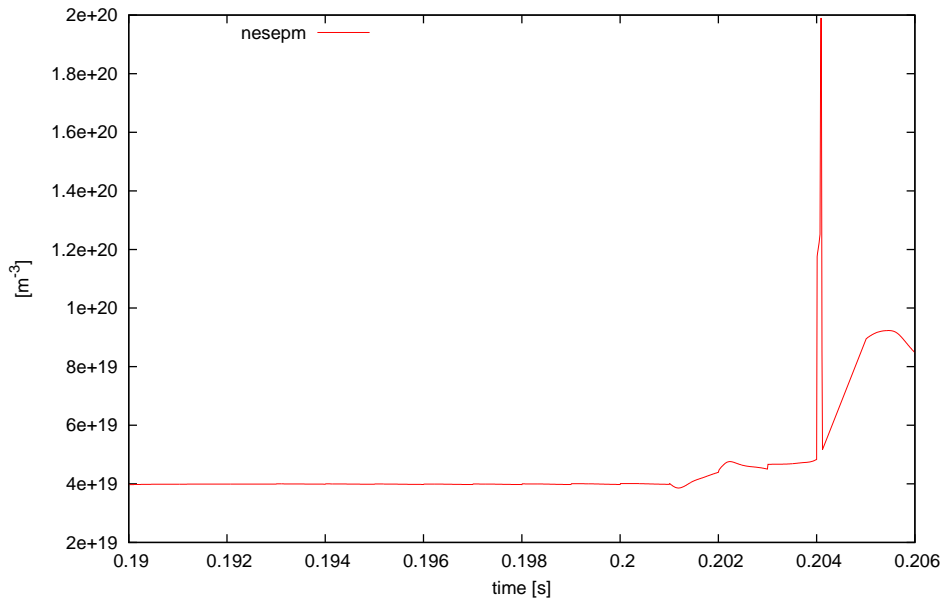
(b) nesepm from the parareal computation at k=3 shows anomalous behaviour.
