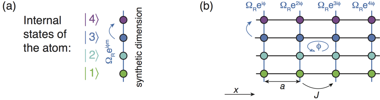
Figure 10. SYNTHETIC DIMENSIONS (a) Schematic illustration of a synthetic dimension, which consists of different internal states of an atom, here illustrated with different colors. Coupling between these states can be realized, for instance, with Raman beams, which are naturally complex \Omega_R e^{i\phi m} and whose phase depends on position, here labeled by the index m . (b) 2D synthetic lattice, where one dimension is a normal optical lattice in real space, where the sites are labeled by the index m and the second dimension is realized with internal states as in (a). This setting mimics an effective magnetic field with flux \alpha = \phi/(2\pi) .
