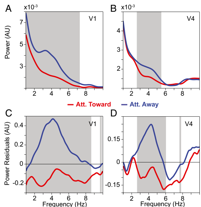
Fig. 3. Average low-frequency LFP power spectra and their modulation by selective attention. (A) Average LFP power spectra in area V1 with attention toward (red) and away (blue) from the activating stimulus. The gray-shaded region indicates frequencies with a significant difference between attention conditions ( P < 0.05 ; nonparametric permutation test with correction for multiple comparisons across frequencies). (B) Same as A, but for area V4. (C) Same as A, but showing the power residuals after removing the 1/f^n component of the power spectrum through robust regression (Methods). (D) Same as C, but for area V4. Att., attention; A.U., arbitrary units.
