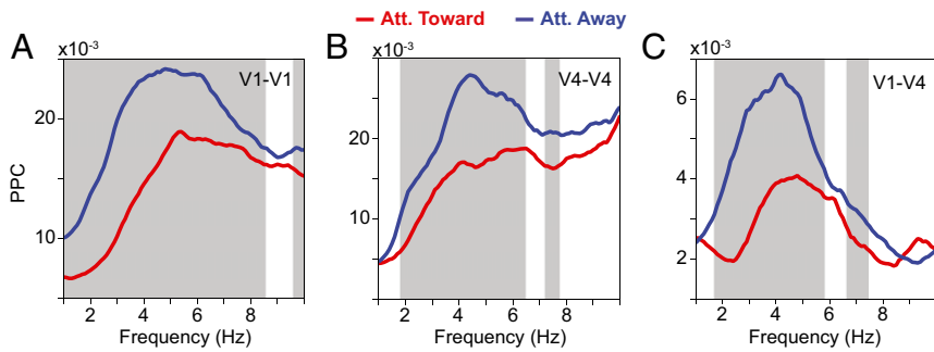
Fig. 4. Average low-frequency LFP phase-locking (PPC) spectra and their modulation by selective attention. (A) Average LFP phase locking between sites within area V1 with attention toward (red) and away from (blue) the activating stimulus. The gray-shaded region indicates frequencies with a significant difference between attention conditions ( P < 0.05 ; nonparametric permutation test with correction for multiple comparisons across frequencies). (B) Same as A, but between sites within area V4. (C) Same as A, but between sites in area V1 and sites in area V4. Att., attention.
