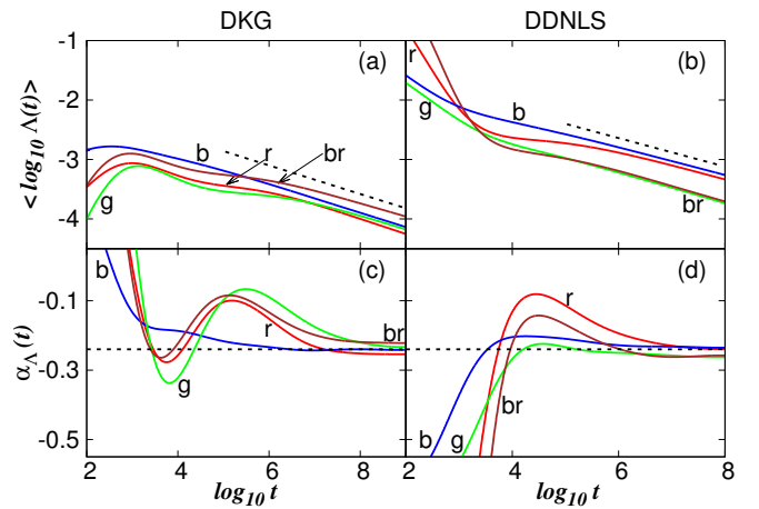
FIG. 2. (Color online) Weak chaos. Averaged (and smoothed) results over 100 disorder realizations of the time evolution of the finite-time mLE \Lambda(t) [(a), (b)] and the corresponding derivatives \alpha_\Lambda (10) [(c), (d)] for the DKG [(a), (c)] and the DDNLS [(b), (d)] systems. The straight dashed lines indicate slopes \alpha_\Lambda = -0.25 . The curve colors correspond to the cases presented in Fig. 1. All panels are in log-log scale.
