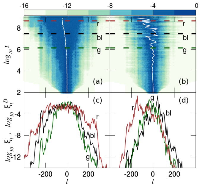
FIG. 5. (Color online) DKG model, weak chaos. The dynamics of a representative initial condition of the W1_K case for one disorder realization. Time evolution of (a) the normalized energy distribution \xi_l and (b) the corresponding DVD. The color scales at the top of the figure are used for coloring lattice sites according to their \log_{10} \xi_l (a) and \log_{10} \xi_l^D (b) values. In both panels a white curve traces the distributions' center. Normalized energy distributions \xi_l (c) and DVDs (d) at times \log_{10} t = 6.14 , \log_{10} t = 7.47 , \log_{10} t = 8.65 [green (g); black (bl); red (r)]. These times are also denoted by similarly colored horizontal dashed lines in (a) and (b).
