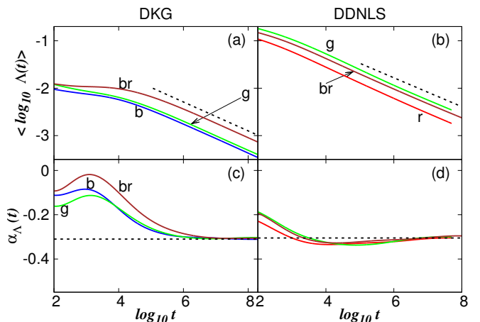
FIG. 4. (Color online) Strong chaos. Similar to Fig. 2. The straight dashed lines indicate slopes \alpha_\Lambda = -0.3 . The various curves correspond to the cases presented in Fig. 3.
