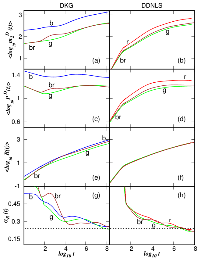
FIG. 10. (Color online) DVD characteristics in the strong chaos regime. Similar to Fig. 7, but for the strong chaos cases presented in Fig. 3. The horizontal dashed lines in (g) and (h) indicate the slope \alpha_R = 0.24 as in Figs. 7(g), (h).
