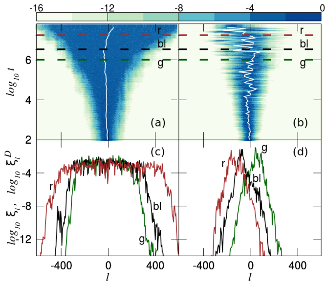
FIG. 9. (Color online) DDNLS model, strong chaos. Similar to Fig. 6, but for a representative initial condition of the S3_D case. The distribution snapshots in the lower panels are taken at times \log_{10} t = 6.01 , \log_{10} t = 6.54 , \log_{10} t = 7.24 [green (g); black (bl); red (r)].
