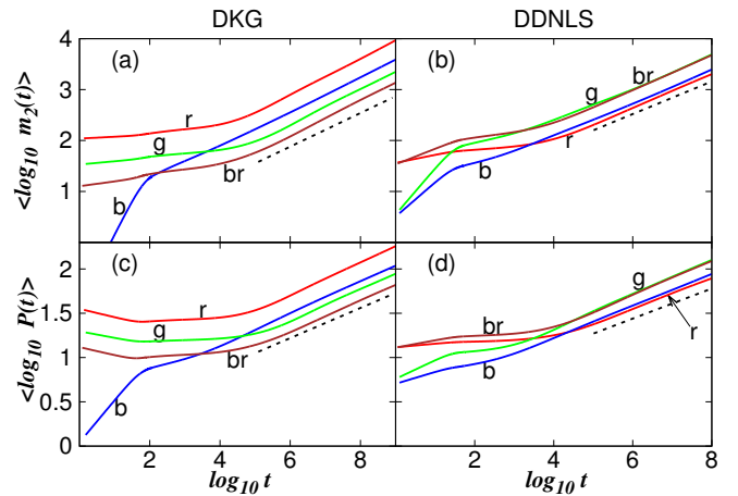
FIG. 1. (Color online) Weak chaos. Averaged (and smoothed) results over 100 disorder realizations of the time evolution of the wave packets' second moment m_2 [(a), (b)] and participation number P [(c), (d)] for the DKG [(a), (c)] and the DDNLS [(b), (d)] systems. The straight dashed lines guide the eye for slopes \frac{1}{3} [(a), (b)] and \frac{1}{6} [(c), (d)]. The presented cases are W1_K, W2_K, W3_K, W4_K [(r) red; (b) blue; (g) green; (br) brown] for the DKG system and W1_D, W2_D, W3_D, W4_D [(br) brown; (g) green; (b) blue; (r) red] for the DDNLS model. All panels are in log-log scale.
