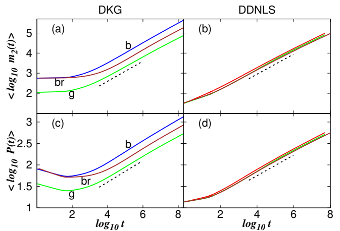
FIG. 3. (Color online) Strong chaos. Similar to Fig. 1. The straight dashed lines guide the eye for slopes \frac{1}{2} [(a), (b)] and \frac{1}{4} [(c), (d)]. The presented cases are S1_K, S2_K, S3_K [(b) blue; (g) green; (br) brown] for the DKG system [(a), (c)] and S1_D, S2_D, S3_D [(g) green; (r) red; (br) brown] for the DDNLS model [(b), (d)].
