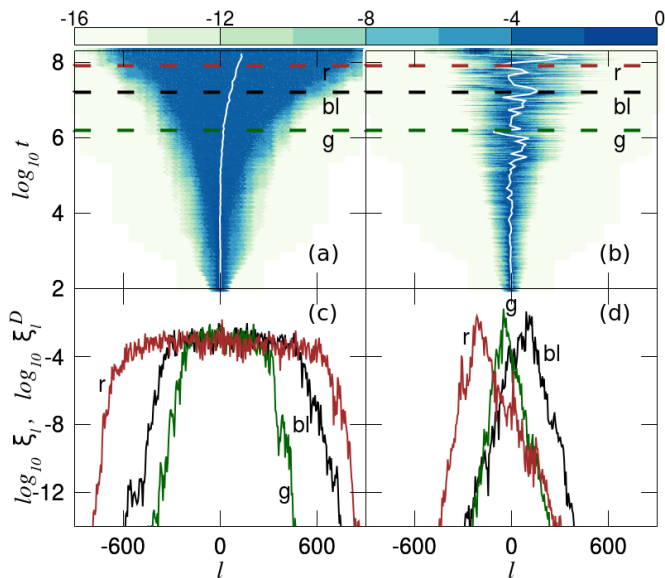
FIG. 8. (Color online) DKG model, strong chaos. Similar to Fig. 5, but for a representative initial condition of the S3_K case. The distribution snapshots in the lower panels are taken at times \log_{10} t = 6.2 , \log_{10} t = 7.2 , \log_{10} t = 7.9 [green (g); black (bl); red (r)].
