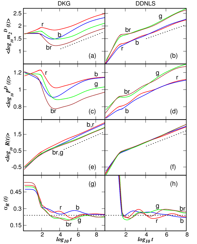
FIG. 7. (Color online) DVD characteristics in the weak chaos regime. Time evolution of the averaged (and smoothed) over 100 disorder realizations, second moment m_2^D [(a), (b)], participation number P^D [(c), (d)] and R (12) [(e), (f)]. The numerically computed derivatives \alpha_R (10) of curves in (e) and (f) are respectively plotted in (g) and (h). Left panels contain results for the DKG model with curve colors corresponding to the cases presented in the left panels of Fig. 1. Results for the DDNLS model are presented in the right panels with curve colors corresponding to the cases considered in the right panels of Fig. 1. The straight dashed lines in (a) and (b) correspond to slope 0.14, while in (e)-(h) indicate the slope \alpha_R = 0.24 . All horizontal axes are logarithmic. Panels (a)-(f) are in log-log scale.
