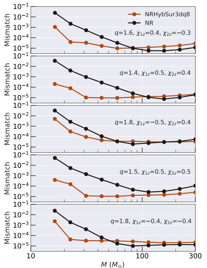
FIG. 8. Comparisons between the NRHybSur3dq8 surrogate model and a few NR waveforms of \sim 10^5 M in duration. We also show the NR resolution error. 95 th -percentile mismatches (over points in the sky) are shown as a function of total mass. The inset text indicates the mass ratio and component spins. Mismatches are computed using the Advanced LIGO design sensitivity noise curve. To best assess the error introduced by the hybridization procedure we use the same set of modes for the NR waveforms as the surrogate. At low masses, the hybridization errors (red circles) become less reliable measures of accuracy due to the large NR resolution error (black circles) itself. Fig. 9 describes a refined comparison to improve the assessment at low masses.
