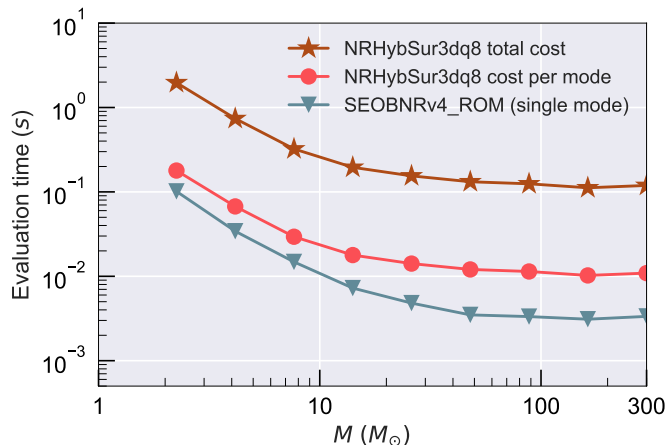
FIG. 12. Evaluation cost for NRHybSur3dq8 including the cost of a Fast Fourier Transform. We show the cost for evaluating all 11 modes modeled by NRHybSur3dq8, as well as the cost of a single mode. These are compared to the evaluation cost of SEOBNRv4_ROM which includes only the (2, 2) mode. The evaluation cost is computed by averaging over 64 points uniformly distributed in the parameter space, q \leq 8 and |\chi_{1z}|, |\chi_{2z}| \leq 0.8 .
