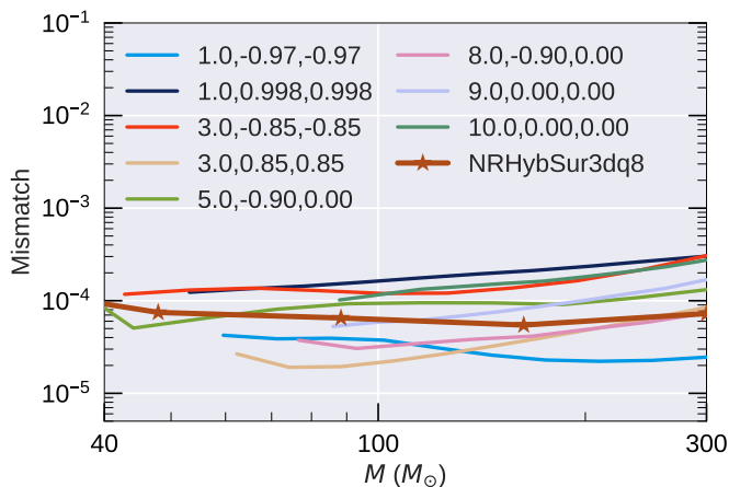
FIG. 10. Errors in NRHybSur3dq8 when evaluated outside its training range. 95 th -percentile mismatches (over points in the sky) are shown as a function of total mass for different extrapolated cases. These are computed using the Advanced LIGO design sensitivity noise curve. To best assess the error introduced by the extrapolation, we use the same set of modes for the NR waveforms as the surrogate. The labels indicate the mass ratio and component spins ( q, \chi_{1z}, \chi_{2z} ). For comparison we reproduce the 95 th -percentile mismatches for NRHybSur3dq8 within its training range from the right panel of Fig. 6.
