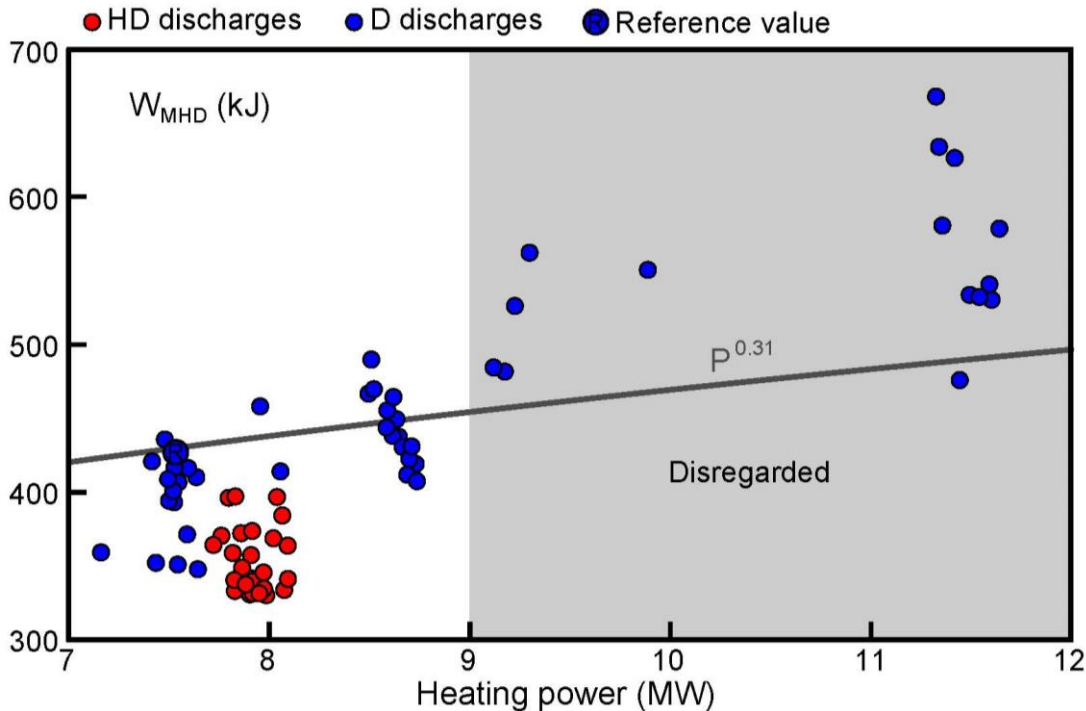
Figure 6: Plasma energy versus applied total heating power for the discharges with HD (red dots) and D (blue dots) pellet injection. Restricting the analysed data set to heating power
