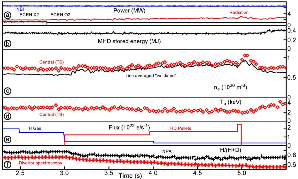
Figure 2: Overview of a typical plasma discharge testing the isotopic fraction control by H/D-pellet injection. In this case, a pure H gas puff is gradually replaced by HD-pellets. This results in a considerable decrease of the H fraction in the plasma. Due to the higher fuelling efficiency, both line-averaged and core density are increased by the pellets. The plasma stored energy remains unaffected while the temperature is decreased. The pellet sequence is concluded by a short phase with maximum pellet flux which generate a short high-density phase that reaches the Greenwald density in the plasma centre.
