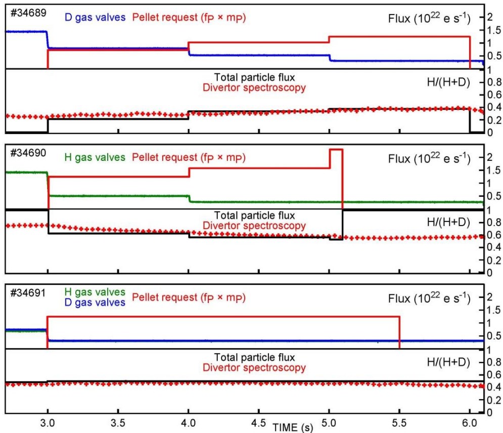
Figure 3: Adjusting the H/(H+D) isotope fraction by injection of H/D pellets replacing the initial strong gas puff in discharges with NBI H^0 injection. In case a pure D gas puff is replaced, the H content is increased; H gas puff replacement reduces the H content. For sufficiently strong particle fuelling, the isotopic fraction measured by divertor spectroscopy approaches quickly the total flux fraction.
