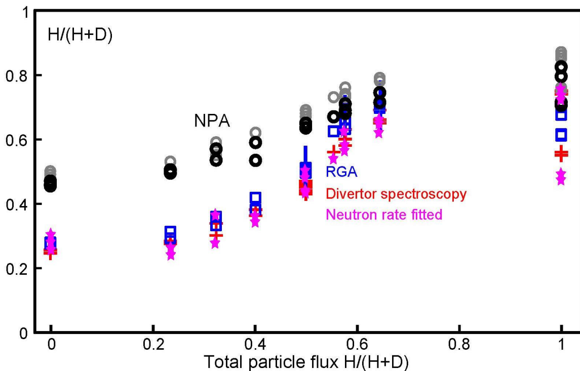
Figure 4: Directly measured H/(H+D) by the NPA (grey circles) and values calculated taking into account CX probabilities and attenuation (black circles) in comparison to edge diagnostics data. Added as well are data estimated from the neutron rate calibrated to fitted relation (*).
