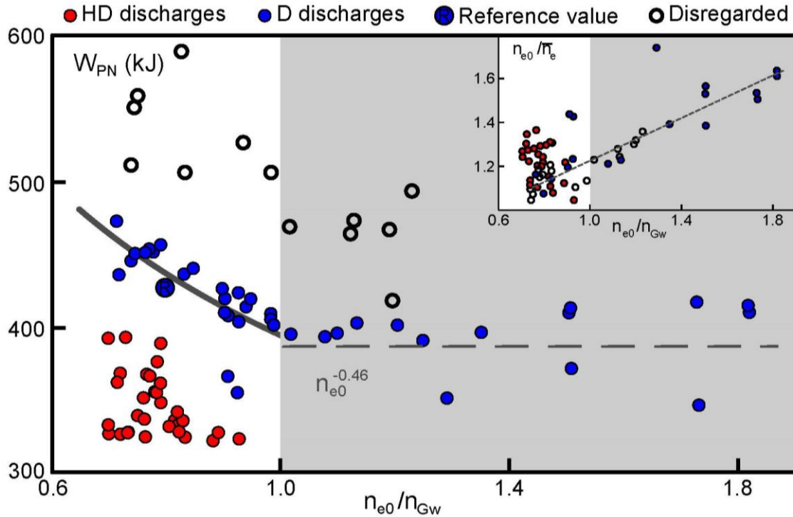
Figure 7: Stored MHD plasma energy normalized with respect to heating power versus core density normalized to the line-averaged Greenwald density formula. The solid line shows a fit to the pure D data from the reference discharges with heating power below 9 MW and core density below n_{Gw} ; the dashed line fits the mean value of W_{PN} above n_{Gw} . The inset shows the peaking factor n_e^0/\bar{n}_e , the dashed line indicated that the peaking factor increases with the normalised core density for the pure D plasmas.
