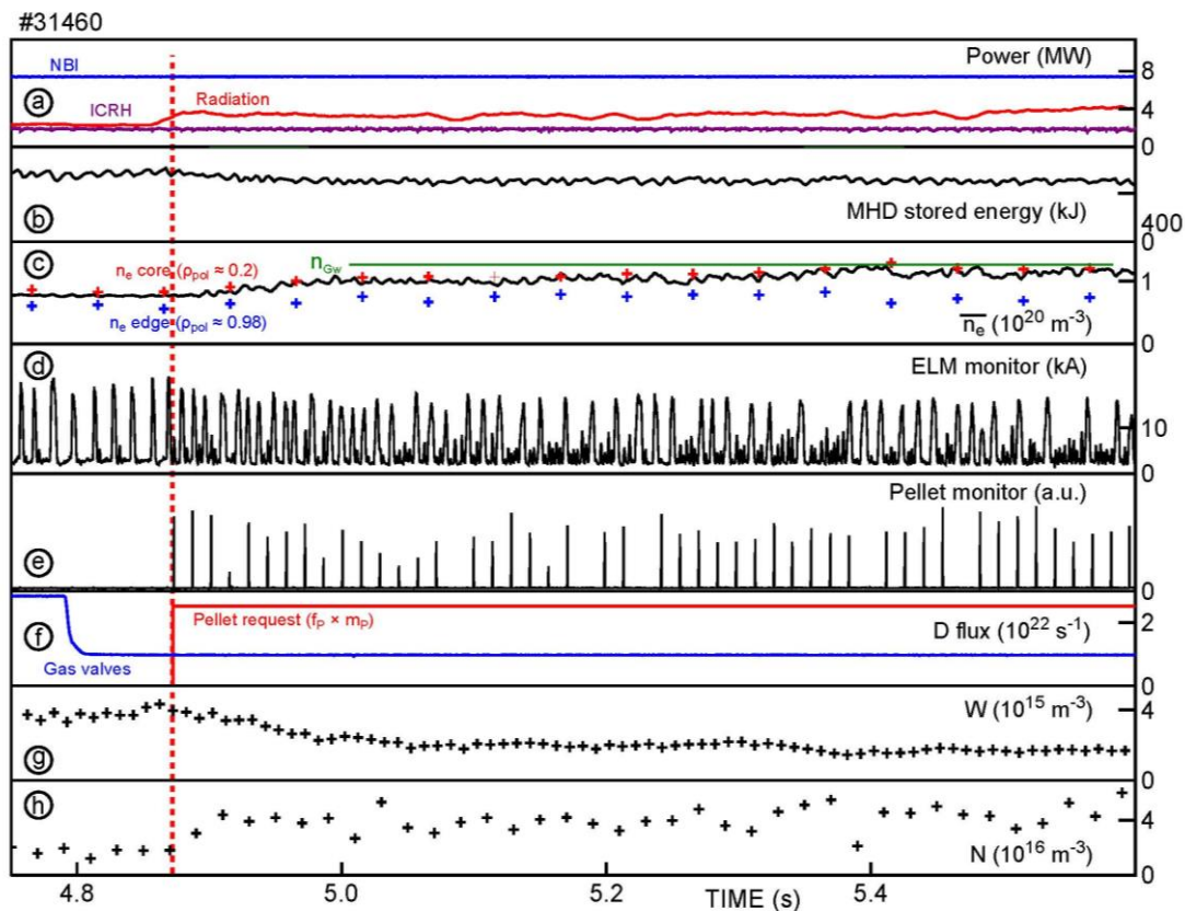
Figure 11: High density operation achieving a core density in the vicinity of n_{Gw} by pellet injection. Doping the D host pellets by N (0.8 % found in the released gas) yields an enhancement of the N concentration in the plasma while the impurity level, here represented by the W concentration, is reduced.
