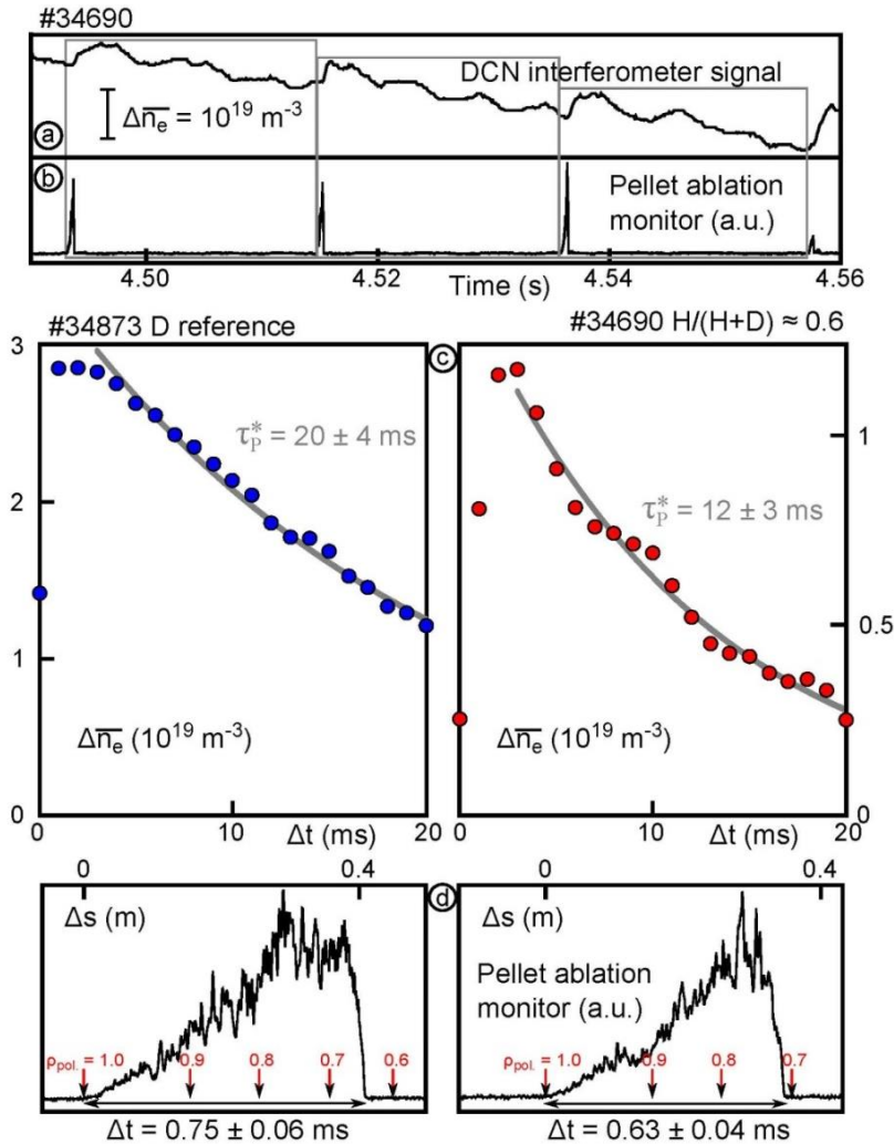
Figure 10: Determination of the pellet particle sustainment time \tau_p^* for a pure D (left) and a HD plasma (right) from the post pellet density decay averaging over 11 virtually identical pellet each (c). Data are taken from the DCN laser interferometer (a) eliminating fringe jump by taking advantage of the pellet ablation monitor as synchronization marker (b) and calibration to Thomson data. D pellets penetrate deeper into the plasma, as shown by typical ablation radiation measurements for single pellets (d).
