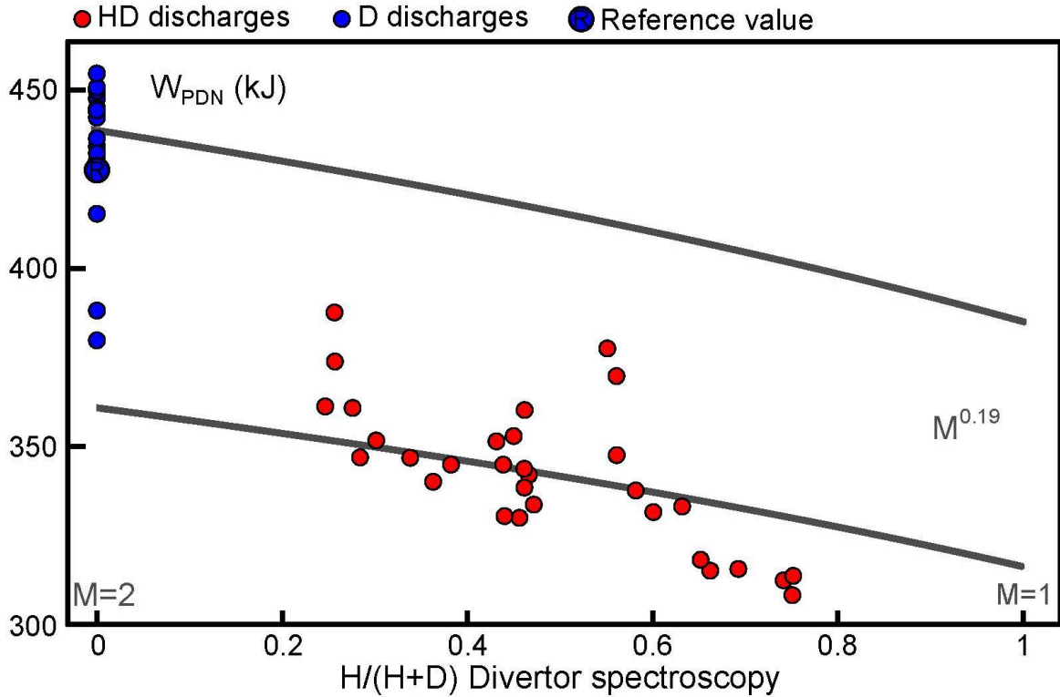
Figure 8: H/(H+D) from divertor spectroscopy versus plasma stored MHD energy normalized with respect to heating power and density dependence. Red dots: H/D pellet fuelled shots. Blue dots: data from reference shot with heating power below 9 MW and core density below n_{Gw} . When attributing D references to M=2 and pure H operation to M=1 , it turns out the observed behaviour near H/(H+D) = 0 does not fit well with a simple isotope fraction exponent a_M for some a_M , e.g. 0 < a_M < 1.0 .
