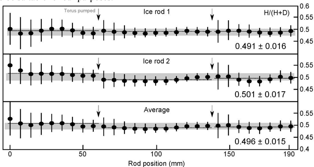
Figure 1: Analysis of the H/(H+D) composition of two ice rods produced from an initially 1:1 H 2 /D 2 gas mixture. Consecutive sequences of 3 pellets were launched into the torus, after each sequence the residual gas was analysed. After several sequences, the torus had to be re-evacuated, thus 3 rod sections are analysed separately. Dashed lines represent the average isotope composition of the three sections.
