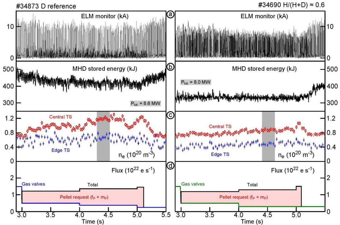
Figure 9: Comparison of the fuelling impact of the pellets in the pure D reference discharge (left) and the discharge with a H/(H+D) fraction of about 0.6 (due to divertor spectroscopy). In both cases, the initiated particle fuelling is almost identical; also the heating power is nearly the same. Obviously, the density increase is much reduced in the presence of H – indicating for a reduction of the particle confinement time. For both cases phases stable with respect to the density evolution are chosen for analysis of the pellet imposed density perturbations (indicated by the grey bars, sequences of pellets with virtually identical size on arrival without lost pellets).
