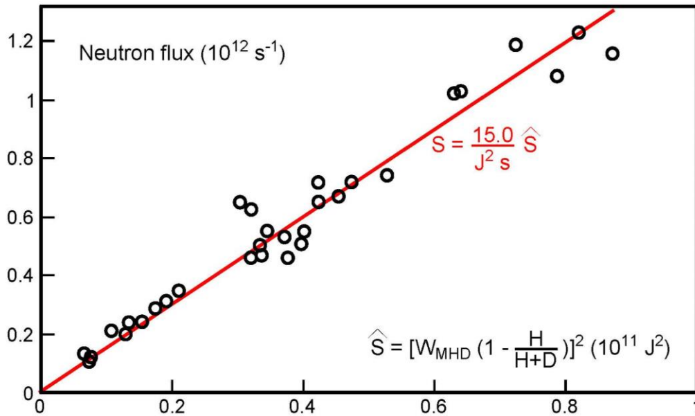
Figure 5: Correlation of the neutron flux with neutron rate as estimated by using the H/(H+D) fraction obtained by divertor spectroscopy measurements. Measured data (black circles) and fit (solid red line).
