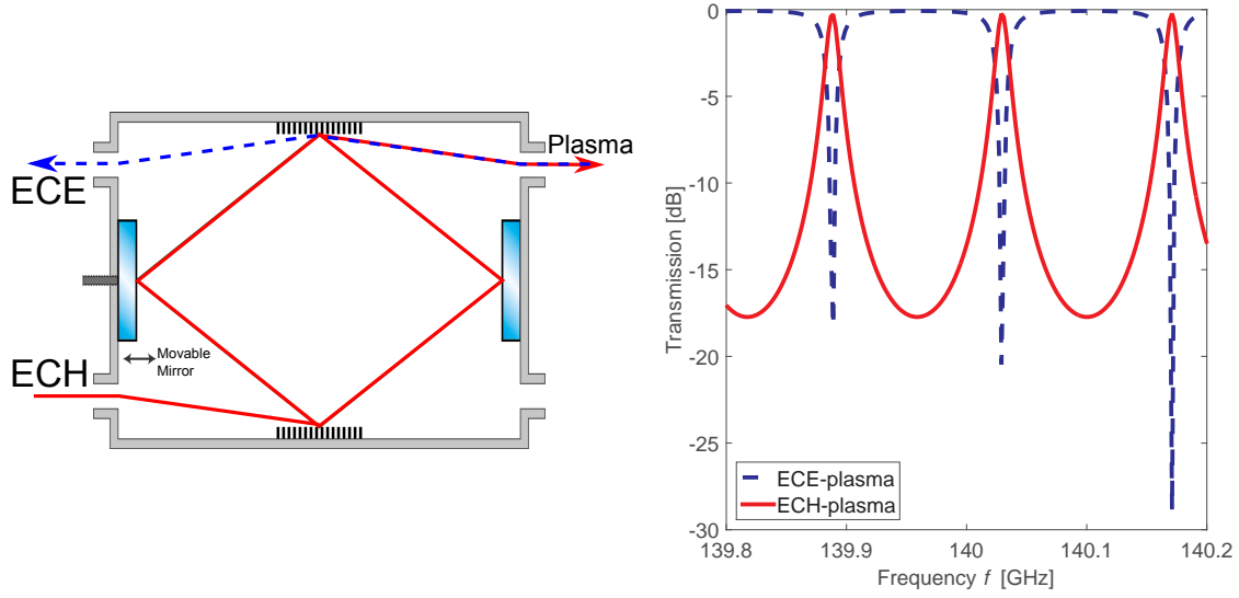
Figure 2. Schematic overview of the bi-directional FADIS set-up on the left [13], which shows two output ports on the plasma side (right) and two input ports (left), connected to the inline ECE radiometer and an ECH source. The paths traveled by ECH and ECE are indicated in red and blue, respectively. Grated mirrors are visible at the top and bottom of FADIS. Two resonator mirrors are shown at the left and right. The left mirror is used to adjust the resonance frequency. The transmission as a function of frequency is shown on the right, for the paths traveled by ECH and ECE in red and blue, respectively, which are the resonant and non-resonant ports for the port labeled plasma. Note that the transmission can be varied by changing either the frequency or the position of the FADIS movable mirror. Residual ECH power, which is not transmitted via the resonant port to the plasma, is dumped into a load connected to the open port (not shown).
