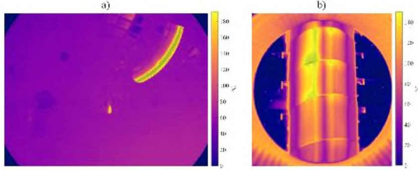
FIG. 3 a) LWIR camera system view b) MWIR camera system view.
