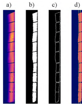
FIG. 12 Image obtained by projecting the left strike-line in the 2D grid, and the process to estimate its horizontal position and width.
