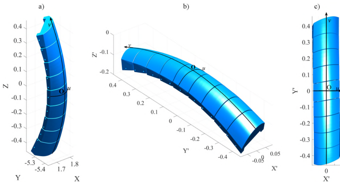
FIG. 7 Module 5 limiter and reference curvilinear axes: a) full view in original coordinate system, b) full view in transformed coordinate system, c) front view obtained through a projection on the X'Y' plane
