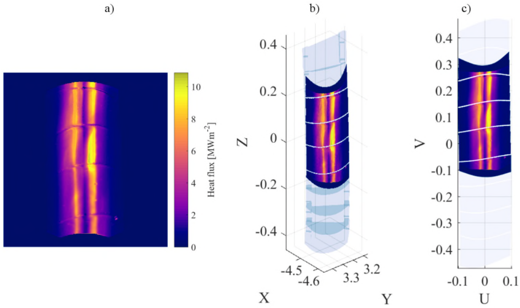
FIG. 10 MWIR camera a) heat flux image for module 3 limiter b) projection onto the XYZ reference system c) projection onto the 2D coordinate system.
