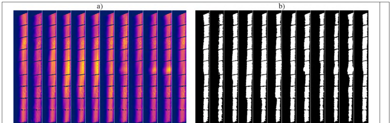
FIG. 11 Left strike-line images a) projected in the 2D grid for the 12 experiments and b) segmented.
