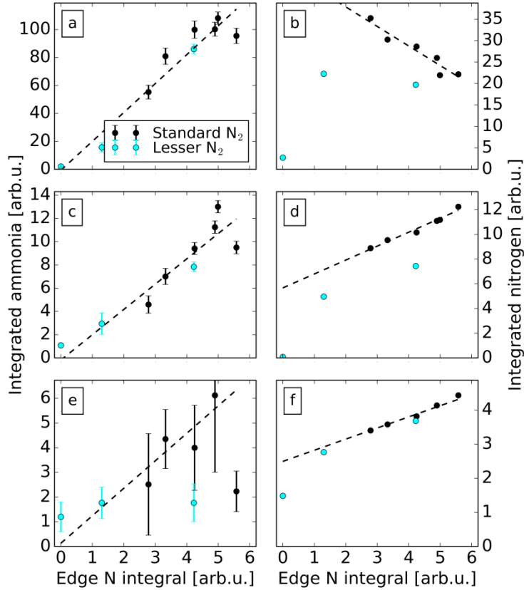
Figure 12: Pulse-integrated partial pressures of ammonia (a, c, e) and nitrogen (b, d, f) in the inner (a, b) and outer (c, d) divertor and the midplane (e, f), shown against pulse-integrated edge nitrogen density from CXRS, from discharges #33027 through #33038
