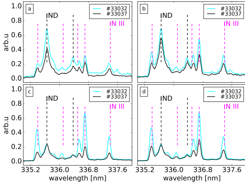
Figure 16: Spectra in the outer divertor, recorded in the flat-top of the seeded phases of discharges 33032 and 33037, in LOSs WOC001 (a), WOC002 (b), WOC004 (c) and WOC006 (d)
