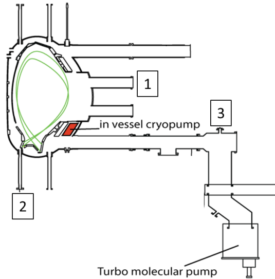
Figure 2: Neutral gas analysis setup at ASDEX-Upgrade. RGAs are located at the midplane (1), in the inner (2) and the outer (3) divertor.
