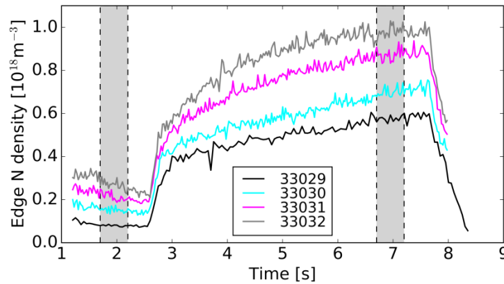
Figure 9: Time traces of the nitrogen density at the plasma edge from charge exchange recombination spectroscopy. Grey bars indicate the intervals representing the reference and the seeded phases.
