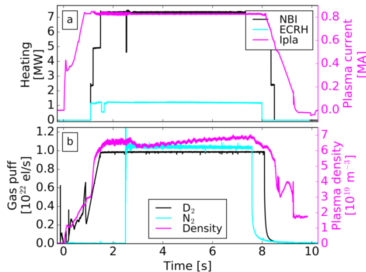
Figure 1: Discharge setup shown by time traces from discharge #33032, a) auxiliary heating and plasma current, and b) D 2 and N 2 injection rate
