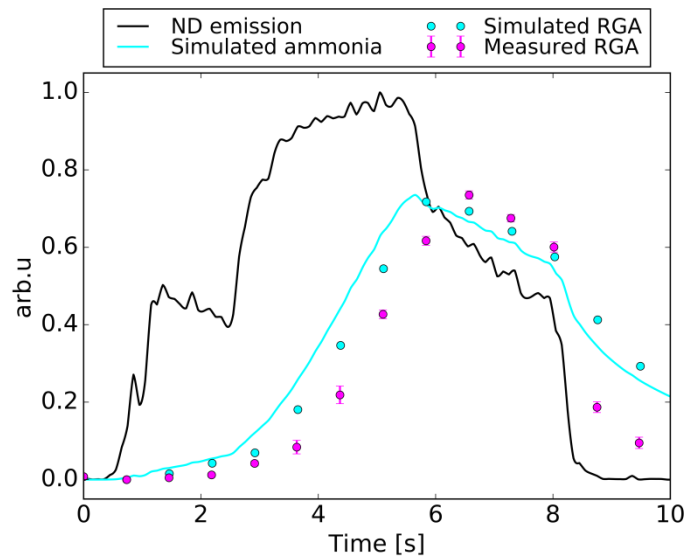
Figure 5: Simulated and recorded pressure of ammonia in the differentially pumped chamber of the inner divertor mass spectrometer in discharge #33038. The ND emission trend represents the flow of ammonia into the chamber. The simulated pressure of ammonia is additionally delayed by taking into account the limited time resolution of the mass spectrometer.
