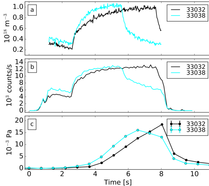
Figure 17: Time traces of the the core nitrogen density from CXRS (a), ND emission intensity in the RIV006 divertor spectroscopy line of sight (b) and partial pressures of ammonia in the inner divertor (c) from discharges #33032 and #33038
