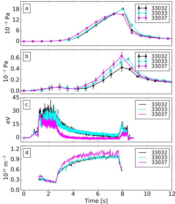
Figure 15: Time traces from discharges #33032, #33033 and #33037. a: partial pressure of ammonia in the inner divertor, b: partial pressure of ammonia in the outer divertor, c: outer divertor electron temperature, d: core nitrogen density from CERS, e: edge nitrogen density from CXRS
