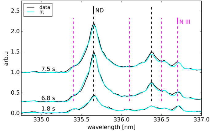
Figure 8: Spectra from various phases of discharge #33032 seen in the LOS RIV006, and the fitted model. The fitted temperatures are listed in Table 2.
