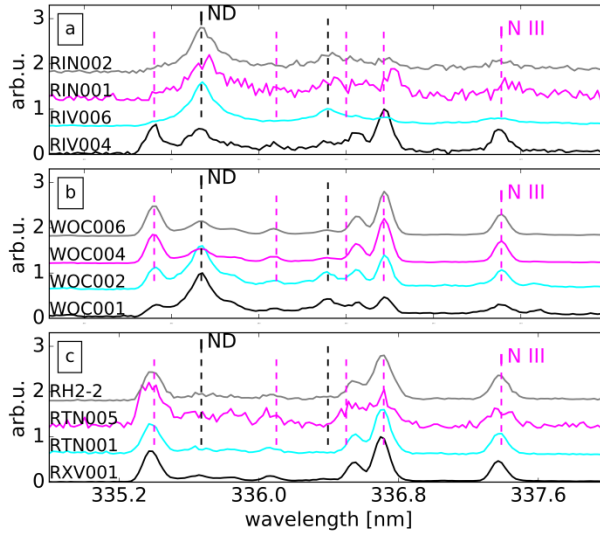
Figure 7: Normalized spectra in the inner (a) and outer (b) divertor region, and near the x-point (c), from t = 6.8 s in discharge #33032
