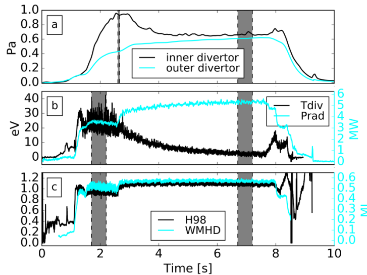
Figure 13: Time traces of absolute pressure in the divertor (a), outer divertor electron temperature and total radiated power (b), and normalized confinement and stored plasma energy (c), from discharge #33032. The grey stripes indicate the reference and seeded phase intervals, relevant for Fig. 10. The absolute pressure values are extrapolated from the direct measurements based on the respective calibration coefficients.
