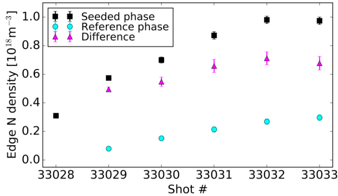
Figure 10: Average values of the edge nitrogen density from CXRS in the reference and the seeded phase of discharges #33028 (shot #1) through #33033 (shot #6), and the difference between them.
