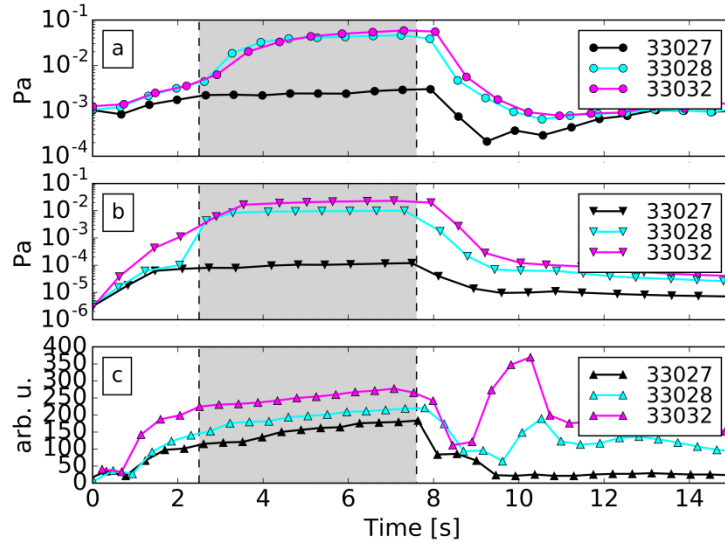
Figure 3: Partial pressures of N_2 in the inner (a) and outer (b) divertor, and in the midplane, for a non-seeded (33027), the first (33028) and the fifth and N_2 -seeded (33032) discharge in the series. The grey areas indicates the duration of N_2 -seeding in #33028 and #33032.
