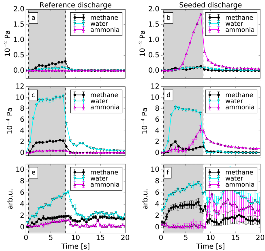
Figure 4: Identified partial pressures of water, methane and ammonia by RGA in the inner divertor (a, b), outer divertor (c, d) and in the midplane (e, f), in a non-seeded (a, c, e) and N 2 -seeded (b, d, f) discharge. The grey strips indicate the discharge phase.
