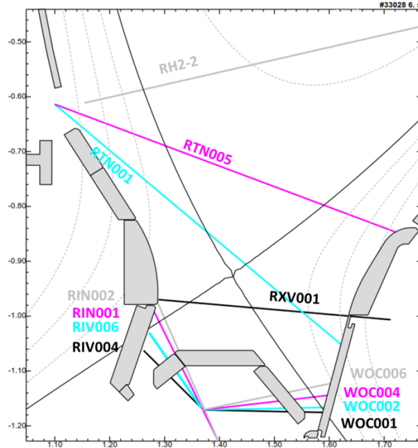
Figure 6: Divertor spectroscopy lines of sight
