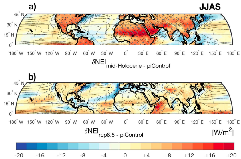
Figure 4. Net energy input (NEI) difference between (a) mid-Holocene and (b) rcp8.5 relative to piControl in June-to-September (JJAS) ensemble means (shading). Black dashed lines in each panel show the piControl as reference (contour interval 20 W/m 2 ). Stippling indicates areas where at least eight out of nine models agree on the sign of the change.
