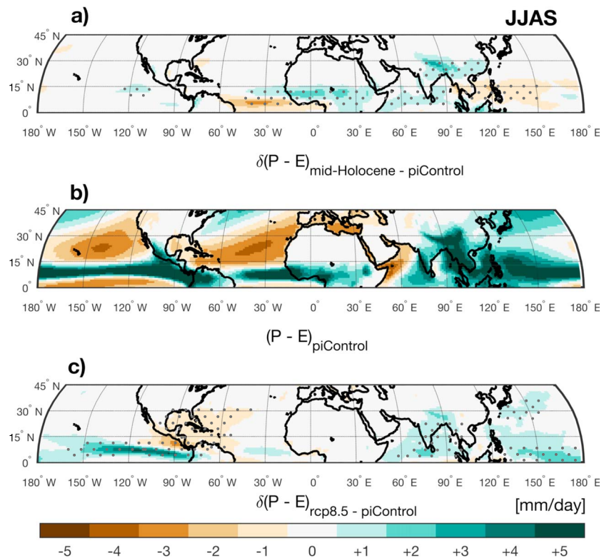
Figure 2. Net precipitation difference between the mid-Holocene (a) and the rcp8.5 (c) relative to piControl in June-to-September (JJAS) ensemble means (shading). PiControl is also shown as reference (b). Stippling indicates areas where at least where eight out of nine models agree on the sign of the change.
