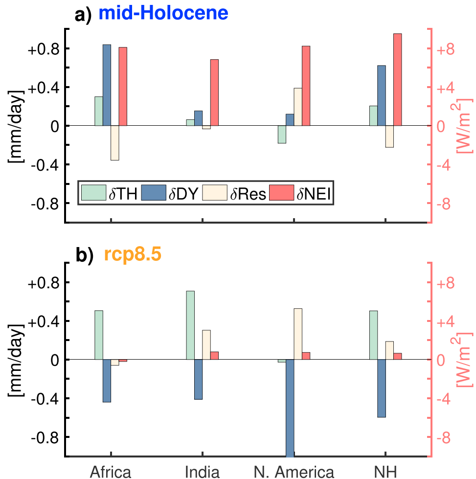
Figure 3. Regionally averaged net energy input (NEI—red axis) changes and changes in thermodynamic ( \delta TH ) and dynamic ( \delta DY ) components of the moisture budget, as well as its residual ( \delta Res ; see equation (1)) for (a) mid-Holocene and (b) rcp8.5 (black axis). Note that eight out of nine models agree on the sign of the change.
