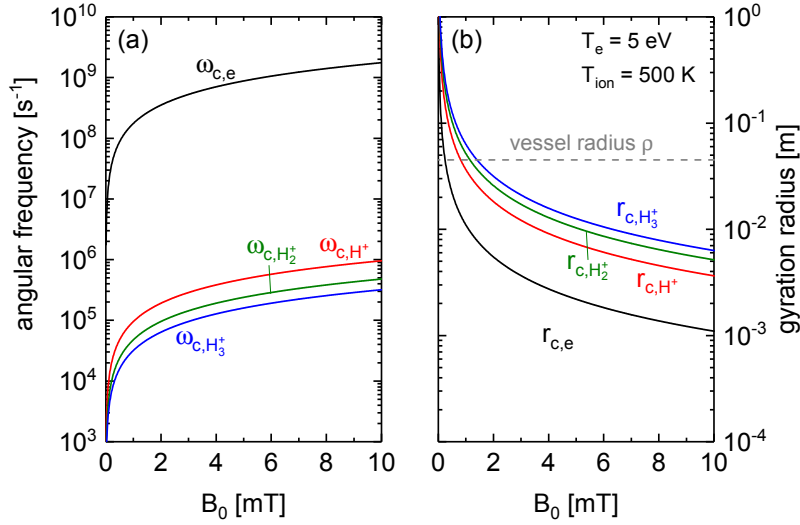
Figure 3.5: Gyration frequencies (a) and radii (b) of electrons and positive hydrogen ions H^+ , H_2^+ , H_3^+ at varying magnetic field. In (b), the radius of the cylindrical discharge vessel applied in this work is indicated for a comparison.
