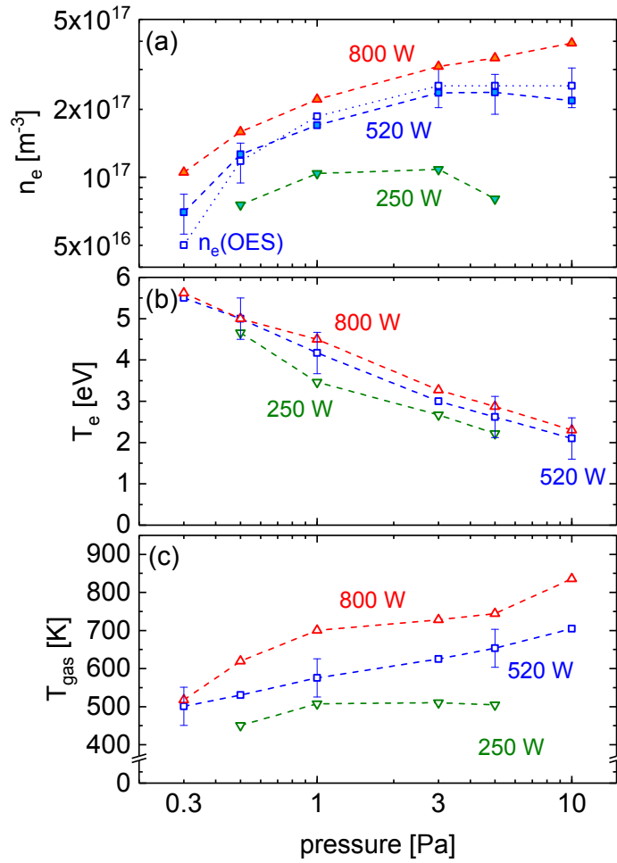
Figure 7.4: Plasma parameters of inductive hydrogen discharges driven at 1 MHz at varying pressure and RF power. Depicted in (a) is the electron density obtained by probe measurements (full symbols) and via optical emission spectroscopy and collisional radiative modelling (open symbols). In (b) the electron temperature is shown, evaluated by OES and CR modelling. (c) shows the gas temperature obtained via OES.
