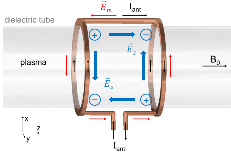
Figure 4.4: Scheme of the Nagoya type III antenna in operation at a fixed point in time. Indicated is the current flowing through the antenna (black), the induced electric field \mathbf{E}_m (red) and the space charges and electric fields generated due to the reaction of the plasma electrons (blue).
