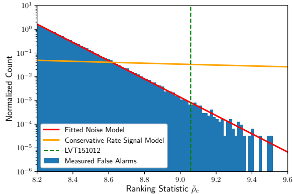
Figure 2. The scaled probability distributions of assumed signals and noise as a function of the ranking statistic \tilde{\rho}_c for the analysis containing LVT151012. Blue shows the normalized histogram of empirically measured false alarms that are within our selected BBH region of the template bank, P_N . Red is the exponential decay model that has been fitted to this set of false alarms, P_S \Lambda_S / \Lambda_N , normalized so that the counts can be directly compared to the noise distribution. Orange shows the signal model based on our conservative rate of detections. The value of \tilde{\rho}_c for LVT151012 is shown as a dotted green vertical line. The ratio of signal to noise at this value of \tilde{\rho}_c strongly favors the signal model.
