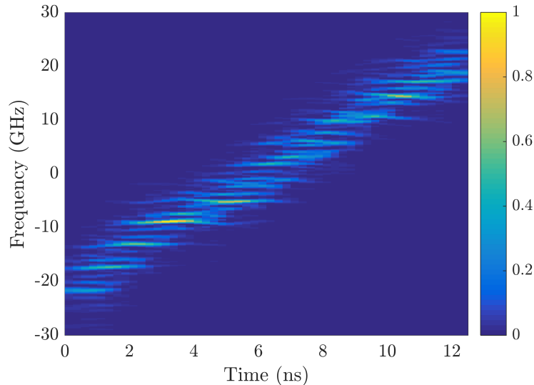
Fig. 4. Two dimensional optical spectrogram of the backward sweep. Intensity is indicated by the linear color-map.
