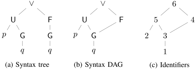
Fig. 1: Syntax tree, syntax DAG, and identifiers of the syntax DAG for the LTL formula (p \text{ U } G q) \vee (F G q)
