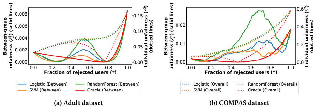
Figure 5: Between-group unfairness (solid lines— \mathcal{E}_\beta^2(b) in Eq. 5) and overall unfairness (dotted lines— \mathcal{E}^2(b) in Eq. 5) as a function of the decision ranking threshold ( \tau ) for various classifiers. Between-group unfairness \mathcal{E}_\beta^2(b) only constitutes a small fraction of the overall unfairness \mathcal{E}^2(b) .
