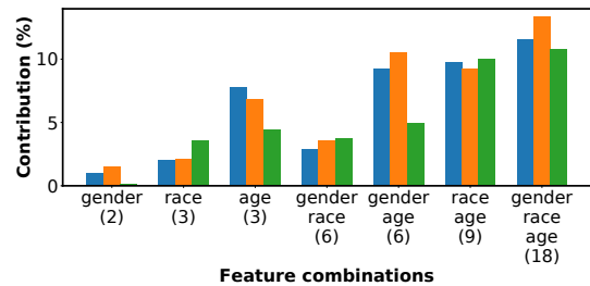
Figure 6: Between-group unfairness ( \mathcal{E}_\beta^2(b) in Eq. 5) as a fraction of the overall/individual unfairness ( \mathcal{E}^2(b) in Eq. 5) for various combinations of sensitive features. Numbers on the x-axis denote how many sensitive feature groups would be formed when using the corresponding sensitive feature set. Logistic regression, SVM and Random Forests achieve similar accuracies of 66%, 67% and 65% as well as similar overall individual unfairness of 0.145, 0.151 and 0.134 respectively on the ProPublica Compas dataset.
