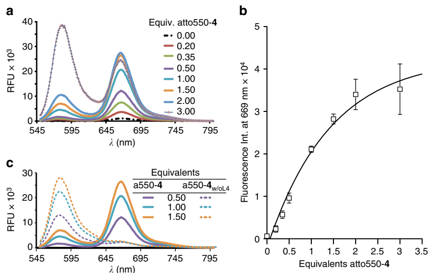
Fig. 4 FRET study of the formation of functional hybrid-nanoconstruct HyApNc. a Fluorescence emission spectra ( \lambda_{\text{ex}} = 535 \text{ nm} ) for FRET-assembled Atto647N-labeled trCLN3-L4 (Atto647N-3) and Atto550-labeled DxR-L4 motif (Atto550-4) HyApNc formation. Atto647N-3 was kept constant at 5 \mu\text{M} with increasing equivalents of Atto550-4. b Maximum fluorescence intensities at \lambda = 669 \text{ nm} ( I_{669} ) as a function of increasing concentration of Atto550-4 showing an increase in energy transfer ( n = 3 , error bars mean \pm S.D.). Saturation is reached between 2.0 and 2.5 equivalents of Atto550-4. c Comparison of the FRET signal ( \lambda_{\text{ex}} = 535 \text{ nm} ) of HyApNc consisting of 4 (straight) and 4 without the lipid tail (a550-4 w/oL4 ; dashed)
