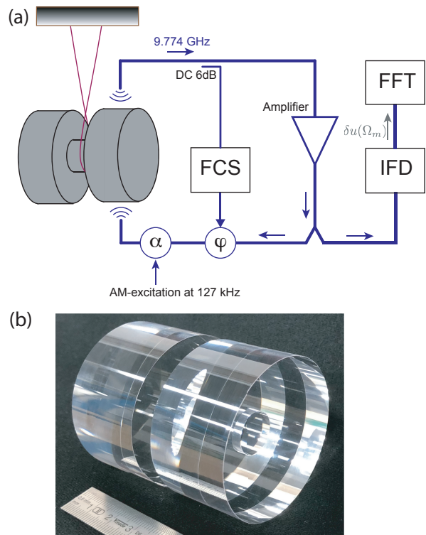
FIG. 1: (Color online) (a) Simplified schematic diagram of the experimental setup. Mechanical motion of the microwave sapphire loop oscillator. The FCS stands for the frequency control system which actuates the phase of the microwave signal by means of voltage-controlled phase shifter \varphi . The DC is the directional coupler. Approximately a half of the generated power is directed to the interferometric frequency discriminator (IFD), which converts frequency fluctuation of the microwave signal into synchronous fluctuations of the output voltage. The output signal \delta u(\Omega_m) is analyzed with FFT spectrum analyzer. For the excitation of the mechanical motion, the amplitude of the microwave oscillator is modulated at the mechanical resonance frequency by using voltage controlled attenuator \alpha . (b) Picture of the sapphire SB resonator. The ruler shows the scale of the system.
